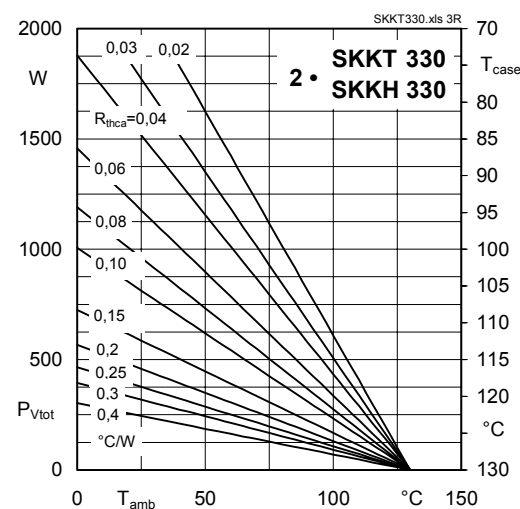
Fig. 3R Power dissipation of two modules vs. case temp.
