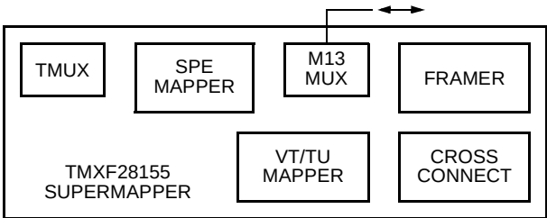
Figure 114. M13 Loopback Received DS3 Input to Transmit DS3 Output
