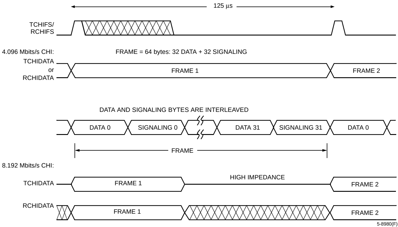
Figure 73. Associated Signaling Mode Concentration Highway Interface Timing
