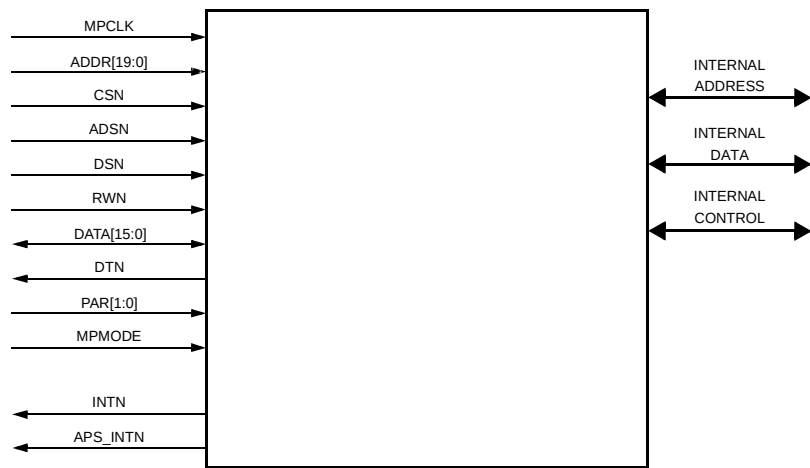
Figure 19. Microprocessor Interface
