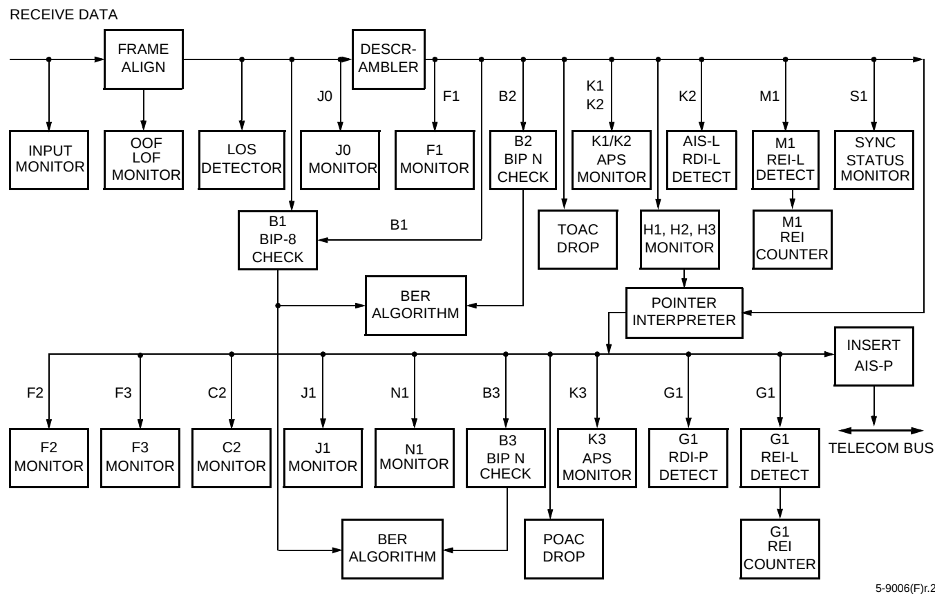
Figure 26. Receive Direction Functional Block Diagram
