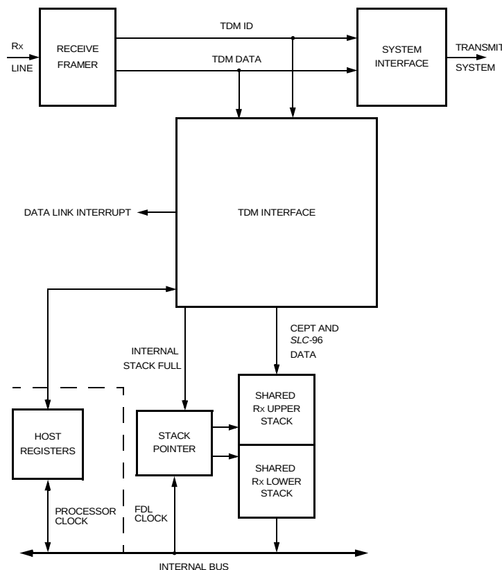
Figure 62. Rx Data Link Block Diagram
