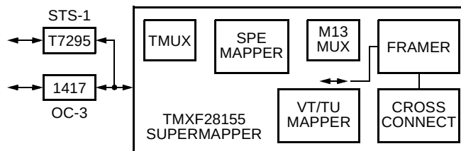
Figure 118. Loopback Line Source DS1 from Framer RP_T to Framer TP_R Through the Cross Connect
