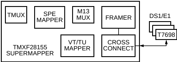
Figure 117. Loopback System Source DS1 from Framers TP_T to Framers RP_R Through the Cross Connect
