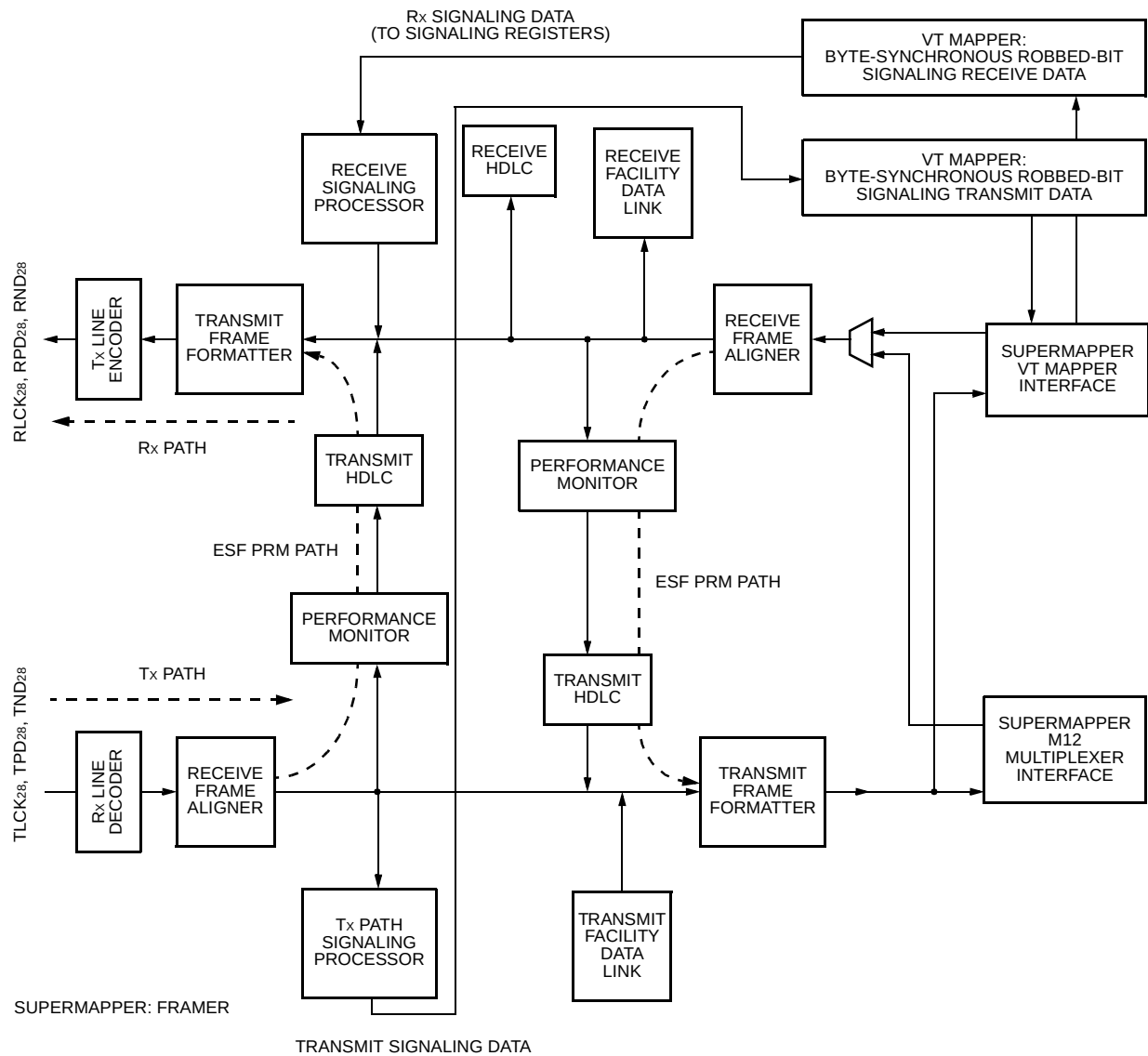
Figure 58. Supermapper Transport (with Intrusive Performance Monitoring) Mode
