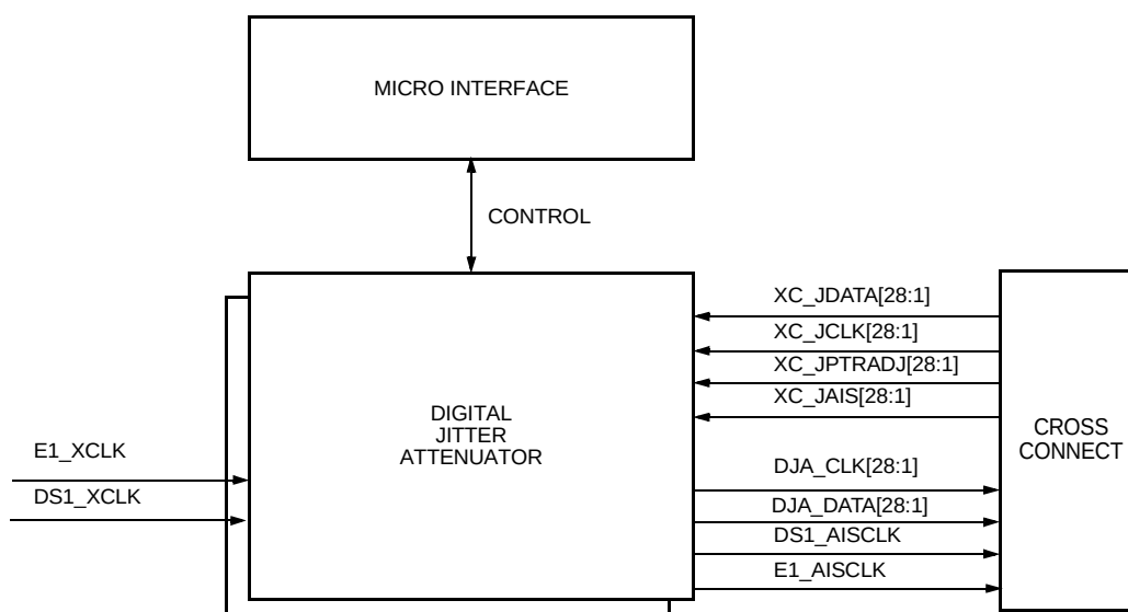
Figure 99. DJA Block with I/O Connections to Other Blocks in the Device
