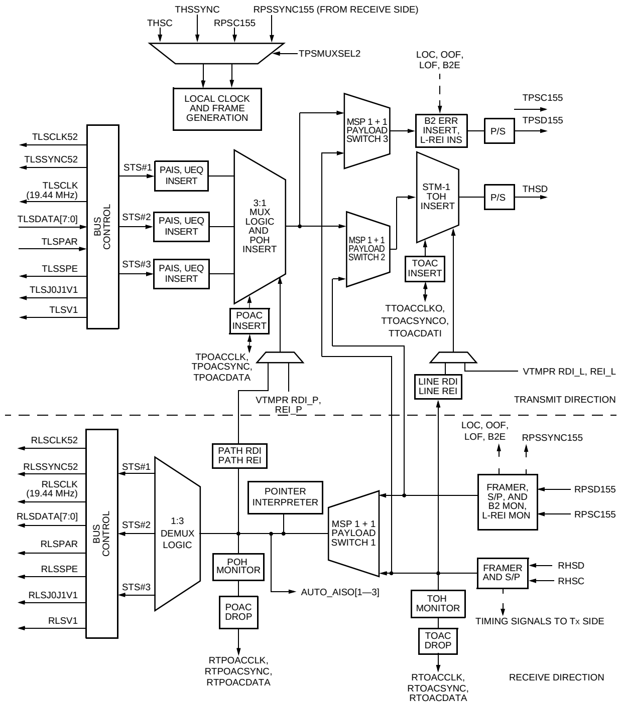
Figure 25. Detailed Block Diagram of the TMUX
