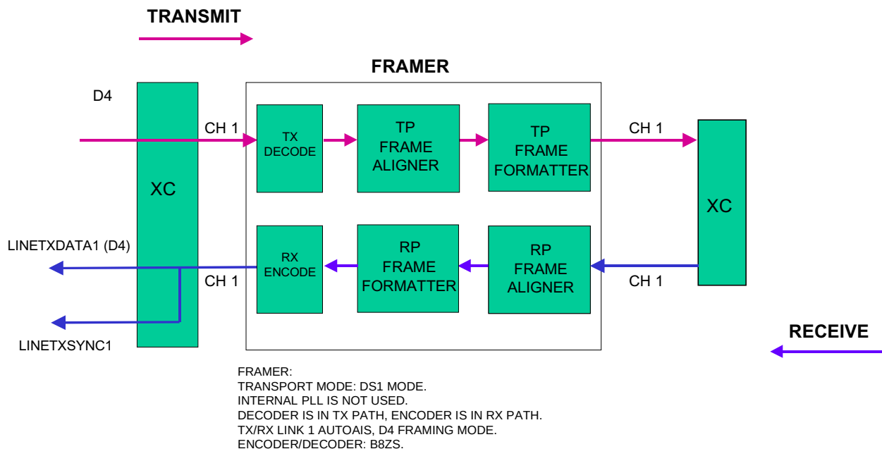
Figure 147. D4 INTENCDEC LINK1 FRAMER TRANSPORT Tx-Rx
