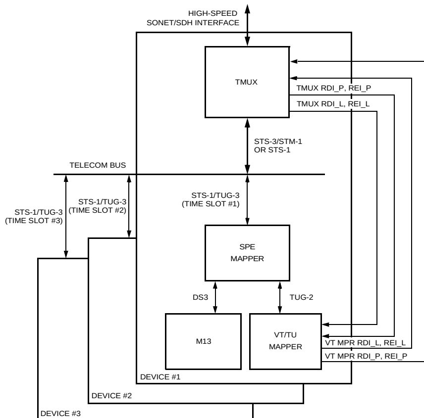
Figure 24. High-Level TMUX Interconnect
