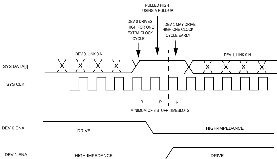
Figure 77. Parallel Bus System Interface Turnaround Timing
