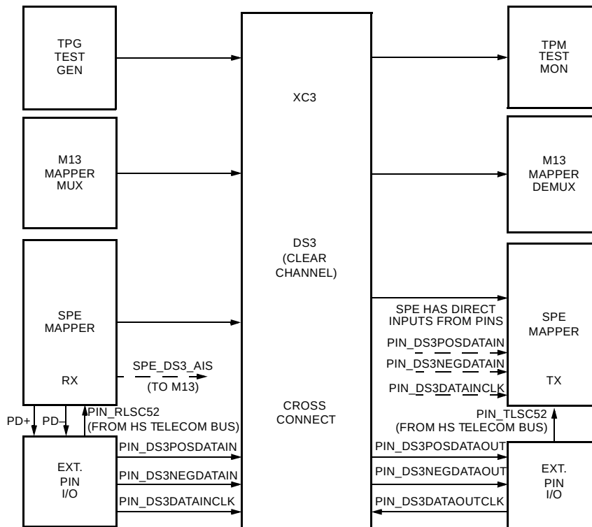
Figure 94. DS3 Cross Connect
