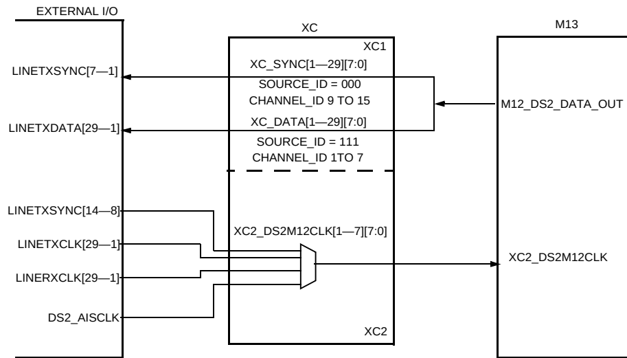
Figure 90. M12 MUX DS2 Output Cross Connect
