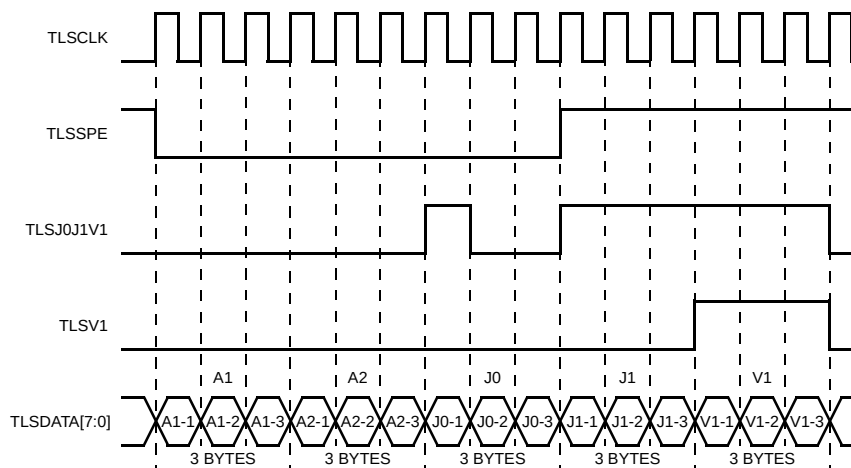
Figure 29. Transmit Low-Speed Bus Interface Signals for STS-3/STM-1 Signals
