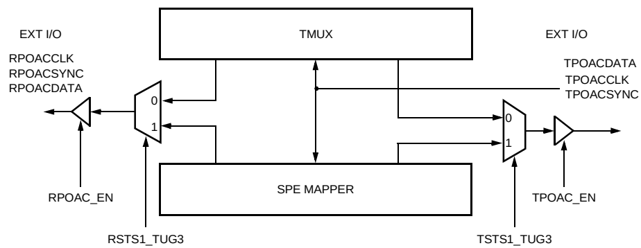
Figure 98. TPOAC and RPOAC Cross Connect
