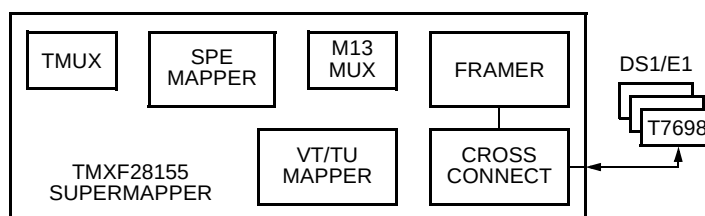
Figure 119. Internal Framer System Side TX → RX DS1 Loopback Without Cross Connect
