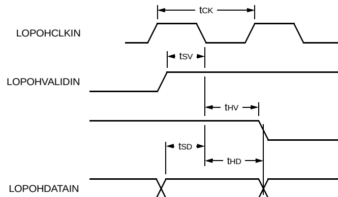
Figure 9. VT Mapper Transmit Path Overhead Detailed Timing
