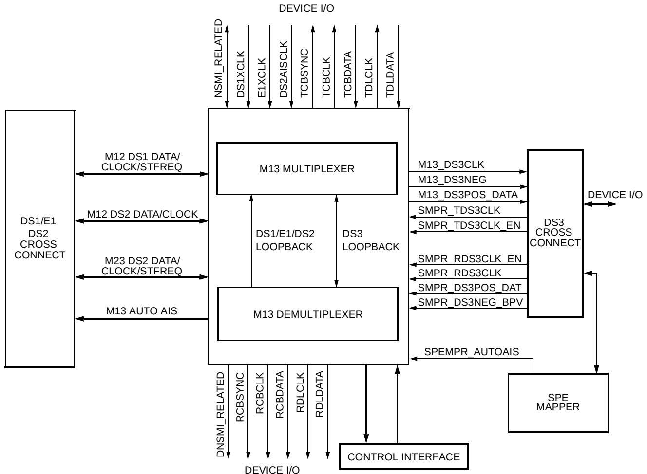
Figure 48. M13 Block Diagram
