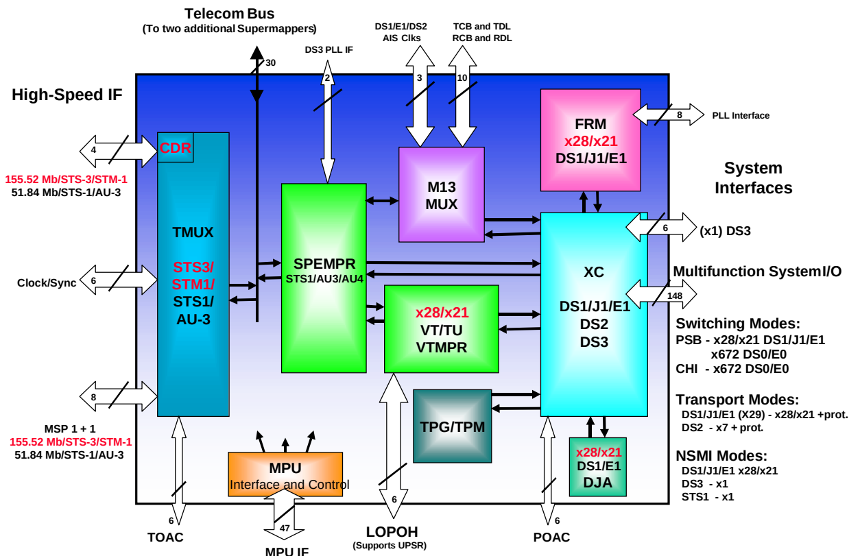
Figure 1. Functional Diagram of Supermapper
