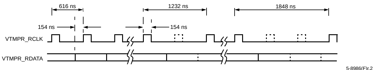
Figure 42. DS1 Mode Gapped Clocking Scheme
