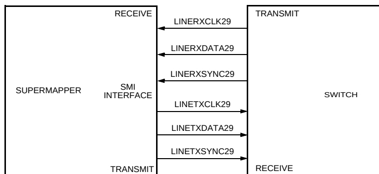
Figure 78. Signals (6-Pin Mode)
