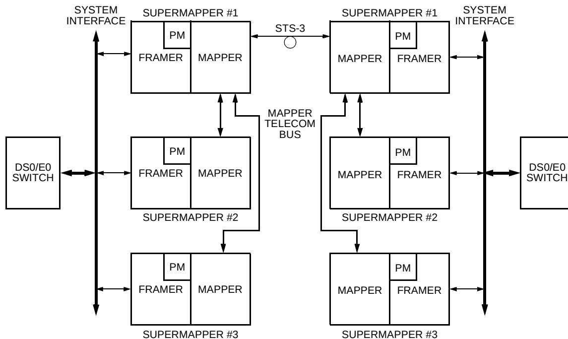
Figure 53. Switching Application of the Supermapper
