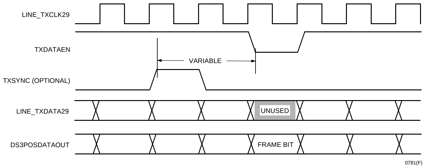
Figure 51. DS3 NSMI Transmit Operation
