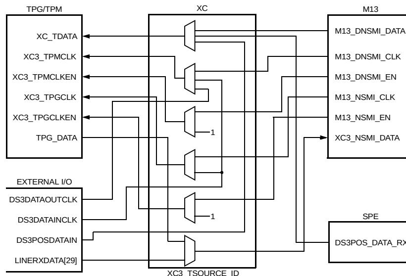
Figure 95. DS3 Test-Pattern Cross Connect
