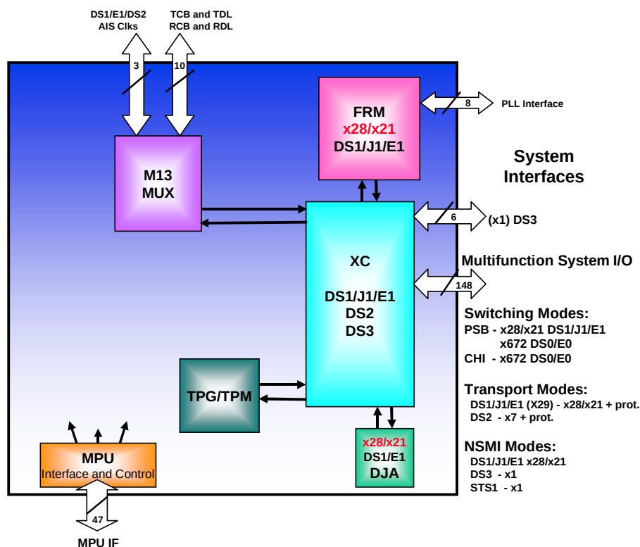
Figure 153. Superframer Block Diagram
