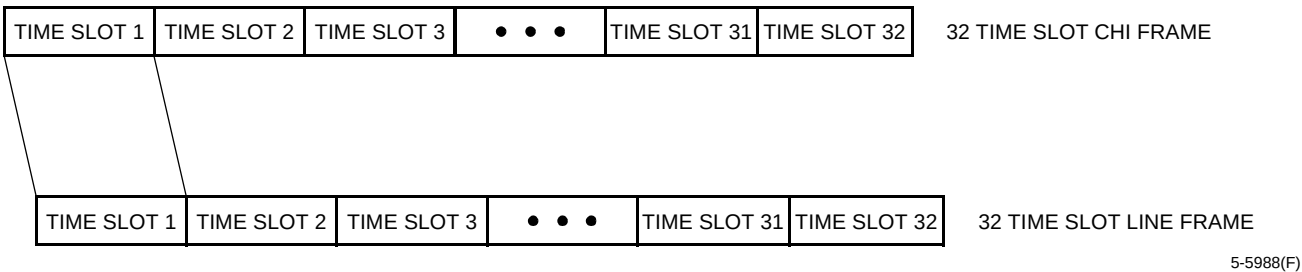
Figure 60. CEPT Transparent Frame Structure
