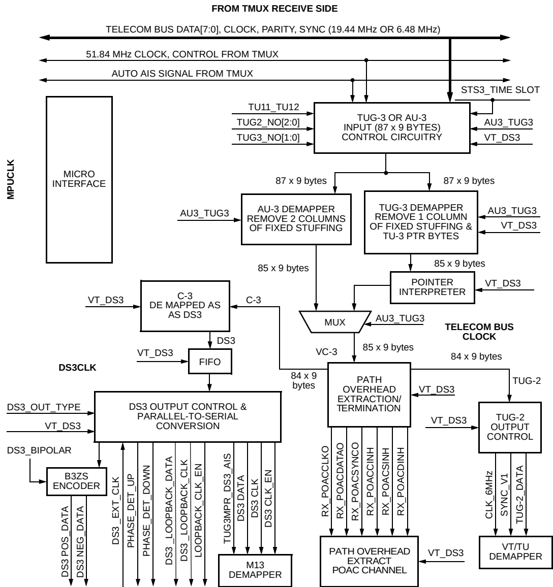
Figure 33. Basic Functional Flow of the SPE Mapper Receive Section
