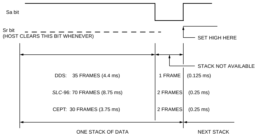
Figure 63. Stack Available and Stack Ready Bit Formatting
