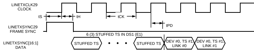
Figure 13. Parallel System Bus Interface Transmit I/O Timing
