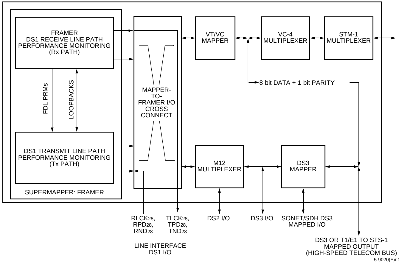
Figure 57. Supermapper Transport Configuration
