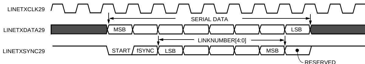
Figure 80. Network Serial Multiplexed Interface (Single Octet)
