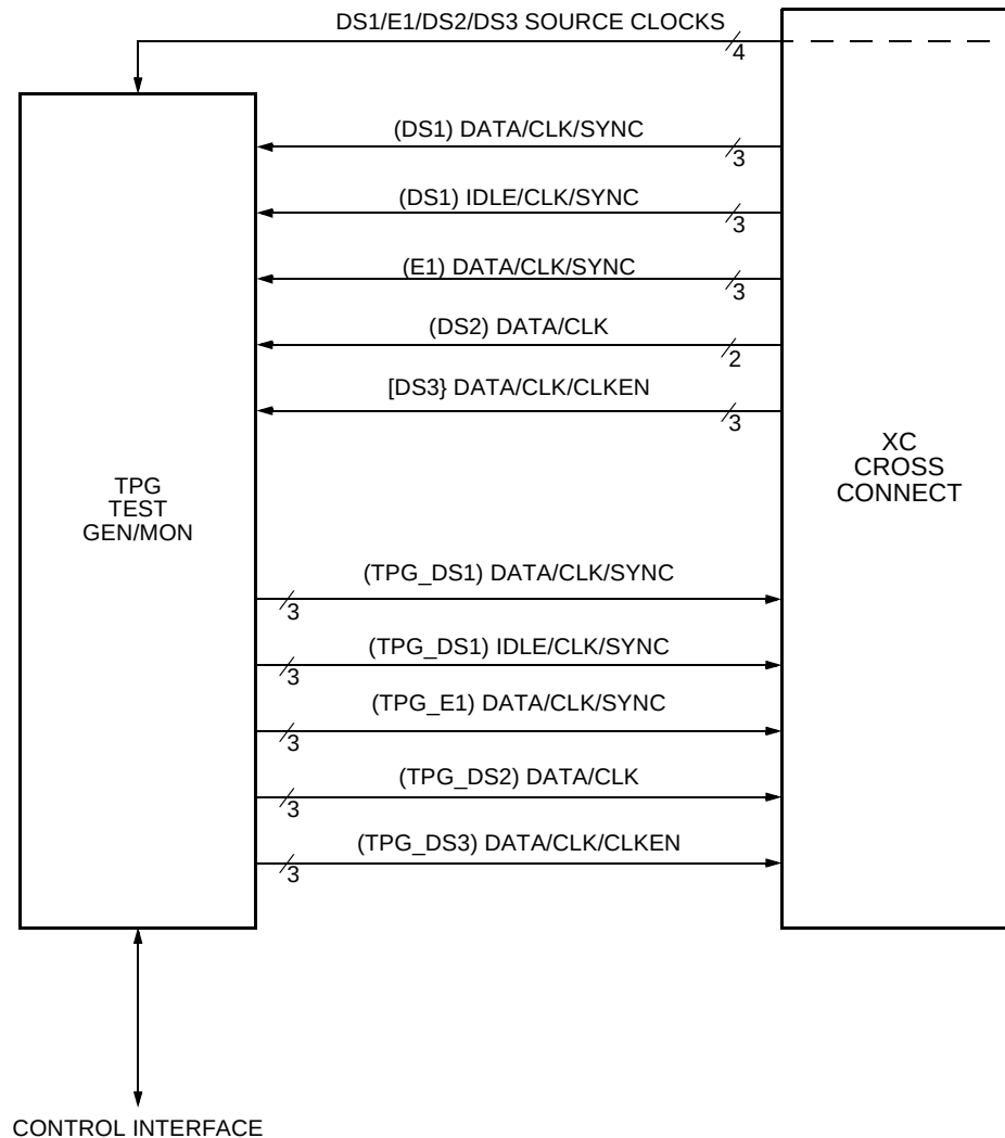
Figure 101. TPG Block Interface Block Diagram
