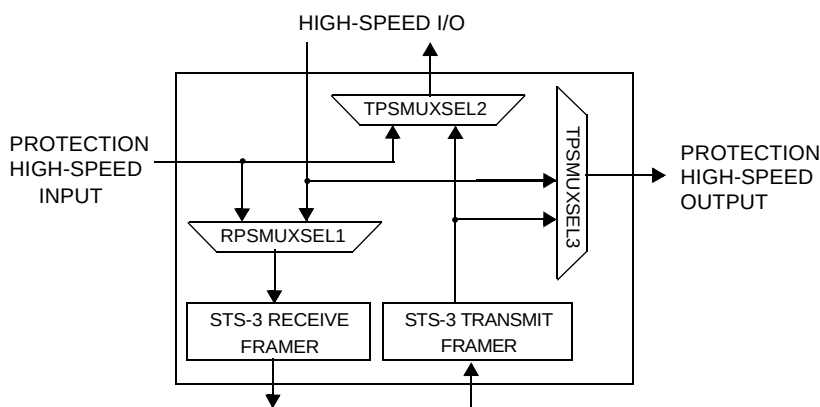
Figure 3. Protection Switch
