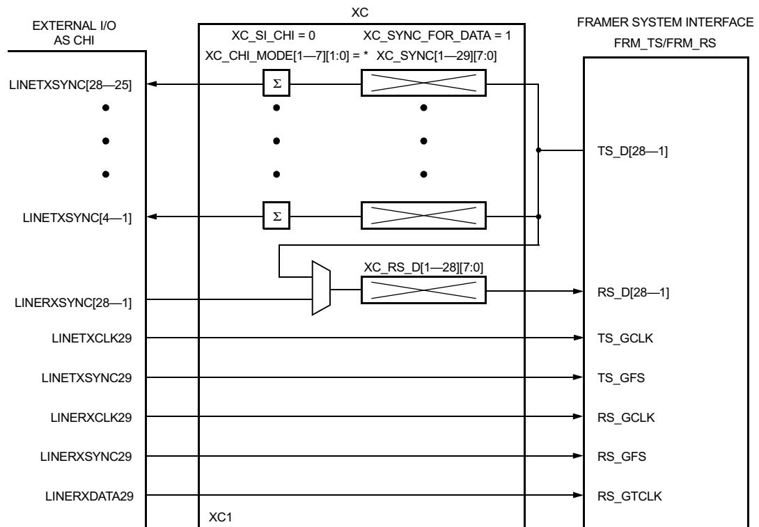
Figure 88. Framer System Interface—Concentration Highway Interface (CHI)
