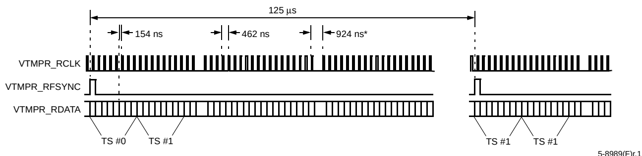
Figure 45. E1 Interface
