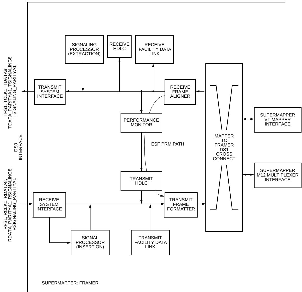
Figure 106. Supermapper Switching Mode for Framer in Parallel System Bus Configuration
