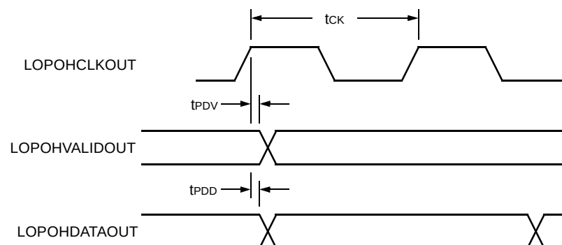
Figure 10. VT Mapper Receive Path Overhead Detailed Timing
