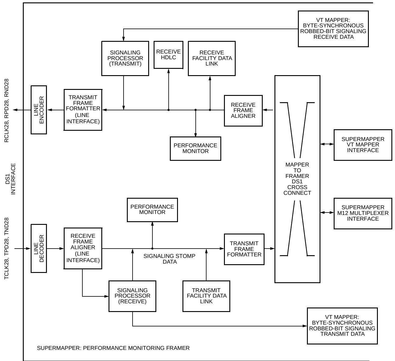
Figure 108. Supermapper Byte-Synchronous Transport Mode: Passive Performance Monitoring
