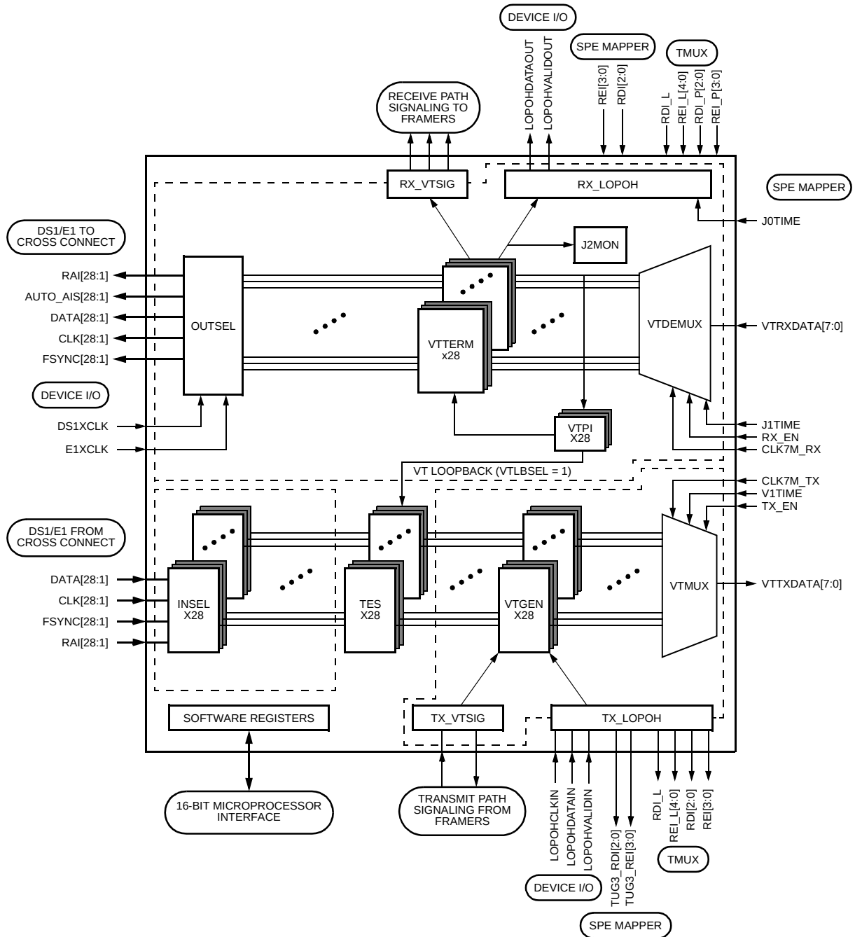
Figure 40. VT Mapper Functional Block Diagram
