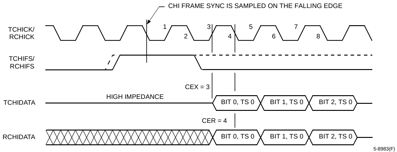
Figure 74. TCHIDATA and RCHIDATA to CHICK Relationship with FRM_CMS = 0
