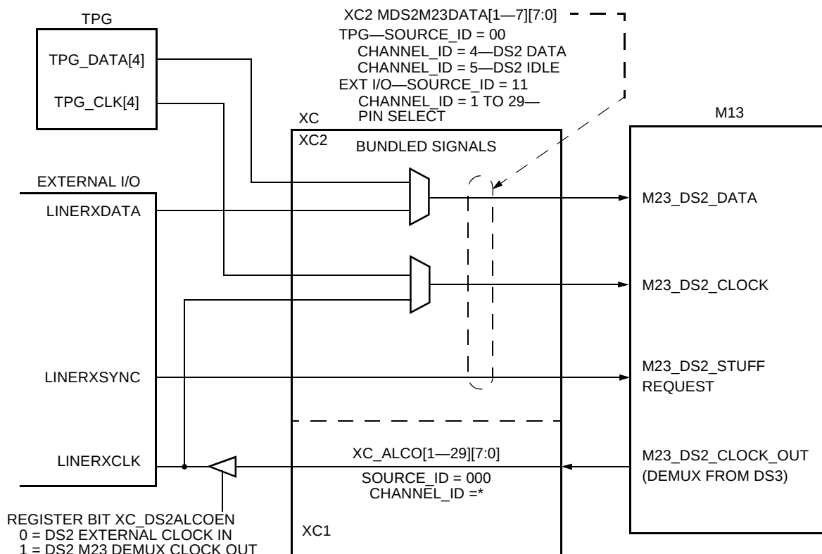
Figure 92. M23 DeMUX DS2 Output Cross Connect
