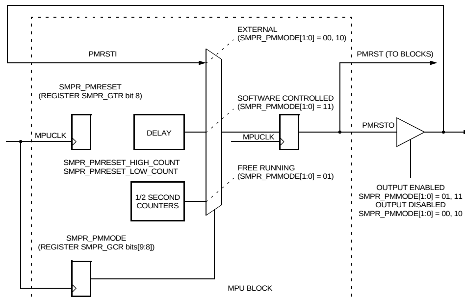
Figure 21. PM Reset Signal Generation
