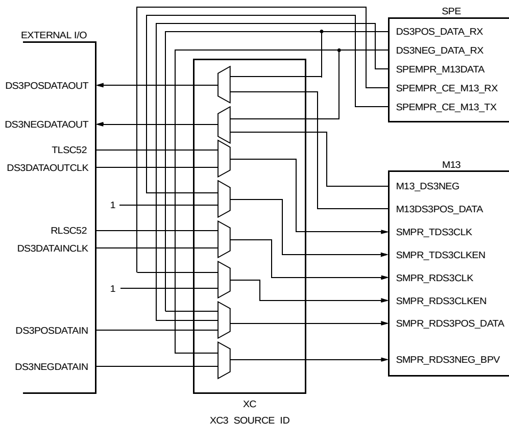
Figure 96. DS3 Basic Cross Connect
