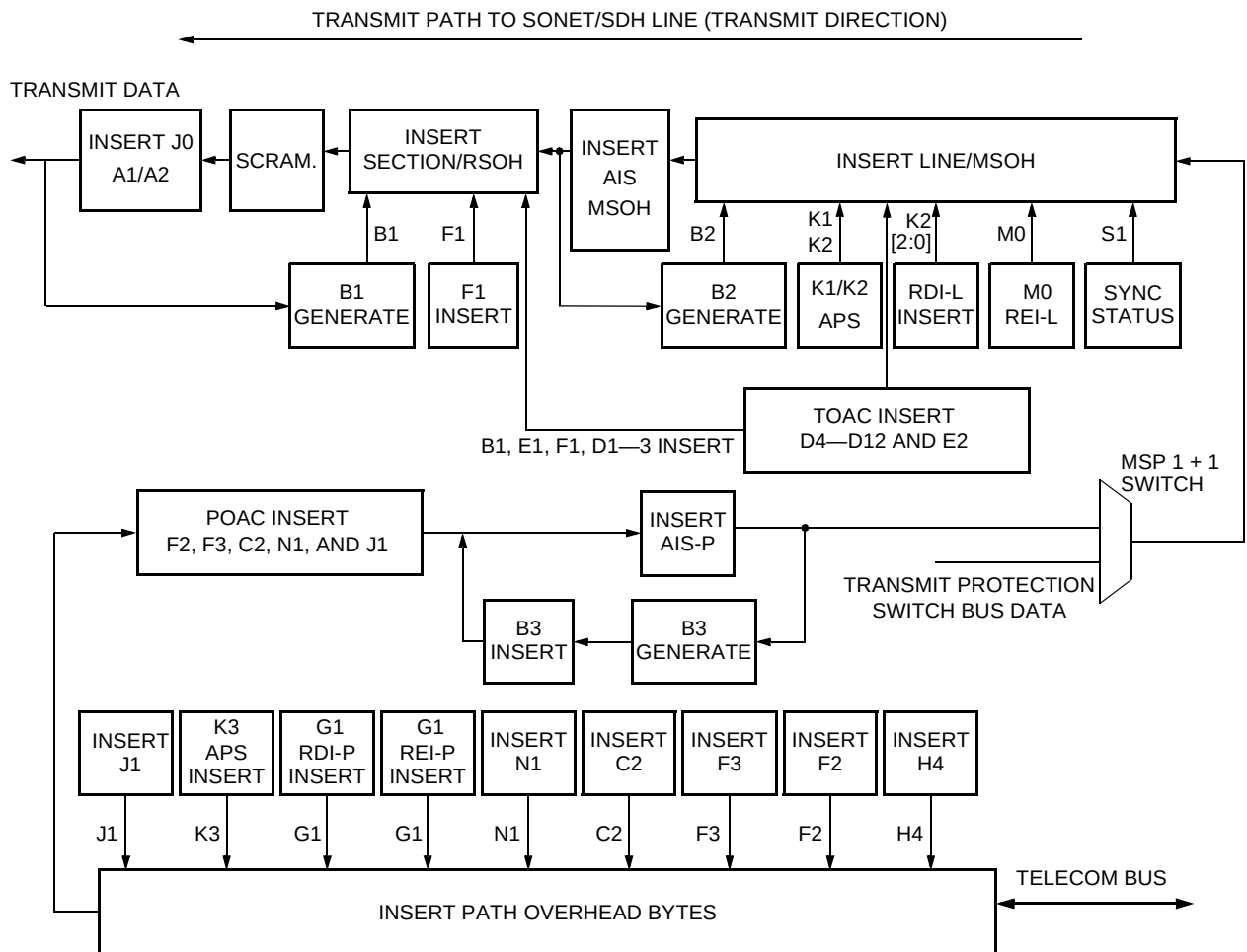
Figure 30. Transmit Direction POH and TOH Insertion Diagram
