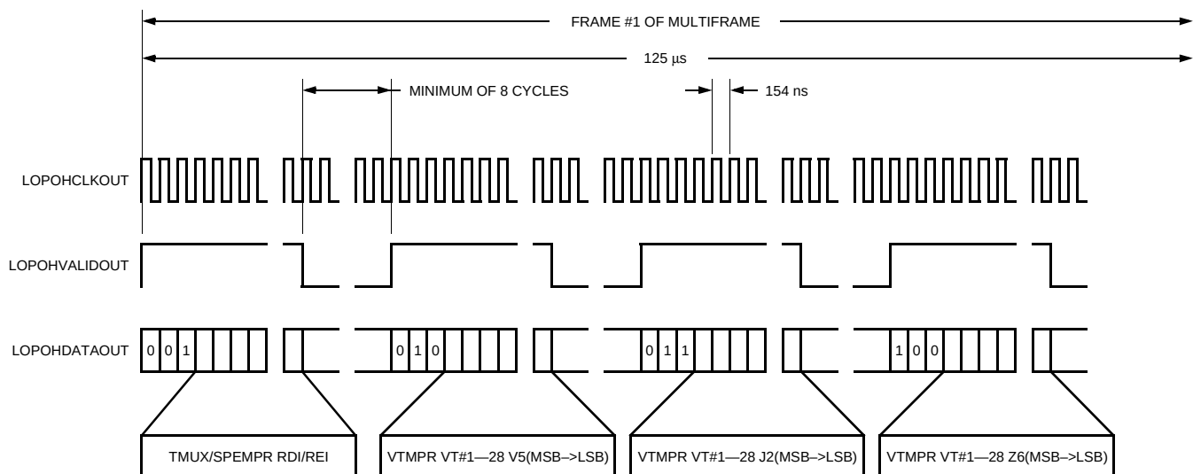
Figure 46. VT Mapper Receive Path Overhead Serial Access Channel
