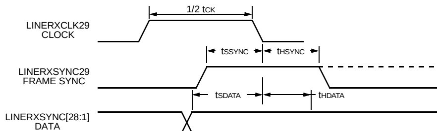
Figure 12. CHI Receive I/O Timing
