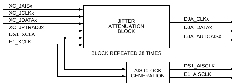
Figure 100. Basic Functional Flow of the DJA Block
