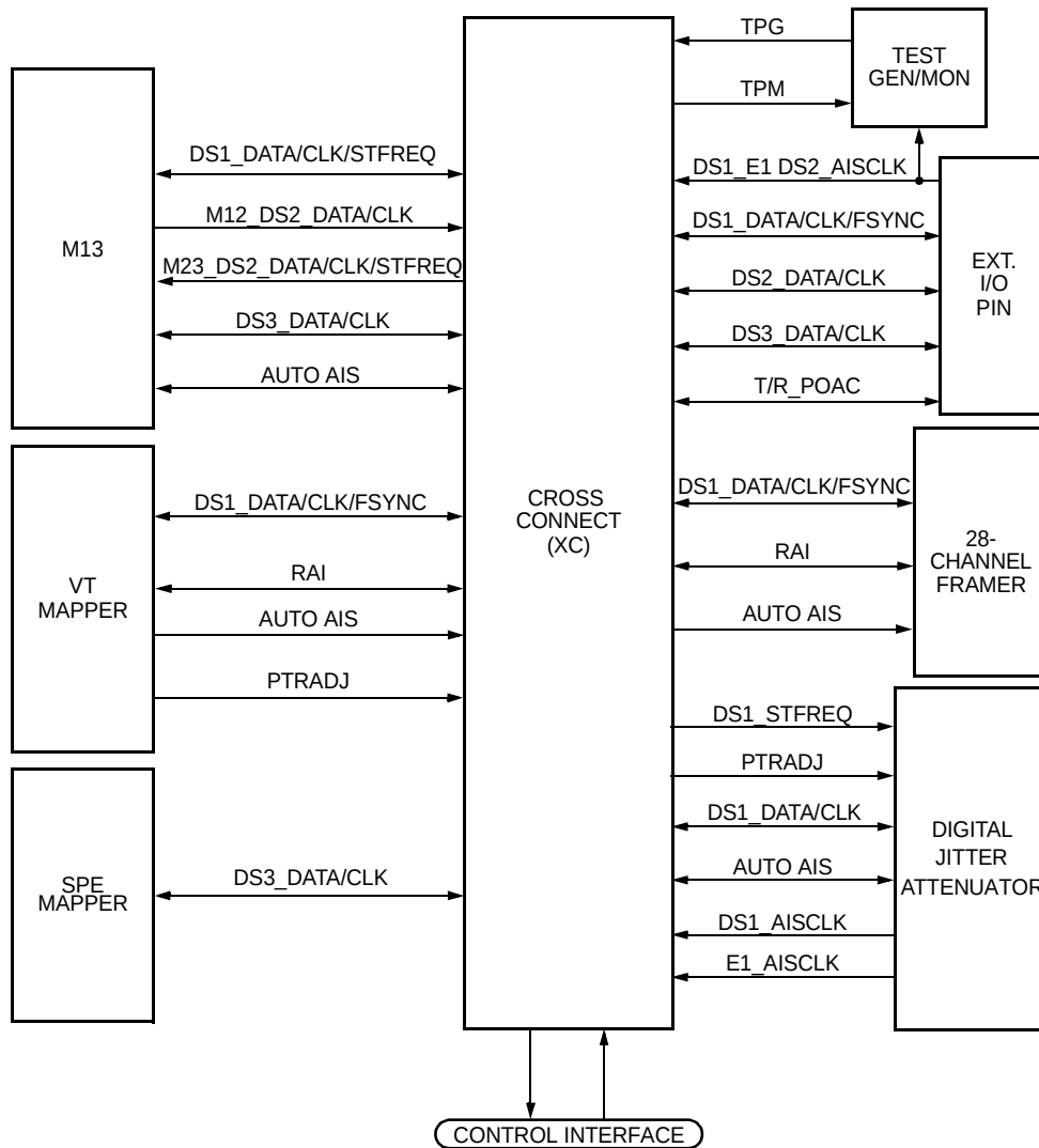
Figure 82. Cross Connect Block Diagram
