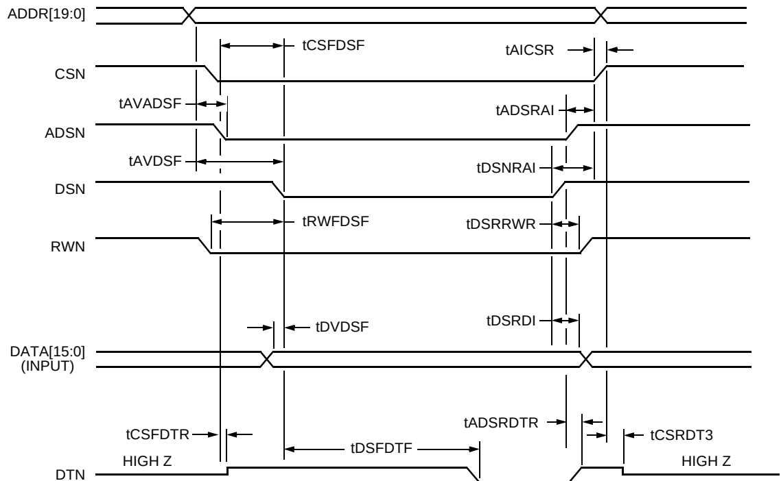
Figure 17. Microprocessor Interface Asynchronous Write Cycle Description (MPMODE (Pin AC18) = 0)
