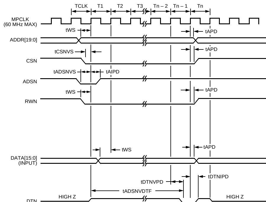
Figure 15. Microprocessor Interface Synchronous Write Cycle (MPMODE (Pin AD17) = 1)
