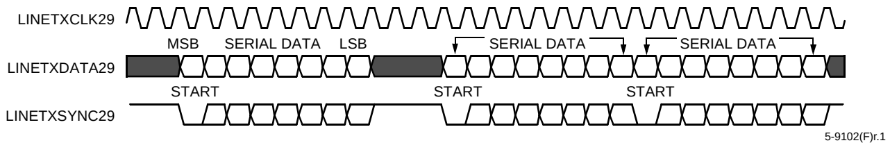
Figure 81. Network Serial Multiplexed Interface (Multiple Octets)
