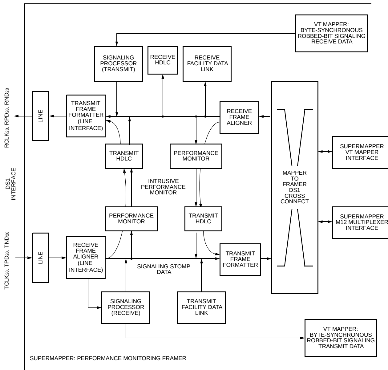
Figure 109. Supermapper Byte-Synchronous Transport Mode: Intrusive Performance Monitoring
