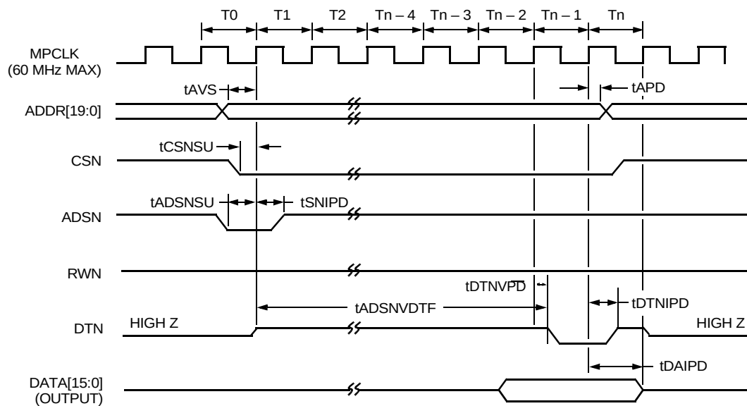
Figure 16. Microprocessor Interface Synchronous Read Cycle (MPMODE (Pin AD17) = 1)
