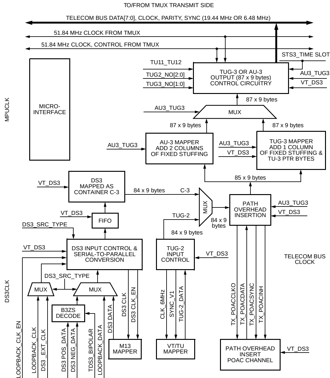
Figure 32. Basic Functional Flow of the SPE Mapper Transmit Section
