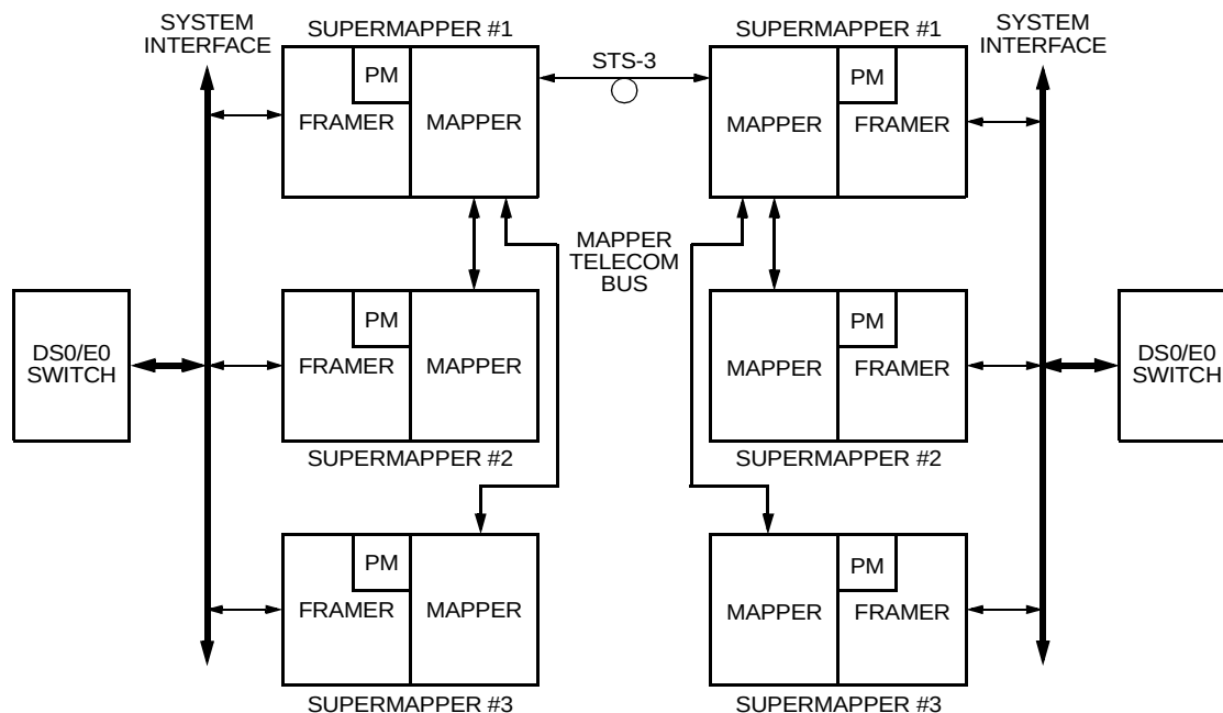
Figure 103. Switching Application of the Supermapper
