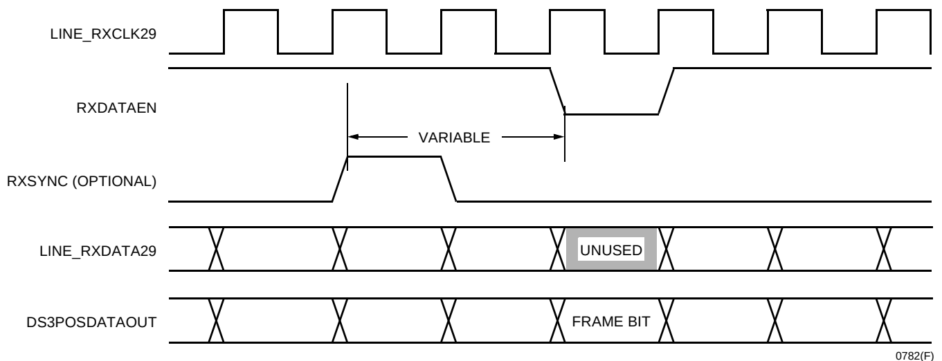
Figure 52. DS3 NSMI Receive Operation
