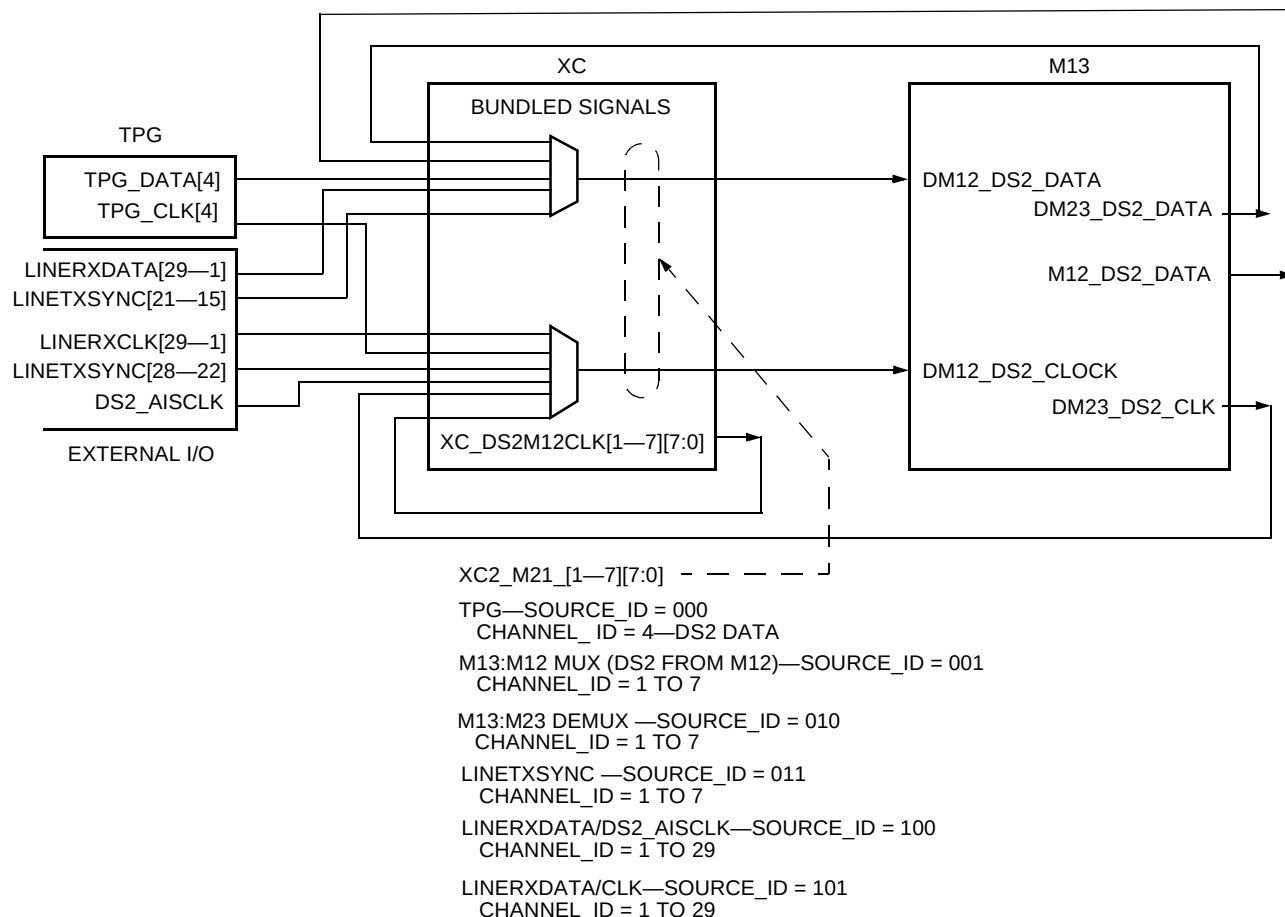
Figure 91. M12 DeMUX Input DS2 Cross Connect
