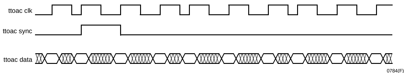
Figure 23. TMUX TTOAC and RTOAC Timing Diagram
