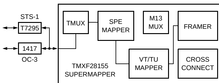
Figure 120. Internal Framer Line Side RX → TX DS1 Loopback Without Cross Connect
