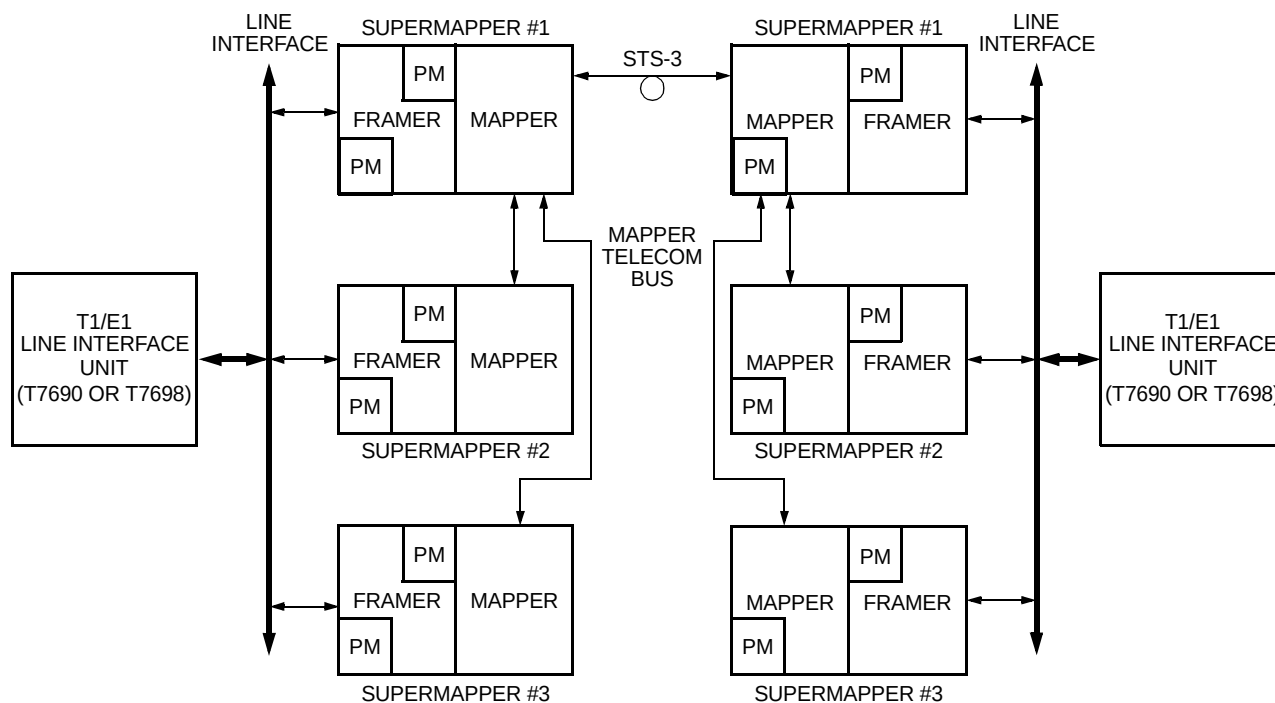
Figure 104. Transport Application of the Supermapper
