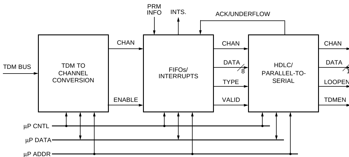
Figure 66. Transmit HDLC FIFO Block Diagram
