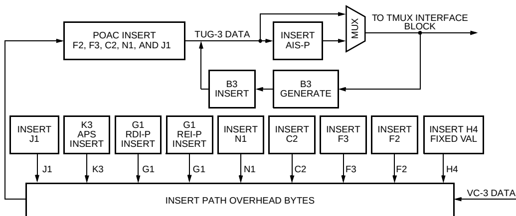
Figure 38. Transmit Direction Path Insertion Block
