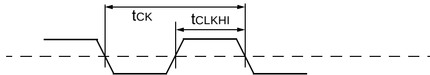
Figure 8. DS3DATAOUTCLK Timing
