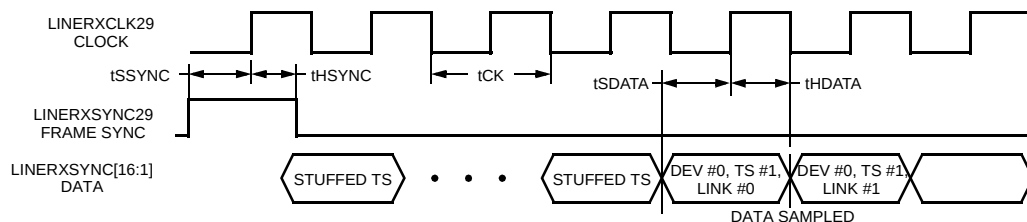
Figure 14. Parallel System Bus Interface Receive I/O Timing
