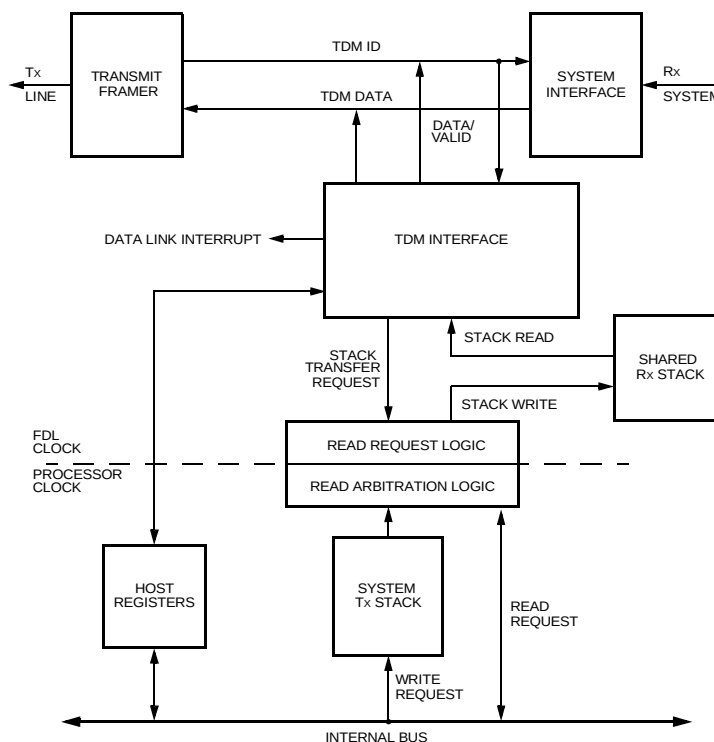
Figure 64. Tx Data Link Block Diagram
