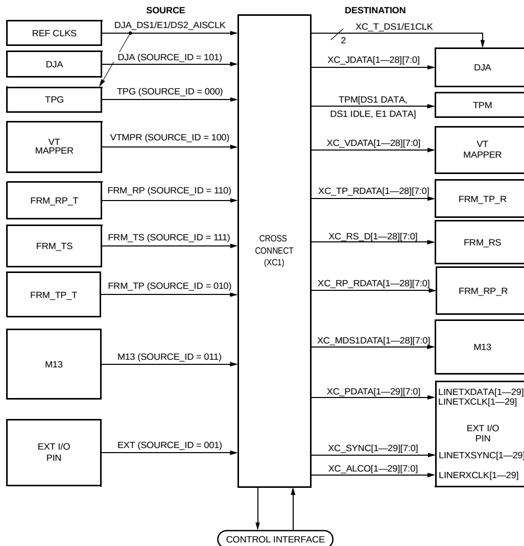
Figure 84. DS1 Cross Connect Interface
