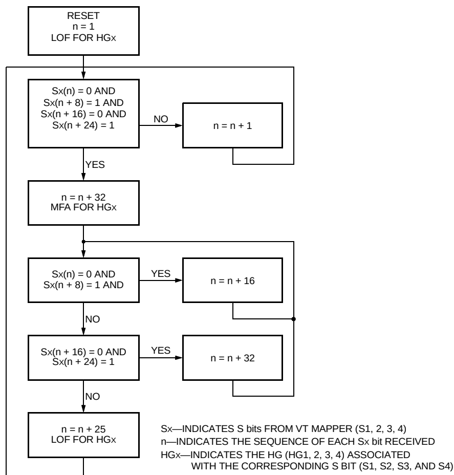
Figure 61. HG Alignment Algorithm
