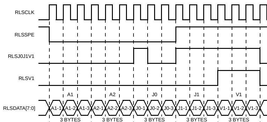
Figure 28. Receive Low-Speed Bus Interface Signals for STS-3/STM-1 Signals
