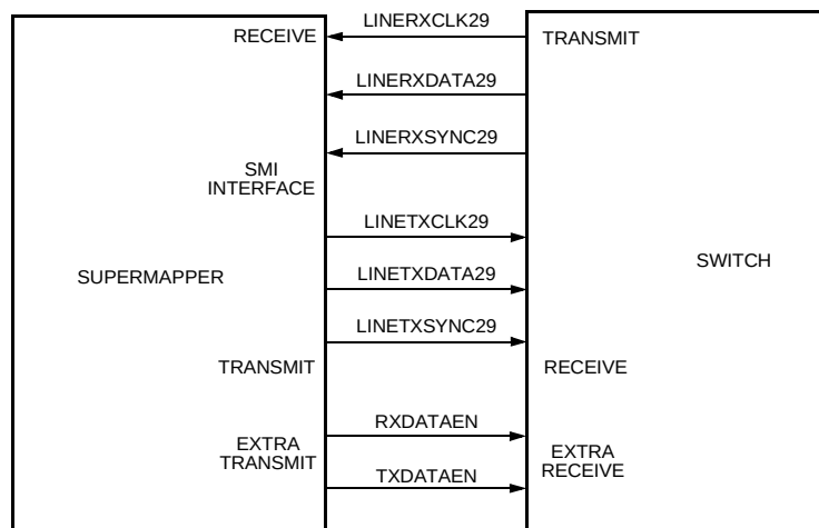
Figure 79. Signals (8-Pin Mode)
