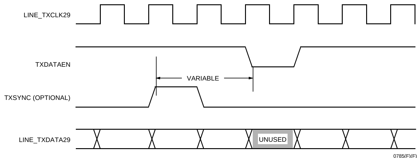
Figure 35. STS-1 NSMI Transmit Operation
