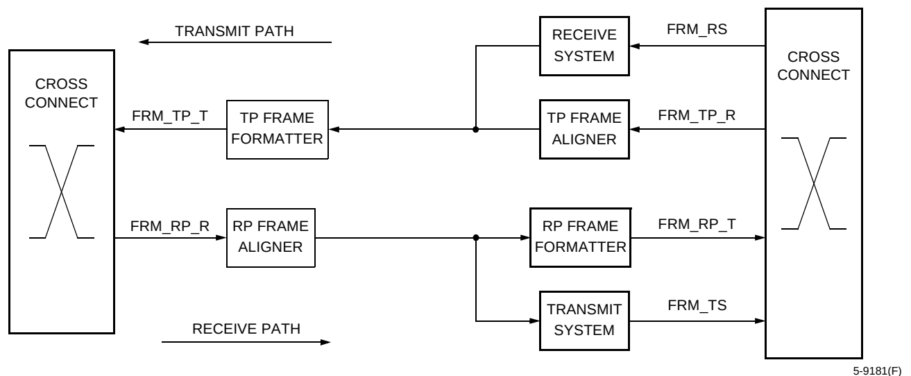
Figure 83. Framer and Cross Connect
