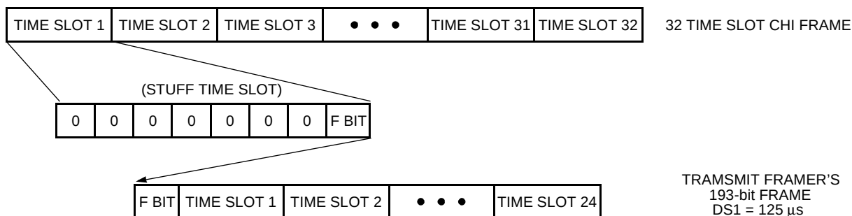
Figure 59. DS1 Transparent Frame Structure
