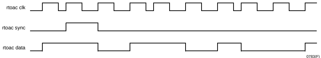
Figure 22. TMUX RTOAC Timing Diagram
