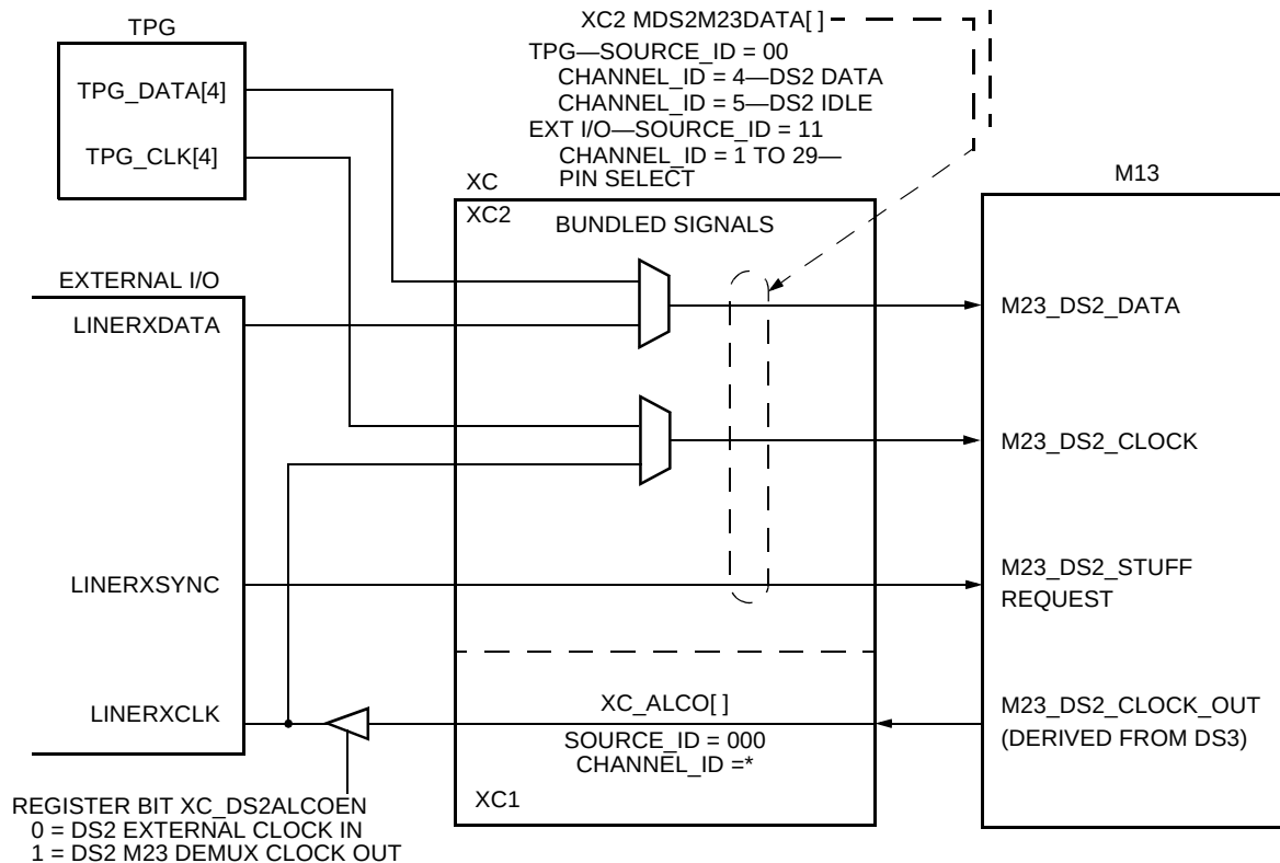
Figure 93. M23 MUX DS2 Input Cross Connect
