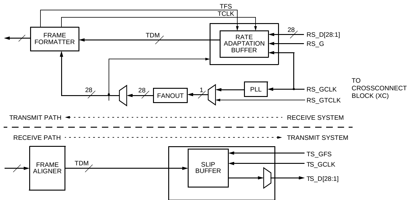
Figure 70. CHI Mode of the Transmit System Interface
