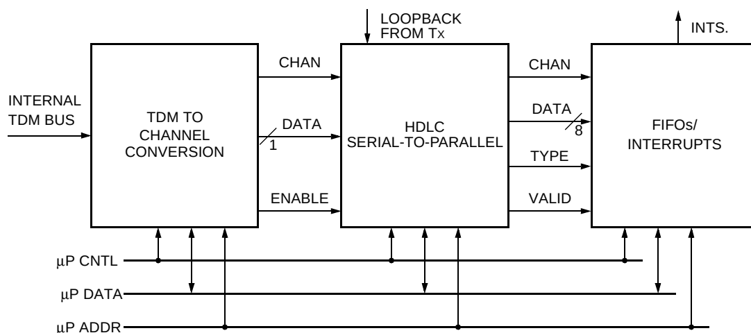
Figure 65. Receive HDLC Block Diagram
