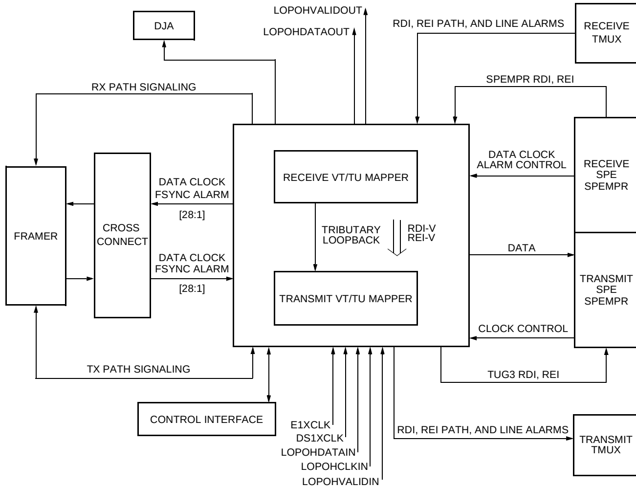
Figure 39. VT Mapper Interface Diagram
