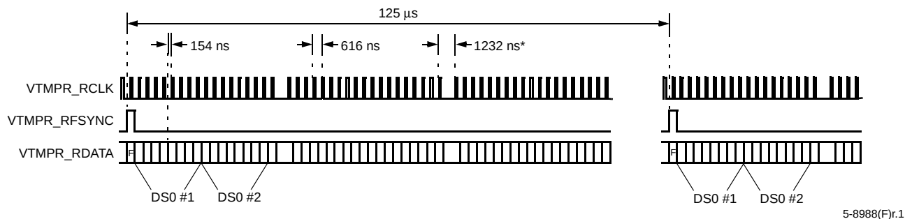
Figure 44. DS1 Interface
