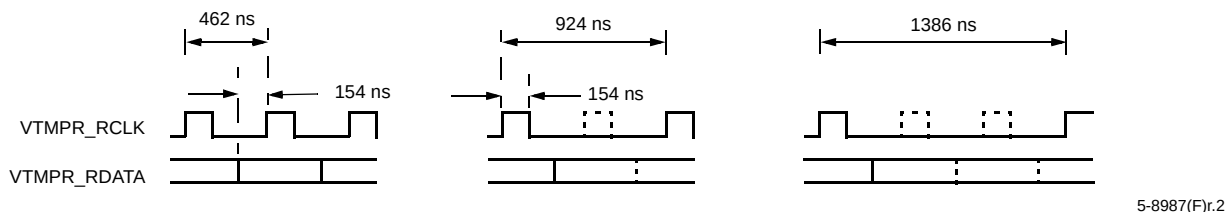
Figure 43. E1 Mode Gapped Clocking Scheme
