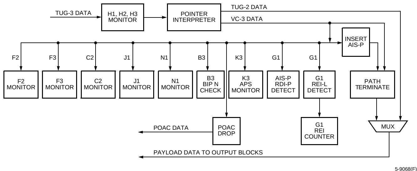
Figure 36. Receive Direction Path Termination Block
