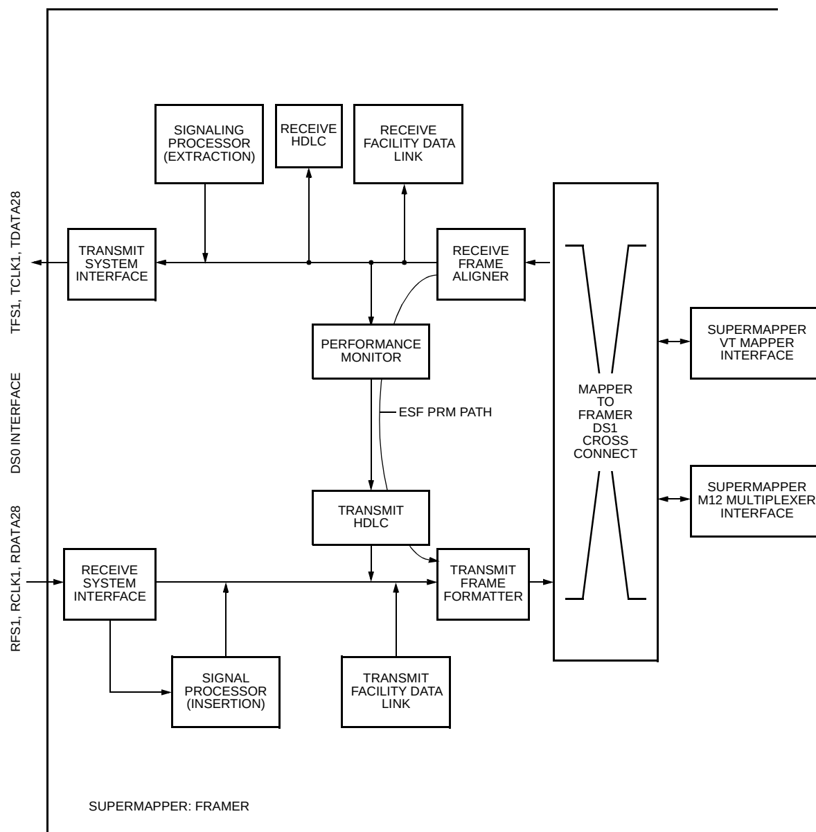
Figure 105. Supermapper Switching Mode for Framer in Concentration Highway Interface (CHI) Configuration
