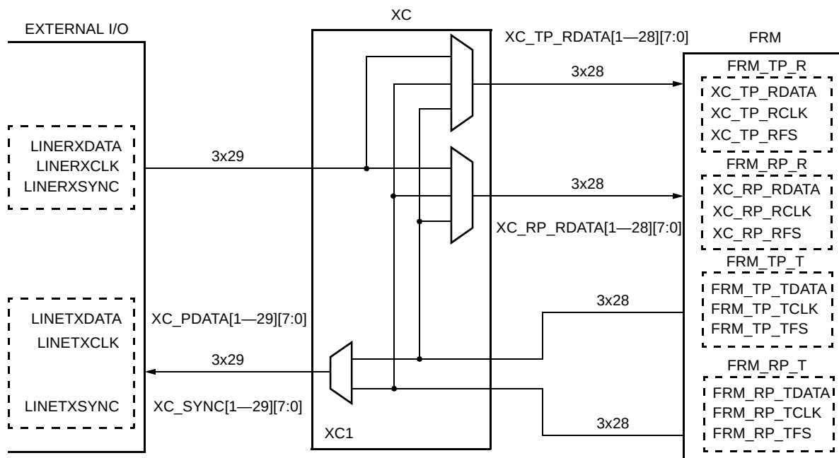
Figure 86. Framer Line Interface Cross Connect
