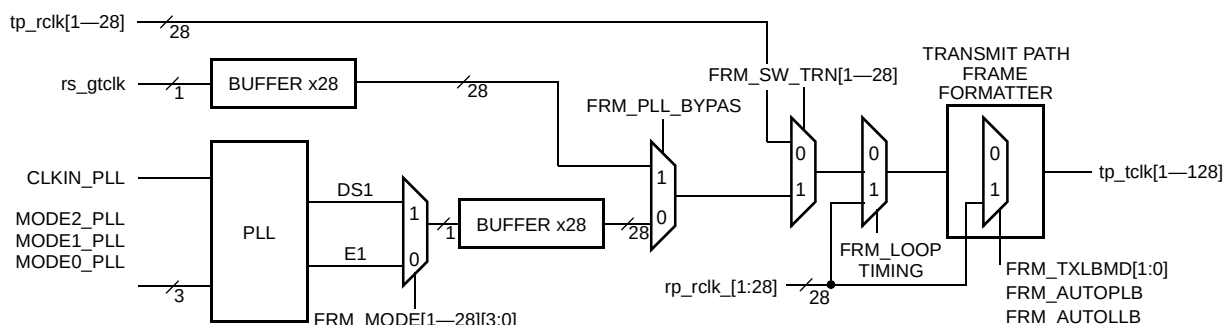
Figure 68. Framer Block Transmit Path Timing Selection
