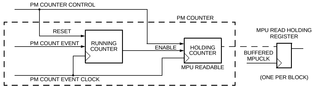
Figure 20. PM Reset Counter
