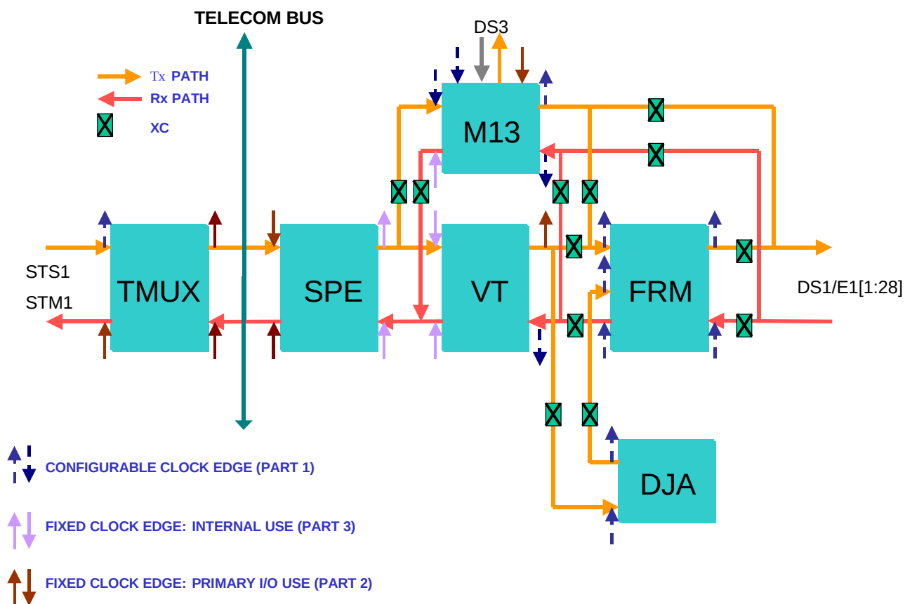
Figure 121. Clock Edges in Supermapper
