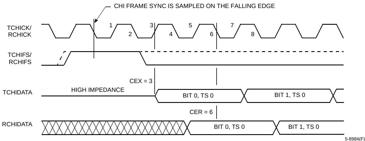
Figure 75. CHI TCHIDATA and RCHIDATA to CHICK Relationship with FRM_CMS = 1
