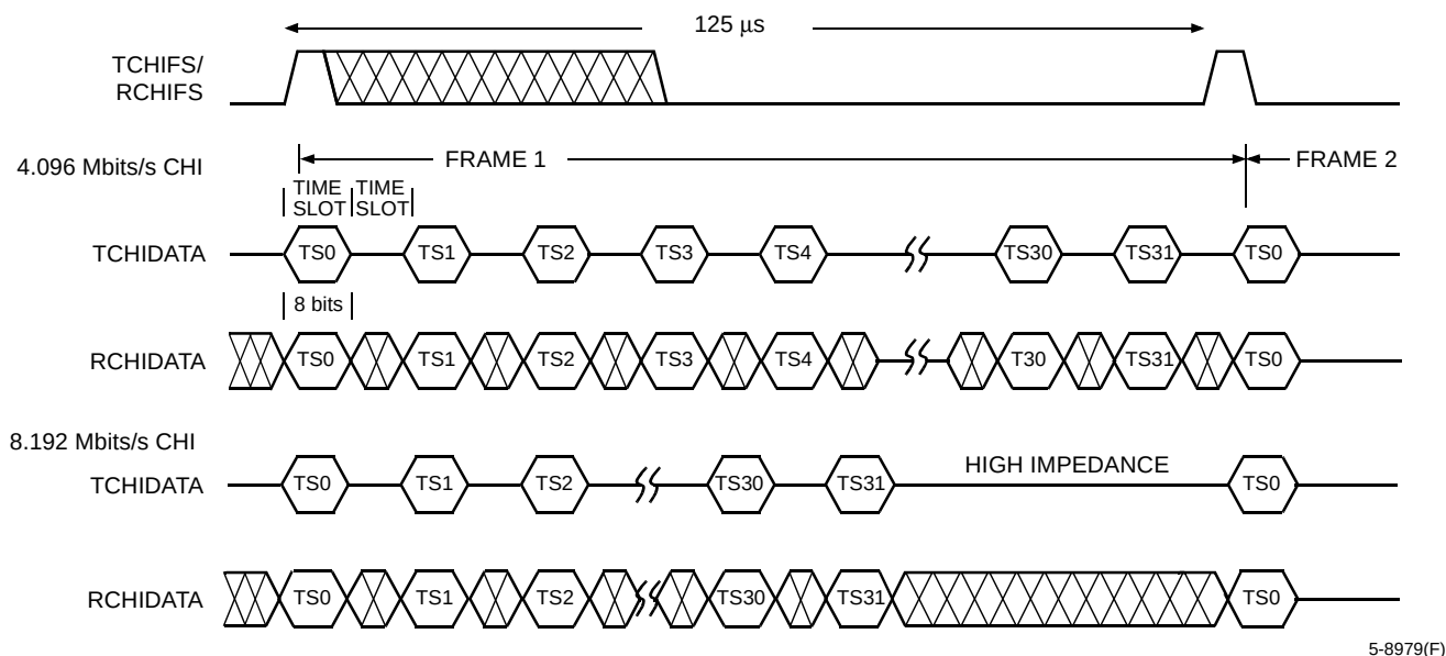
Figure 72. CHIDTS Mode Concentration Highway Interface Timing
