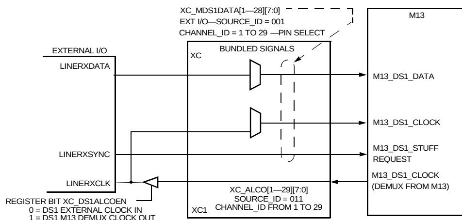
Figure 85. DS1/E1 External I/O to M13
