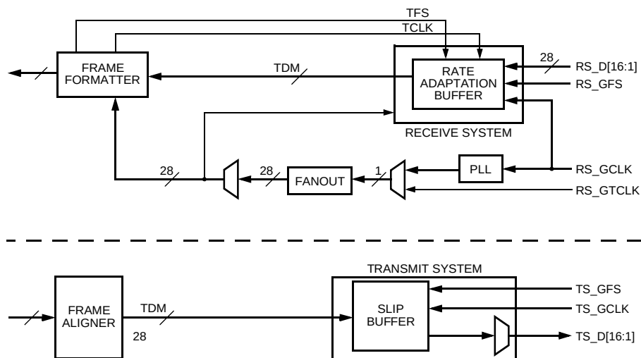
Figure 76. Parallel Bus System Interface Mode of the Transmit System Interface
