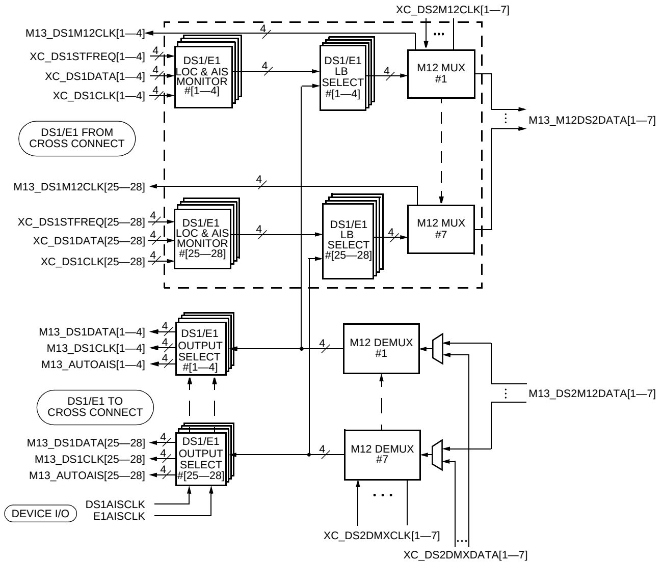
Figure 49. M12 Functional Block Diagram
