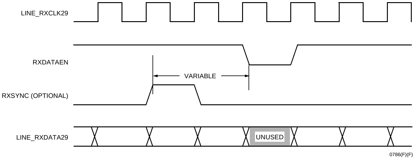
Figure 34. STS-1 NSMI Receive Operation
