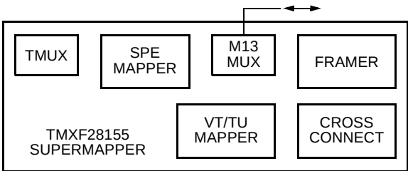
Figure 115. Loopback the DeMUXed DS1 or E1 Signals
