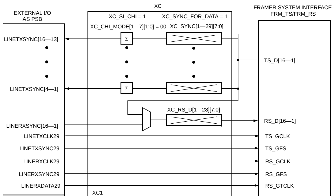
Figure 87. Framer System Interface—Parallel System Bus (PSB)
