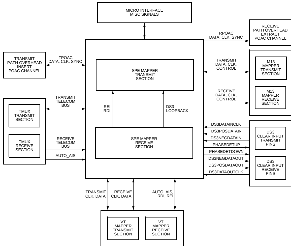
Figure 31. SPE Mapper Block with Connections to External Pins and Other Blocks in the Device
