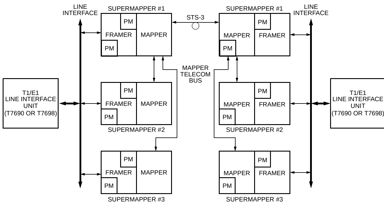
Figure 56. Transport Application of the Supermapper
