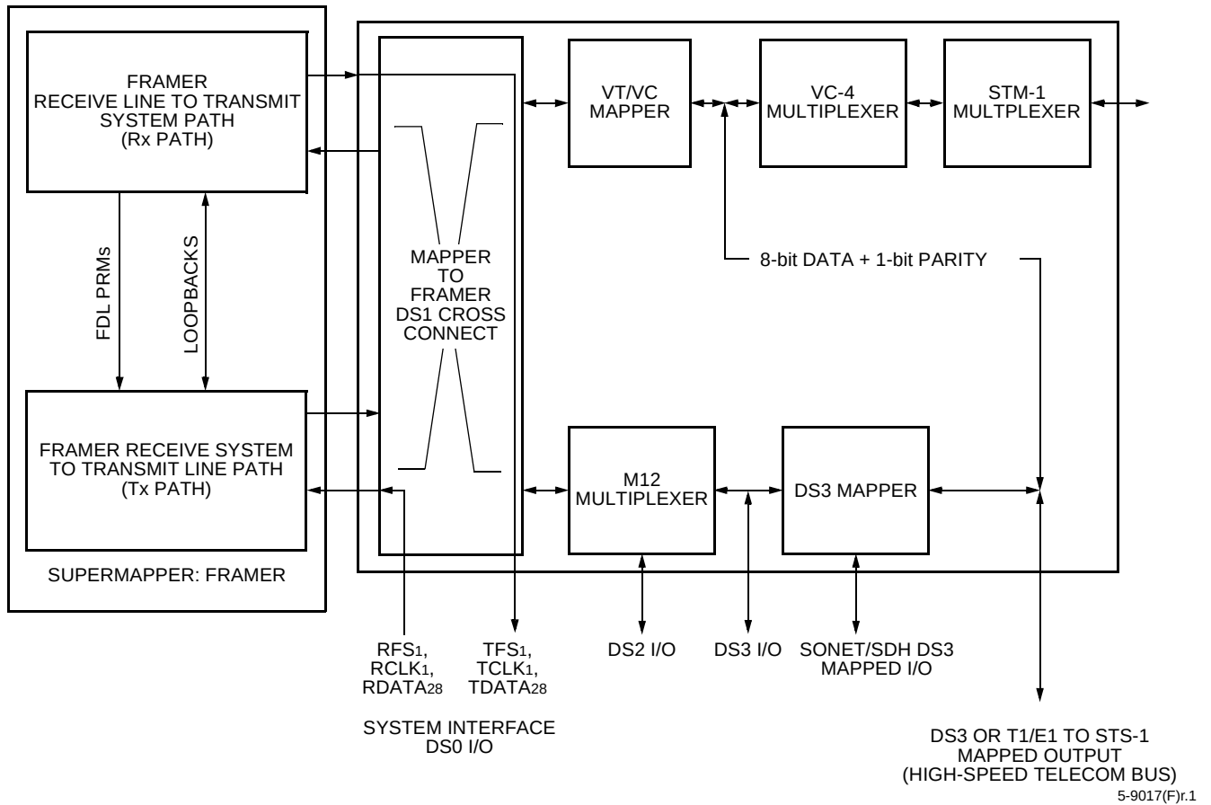
Figure 54. Supermapper Switching Configuration
