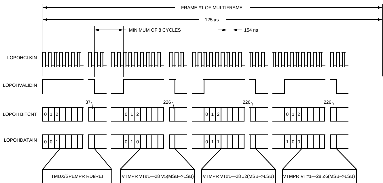
Figure 47. VT Mapper Transmit Path Overhead Serial Access Channel
