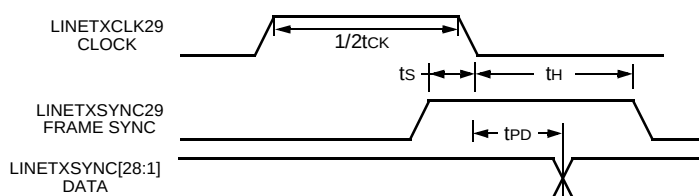
Figure 11. CHI Transmit I/O Timing
