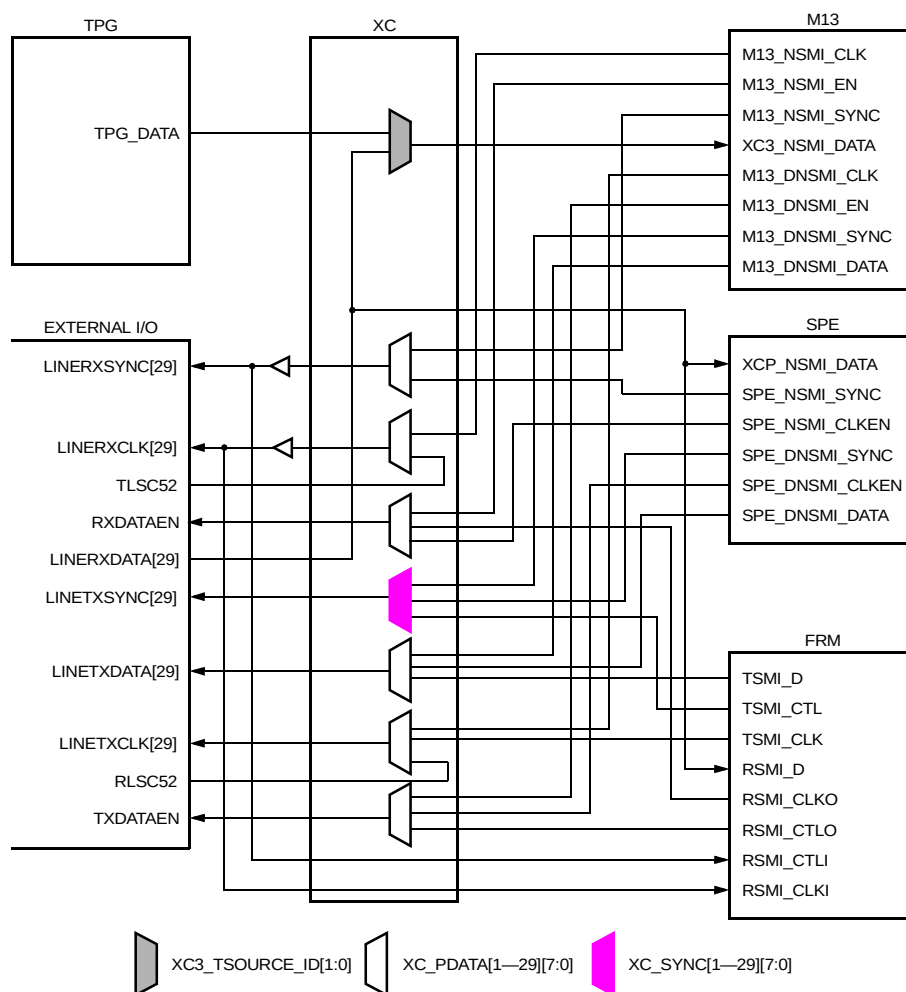
Figure 97. NSMI Interface Cross Connect
