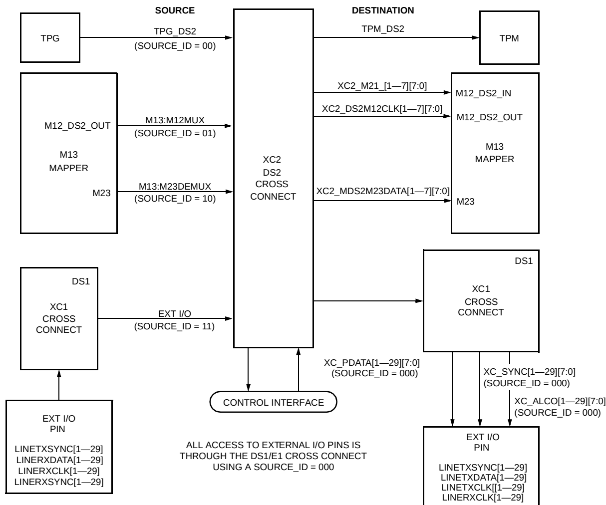
Figure 89. DS2 Cross Connect Interface
