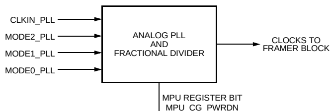
Figure 67. Framer PLL
