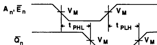
Waveform 2. For Non-Inverting Outputs
