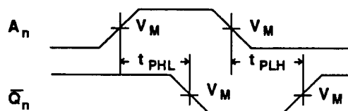
Waveform 1. For Inverting Outputs
