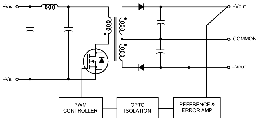
Figure 1. Simplified Schematic
