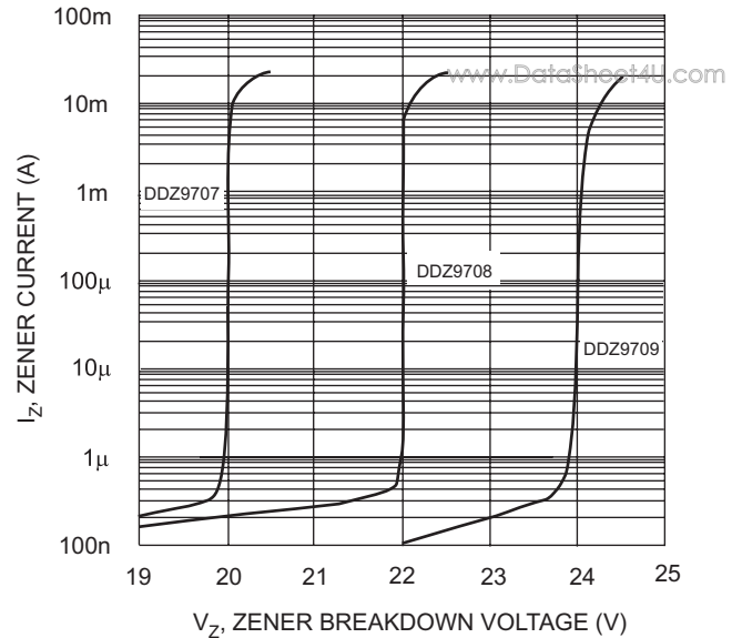
Fig. 7 Typical Reverse Characteristics, DDZ9707 - DDZ9709
