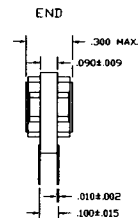
DPS45128, DPS45129
