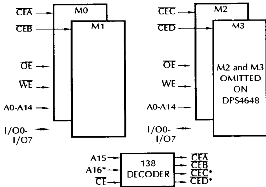
DPS4648, DPS41288
