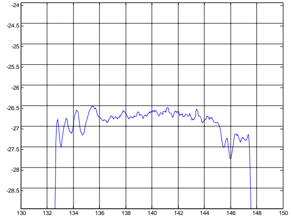
Phase Linearity(f0±7MHz)
