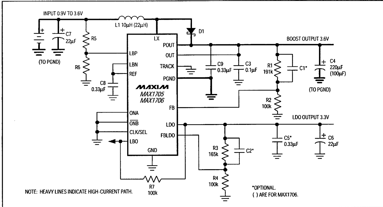
Figure 2. Typical Operating Circuit (PWM Mode)
