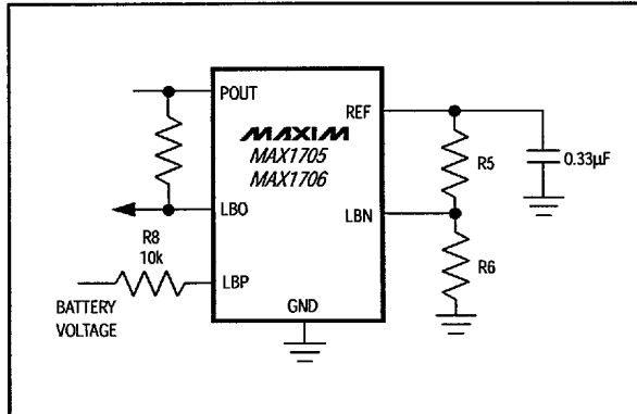
Figure 6. Detecting Battery Voltages Below 1.25V
