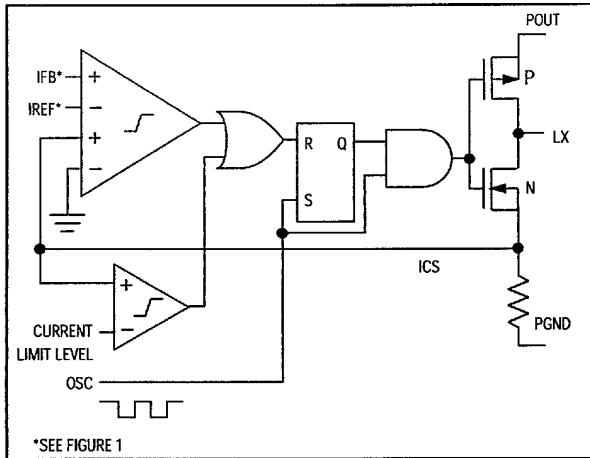
Figure 3. Simplified PWM Controller Block Diagram
