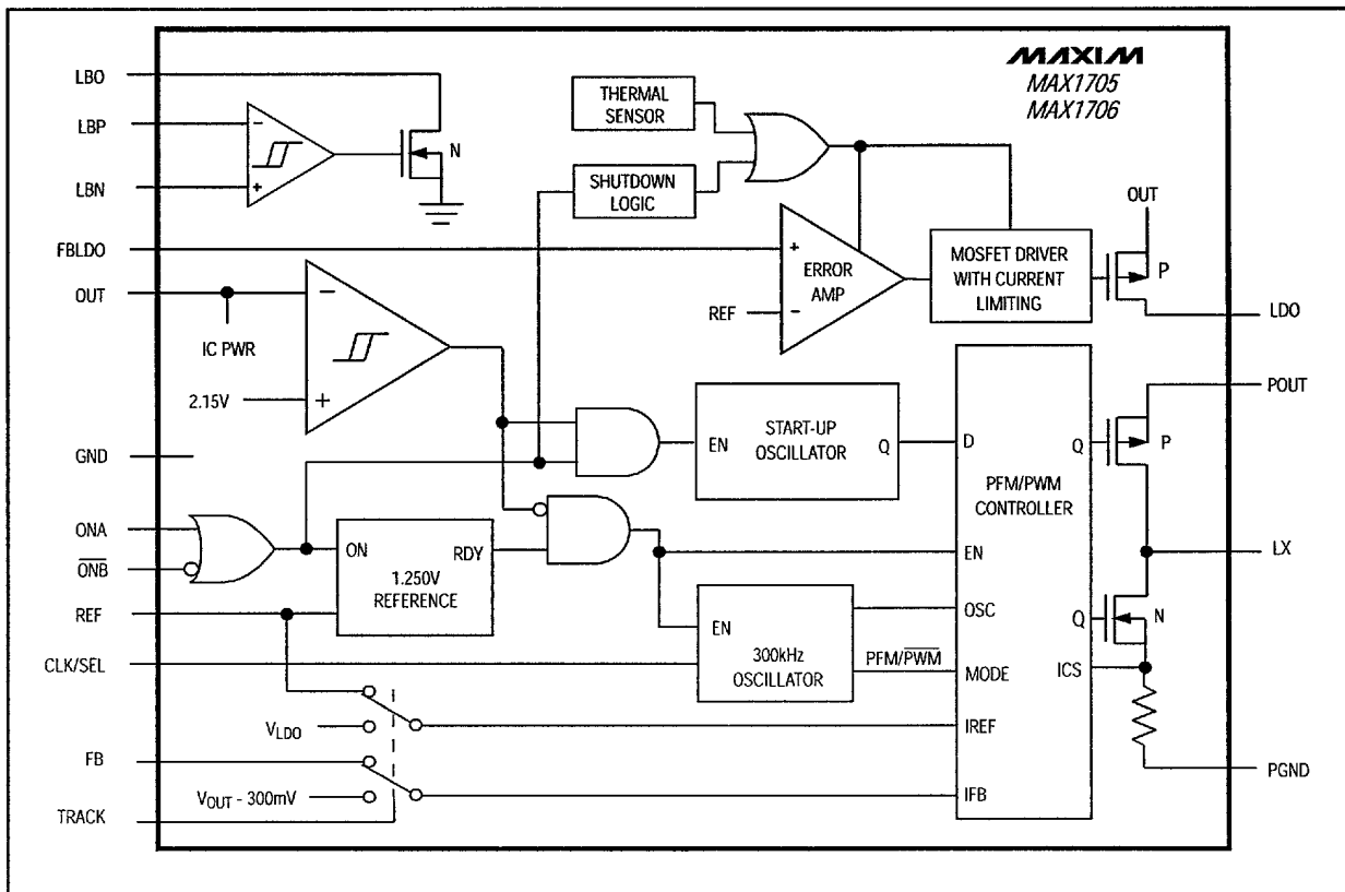
Figure 1. Functional Diagram
