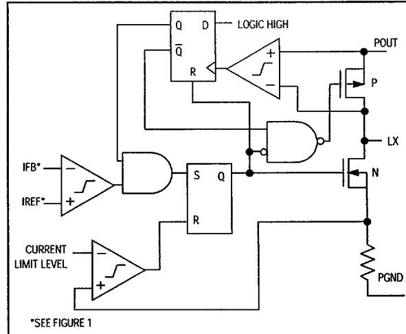
Figure 4. Controller Block Diagram in PFM Mode
