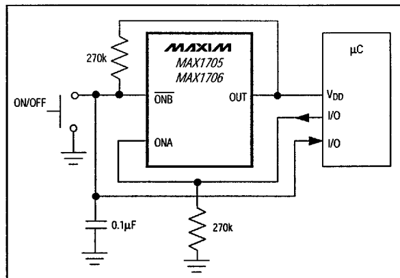
Figure 10. Momentary Pushbutton On/Off Switch
