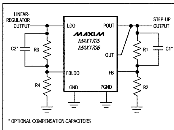
Figure 8. Feedback Connections for the MAX1705/MAX1706
