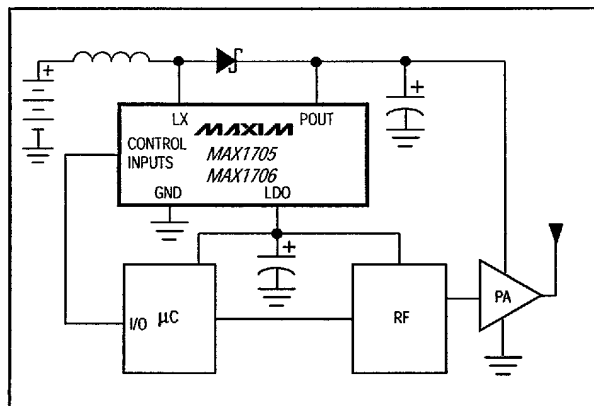
Figure 9. Typical Phone Application
