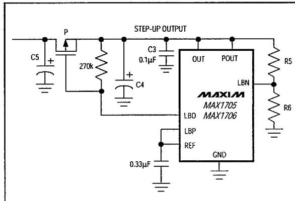
Figure 7. Using the Low-Battery Comparator for Load Control During Start-Up
