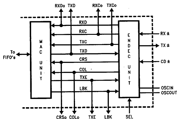
FIGURE 8-1. MAC and Internal ENDEC Interface Signals
