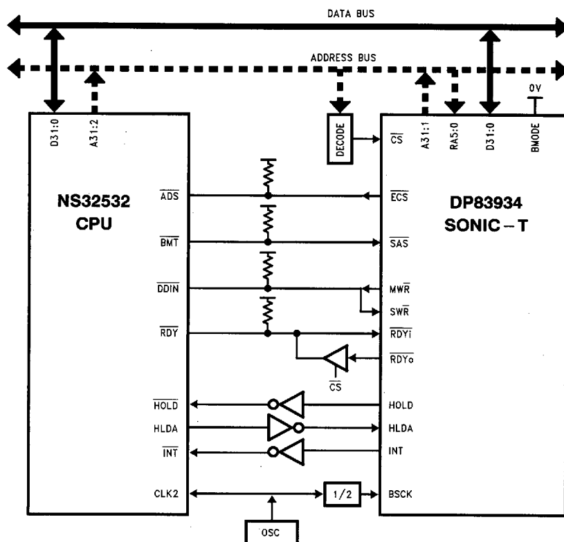
FIGURE 7-1. SONIC-T to NS32532 Interface Example
