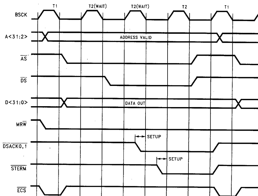
FIGURE 7-11. Memory Write, BMODE = 1, Asynchronous (2 Wait-State)
