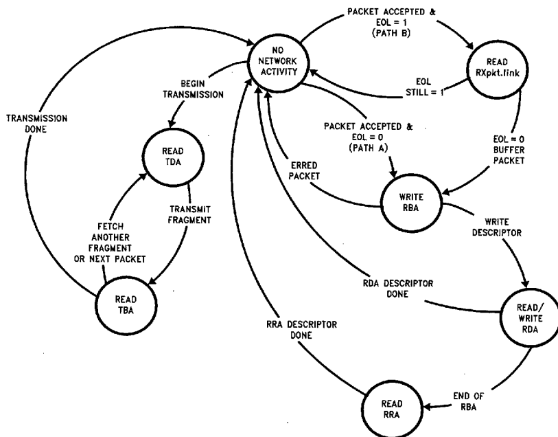
FIGURE 7-5. Bus Status Transitions
