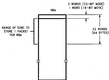
FIGURE 5-11. Setting EOBC for Single Packet RBA
