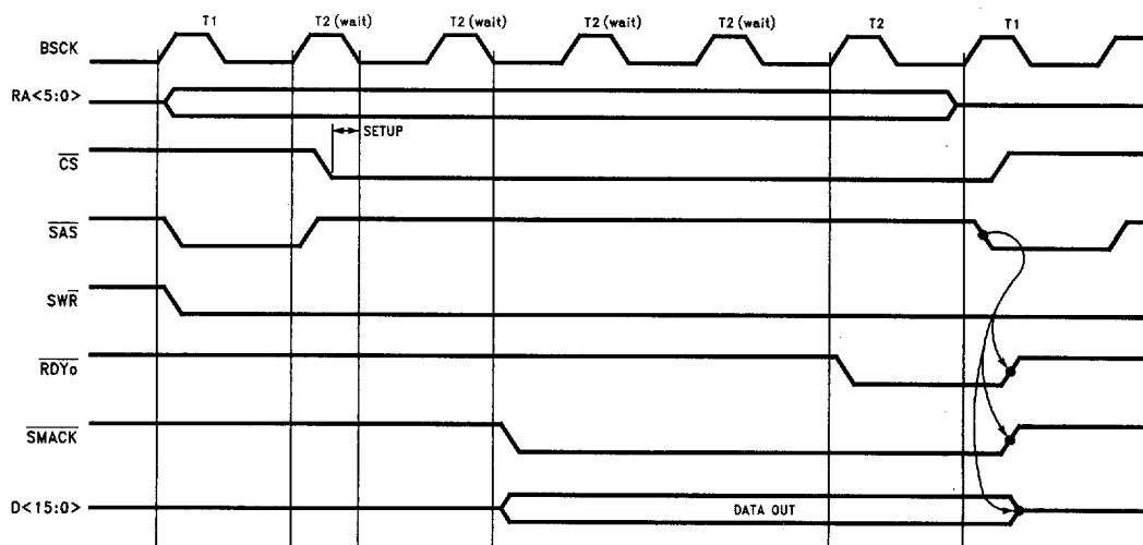
FIGURE 7-21. Register Read, BMODE = 0
