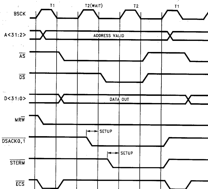
FIGURE 7-10. Memory Write, BMODE = 1, Asynchronous (1 Wait-State)
