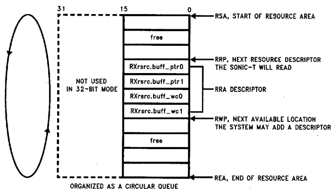
FIGURE 5-4. Receive Resource Area Format
