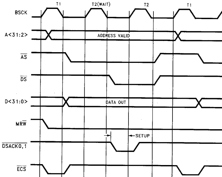
FIGURE 7-7. Memory Write, BMODE = 1, Synchronous (1 Wait-State)
