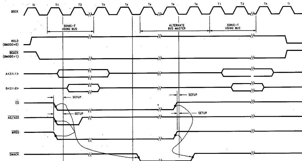
FIGURE 7-23. On-Chip Memory Arbitration
