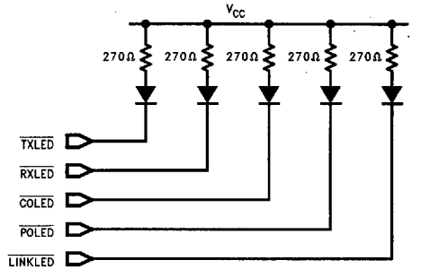
FIGURE 3-4. Typical SONIC-T LED Connection
