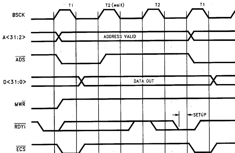
FIGURE 7-13. Memory Write, BMODE = 0, Synchronous (1 Wait-State)
