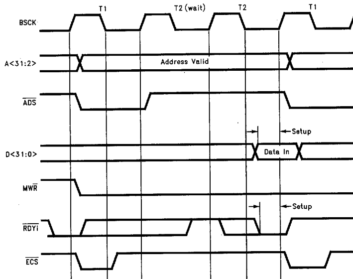
FIGURE 7-12. Memory Read, BMODE = 0, Synchronous (1 Wait-State)
