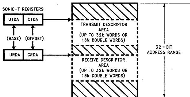
FIGURE 5-2. Transmit and Receive Descriptor Area Pointers
