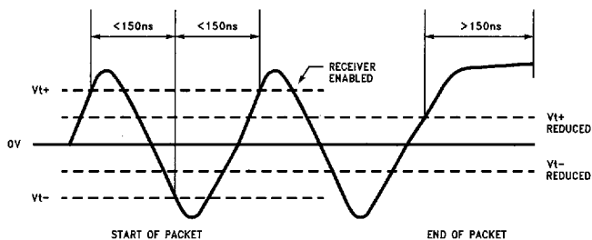
FIGURE 3-2. Twisted Pair Squelch Waveform (10BASE-T Mode)
