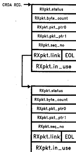
FIGURE 5-10. RDA Initialization Example
