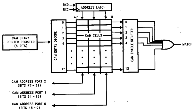
FIGURE 6-1. CAM Organization
