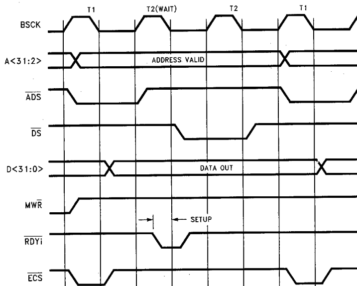
FIGURE 7-16. Memory Write, BMODE = 0, Asynchronous (1 Wait-State)
