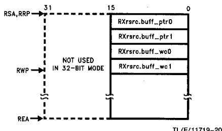
FIGURE 5-9. RRA Initialization
