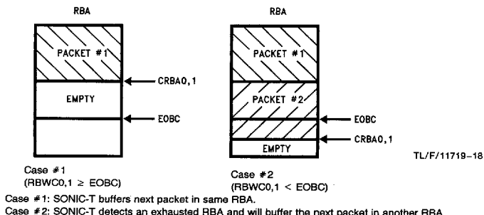
FIGURE 5-5. Receive Buffer Area
