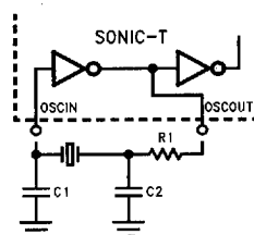
FIGURE 8-4. Crystal Connection to the SONIC-T (see text)
