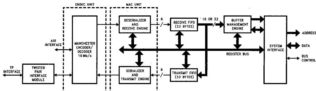
FIGURE 3-1. SONIC-T Block Diagram
