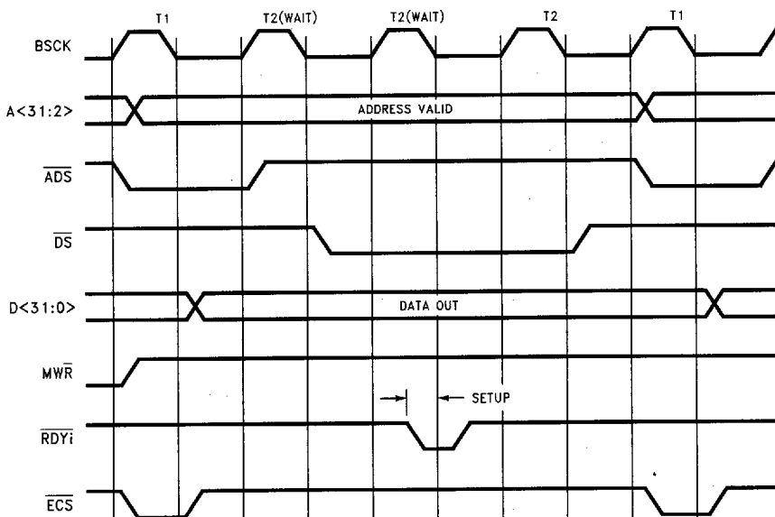
FIGURE 7-17. Memory Write, BMODE = 0, Asynchronous (2 Wait-State)
