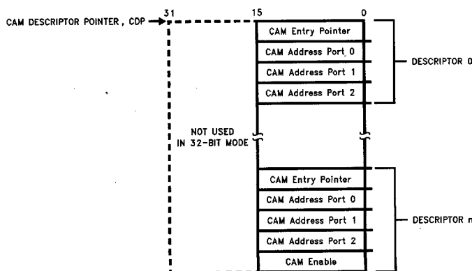
FIGURE 6-2. CAM Descriptor Area Format
