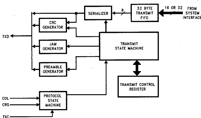
FIGURE 3-7. MAC Transmitter
