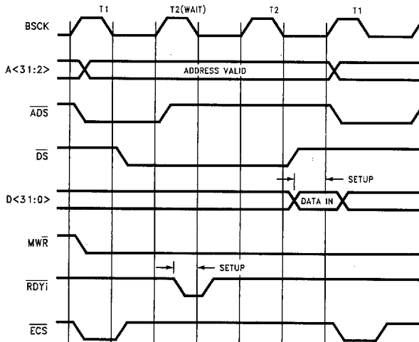
FIGURE 7-14. Memory Read, BMODE = 0, Asynchronous (1 Wait-State)
