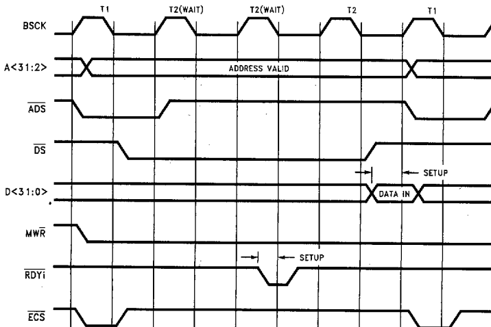
FIGURE 7-15. Memory Read, BMODE = 0, Asynchronous (2 Wait-State)
