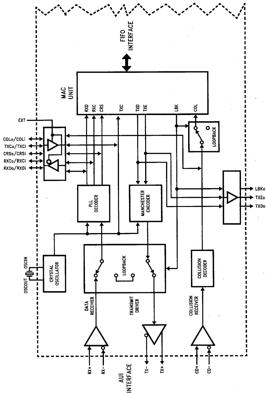
FIGURE 3-5. Block Diagram of Ethernet ENDEC
