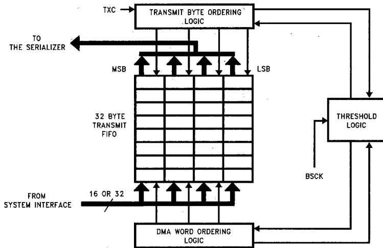
FIGURE 3-9. Transmit FIFO
