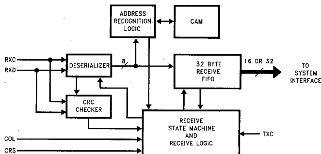
FIGURE 3-6. MAC Receiver
