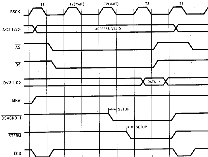
FIGURE 7-9. Memory Read, BMODE = 1, Asynchronous (2 Wait-State)
