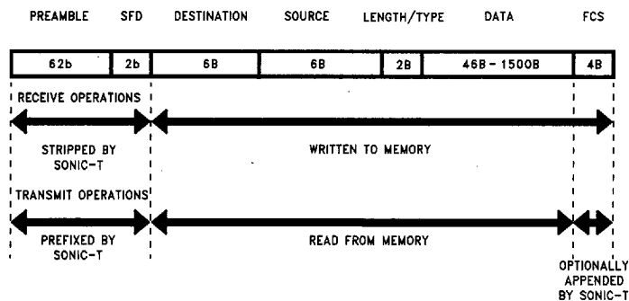
FIGURE 4-1. IEEE 802.3 Packet Structure
