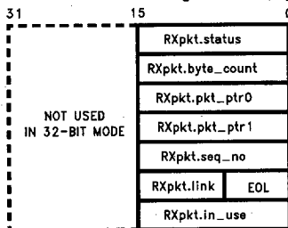
FIGURE 5-6. Receive Descriptor Format
