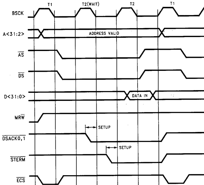
FIGURE 7-8. Memory Read, BMODE = 1, Asynchronous (1 Wait-State)
