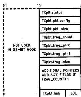
FIGURE 5-13. Transmit Descriptor Area
