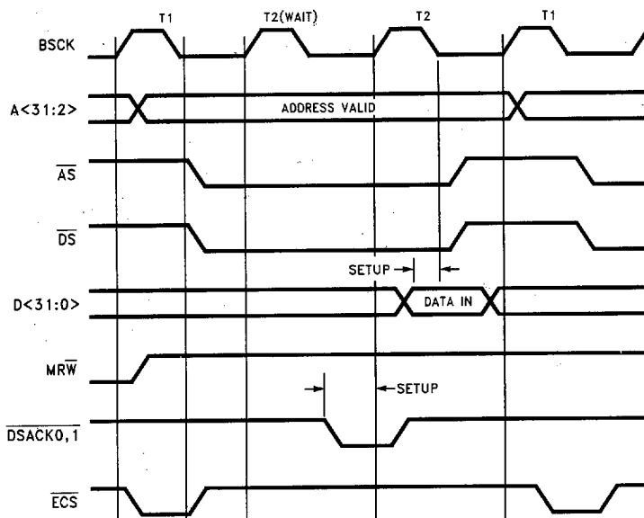
FIGURE 7-6. Memory Read, BMODE = 1, Synchronous (1 Wait-State)
