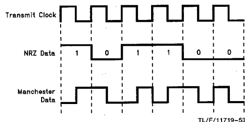
FIGURE 8.3. Manchester Encoded Data Stream
