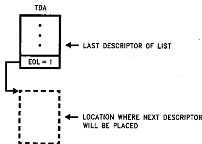
FIGURE 5-16. Initializing Last Link Field
