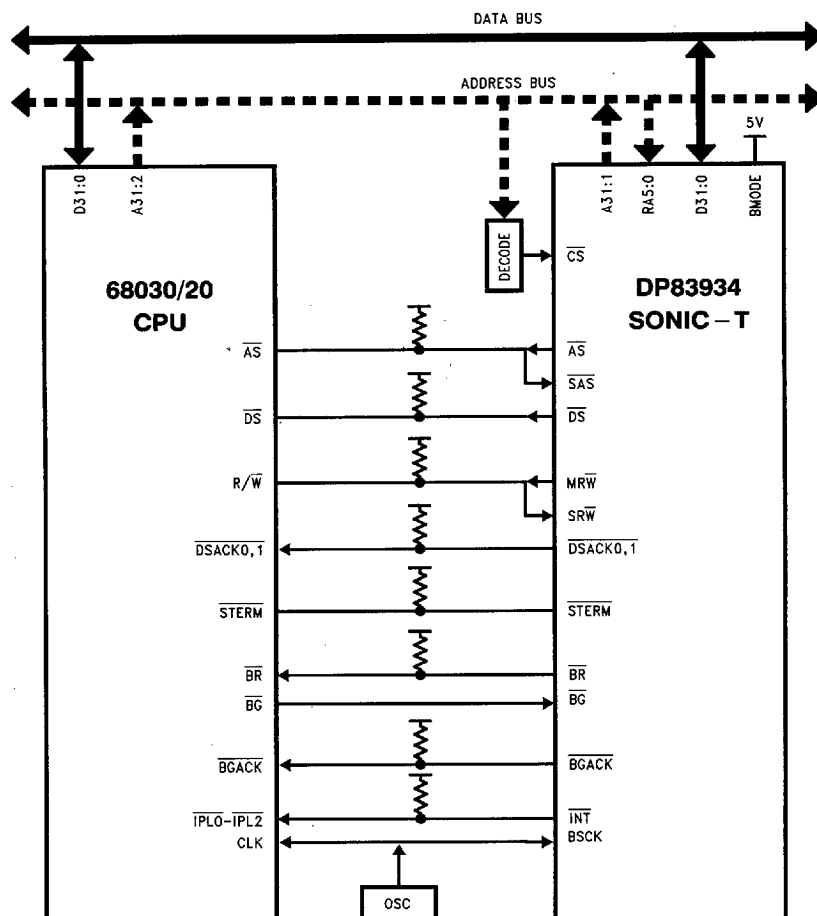
FIGURE 7-2. SONIC-T to Motorola 68030/20 Interface Example
