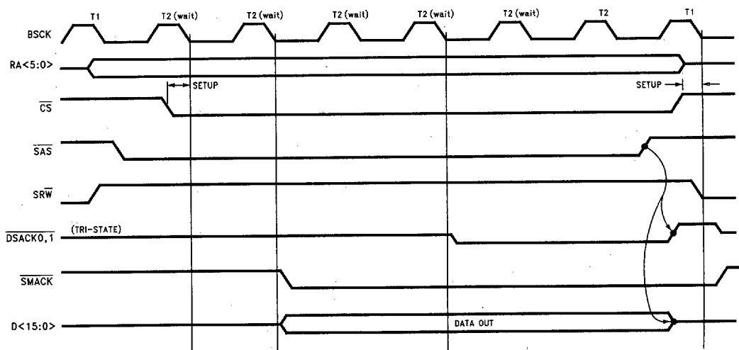
FIGURE 7-19. Register Read, BMODE = 1
