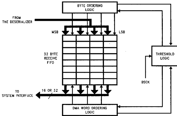
FIGURE 3-8. Receive FIFO
