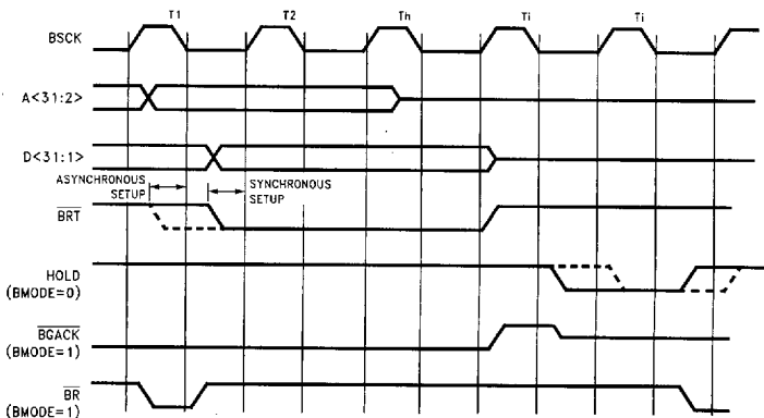
FIGURE 7-18. Bus Exception (Bus Retry)
