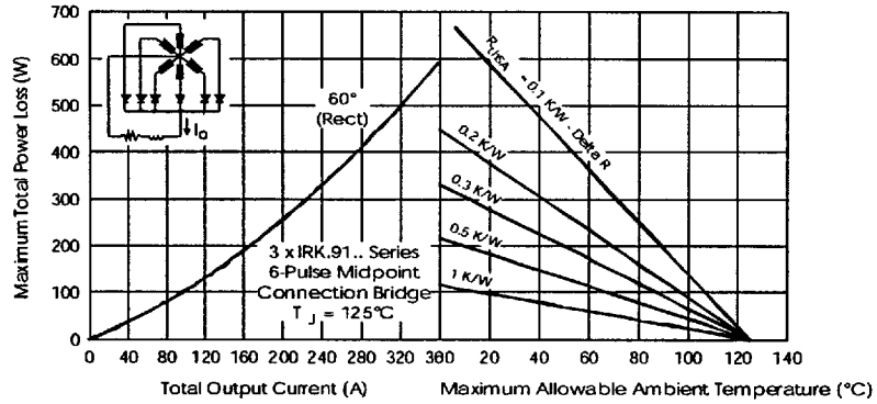
Fig. 16 - On-state Power Loss Characteristics
