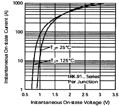
Fig. 18 - On-state Voltage Drop Characteristics
