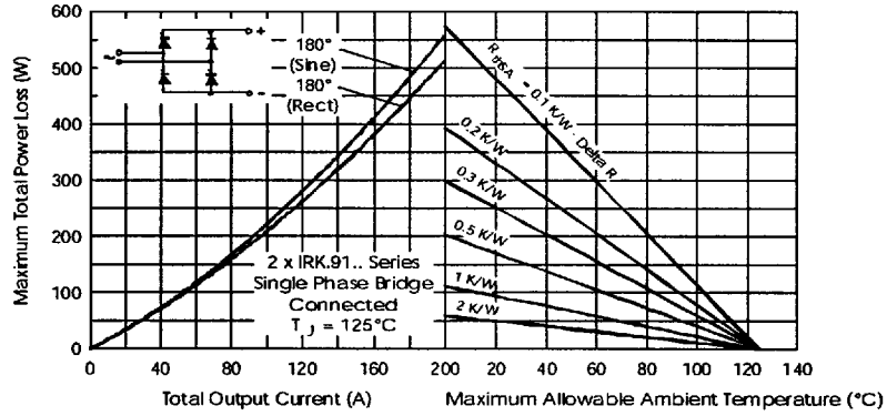
Fig. 15 - On-state Power Loss Characteristics (Single Phase Bridge IRKU+IRKV)
