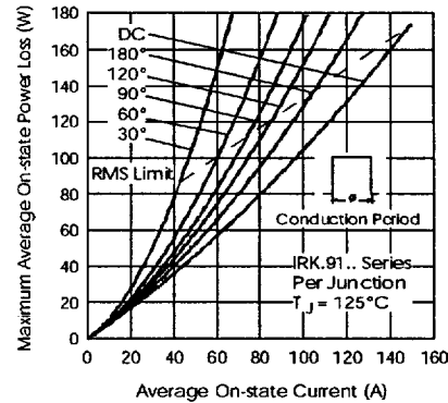
Fig. 12 - On-state Power Loss Characteristics
