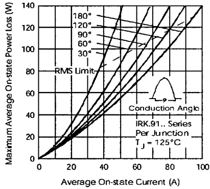
Fig. 11 - On-state Power Loss Characteristics
