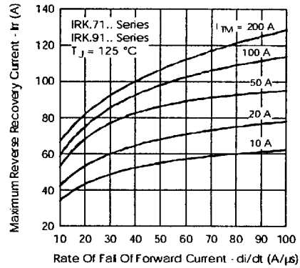
Fig. 20 - Recovery Current Characteristics
