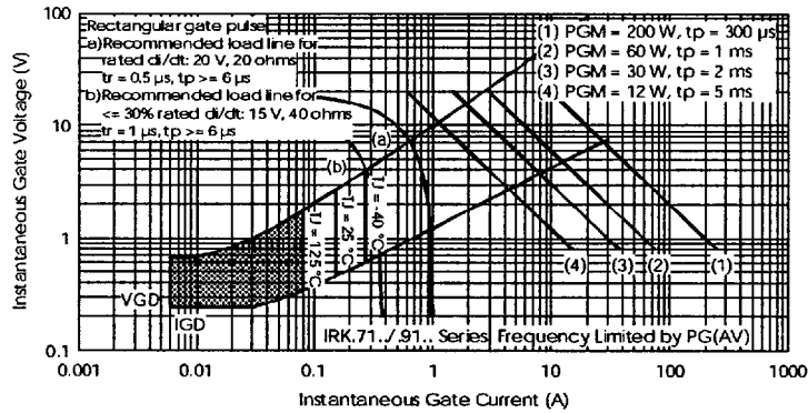
Fig. 22 - Gate Characteristics
