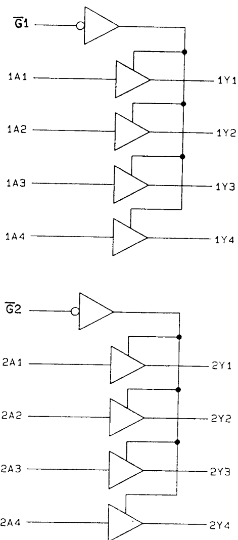
FIGURE 3. Logic diagram.
