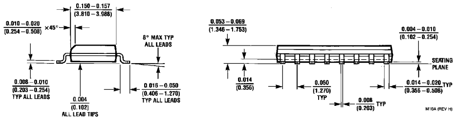
16-Lead Molded Package Small Outline (M) Order Number DS88LS120M NS Package Number M16A
