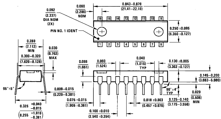
Molded Dual-In-Line Package (N) Order Number DS88LS120N NS Package Number N16A
