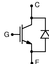
Fig.2 ITZ25C12 circuit
