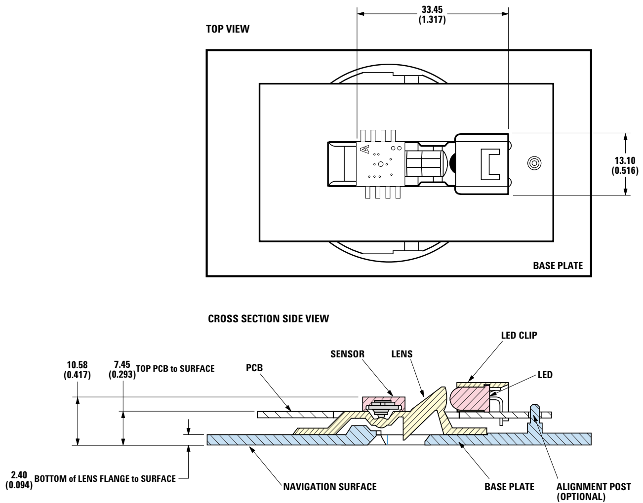
Figure 4. 2D Assembly drawing of ADNS-5030 (top and side view).
