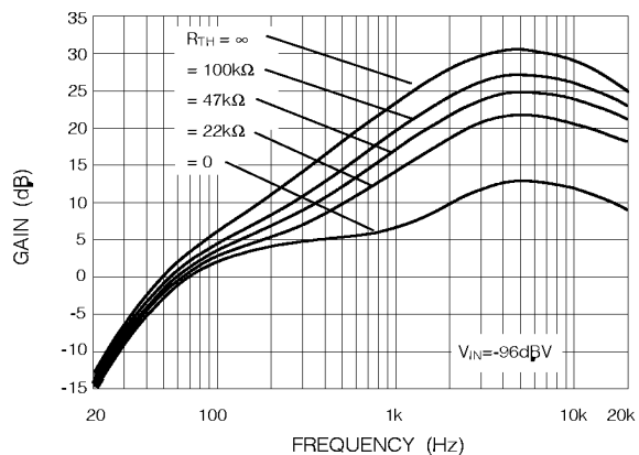
Fig. 9 Frequency Characteristics for Different R_{TH} Values
