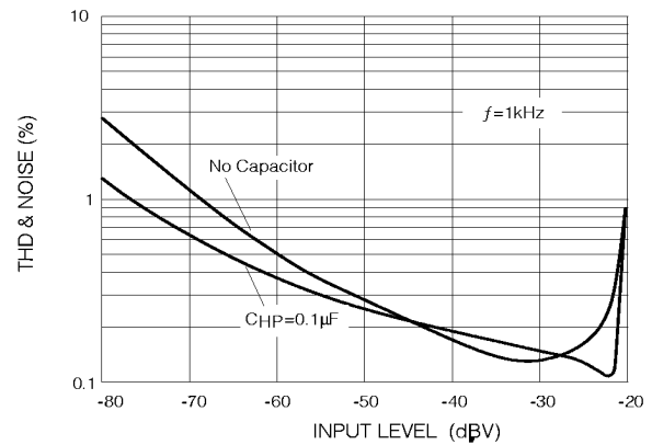
Fig. 13 THD & Noise vs Input Level
