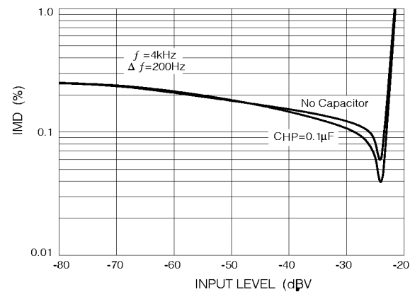
Fig. 15 Intermodulation Distortion (CCIF) vs Level
