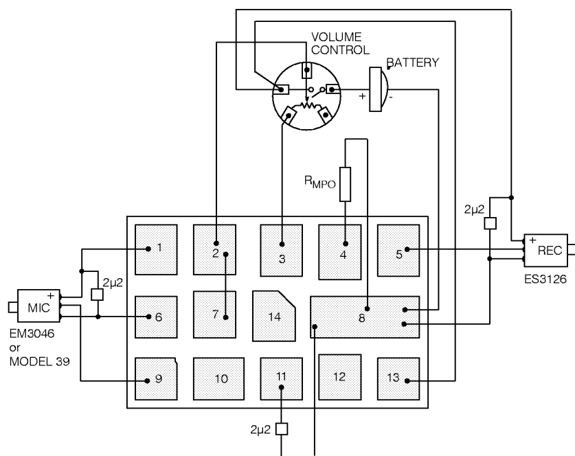
Fig. 3 Typical Assembly Diagram
