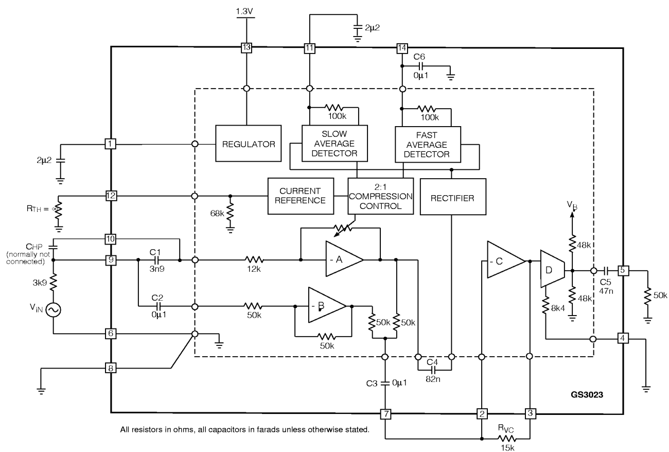
Fig. 4 Characterization Circuit (used to generate typical curves)
