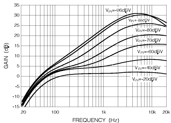
Fig. 5 Frequency Response for Different Input Levels
