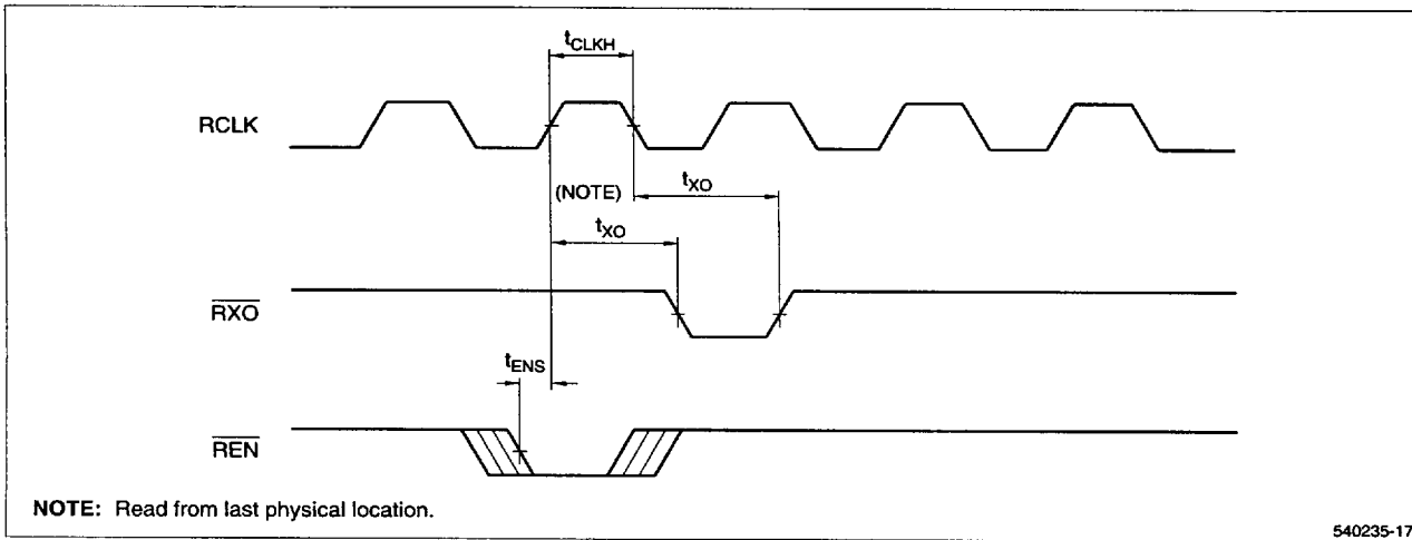
Figure 23. Read-Expansion-Out Timing, IDT-Compatible Operating Mode
