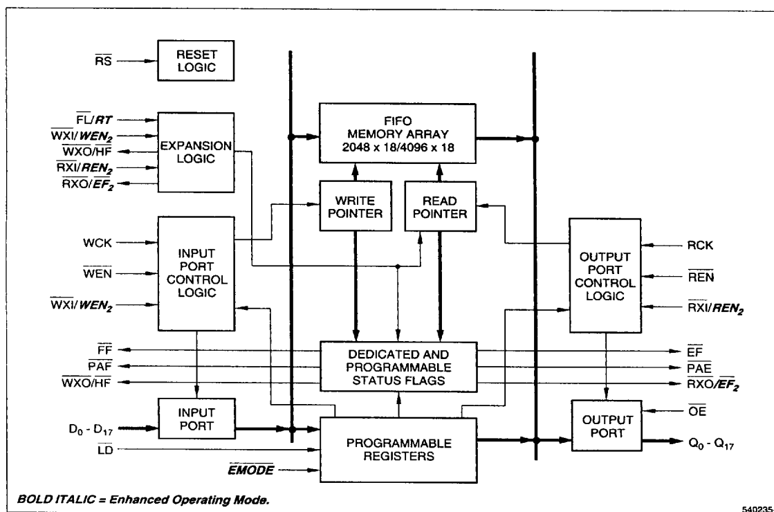
Figure 1. LH540235/45 Block Diagram
