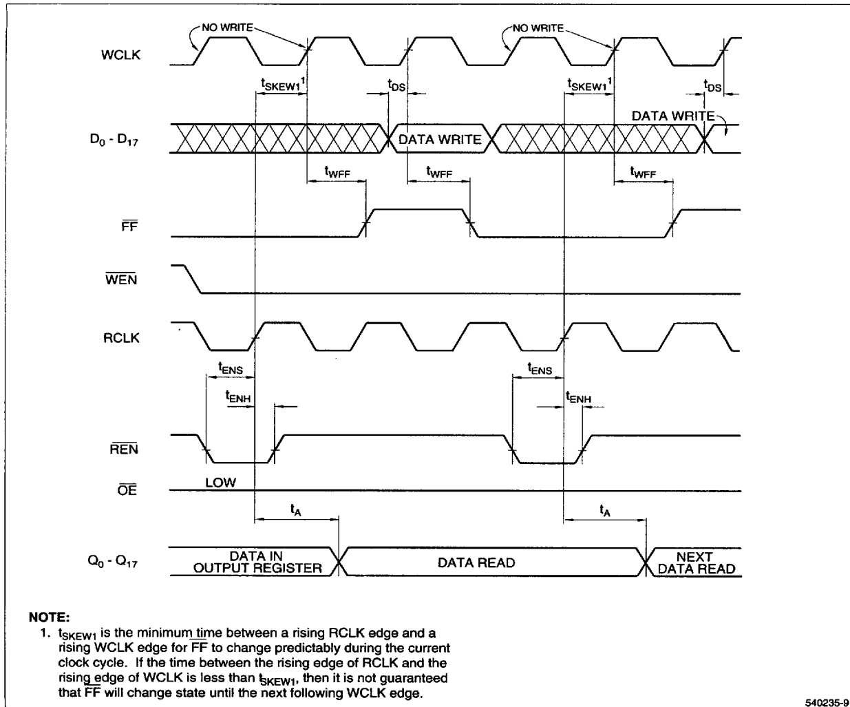
Figure 10. Full-Flag Timing
