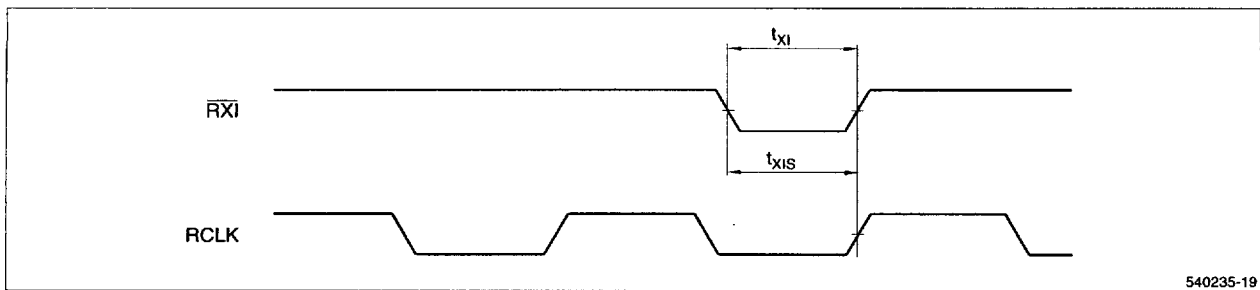
Figure 25. Read-Expansion-In Timing, IDT-Compatible Operating Mode
