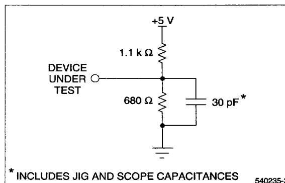
Figure 4. Output Load Circuit
