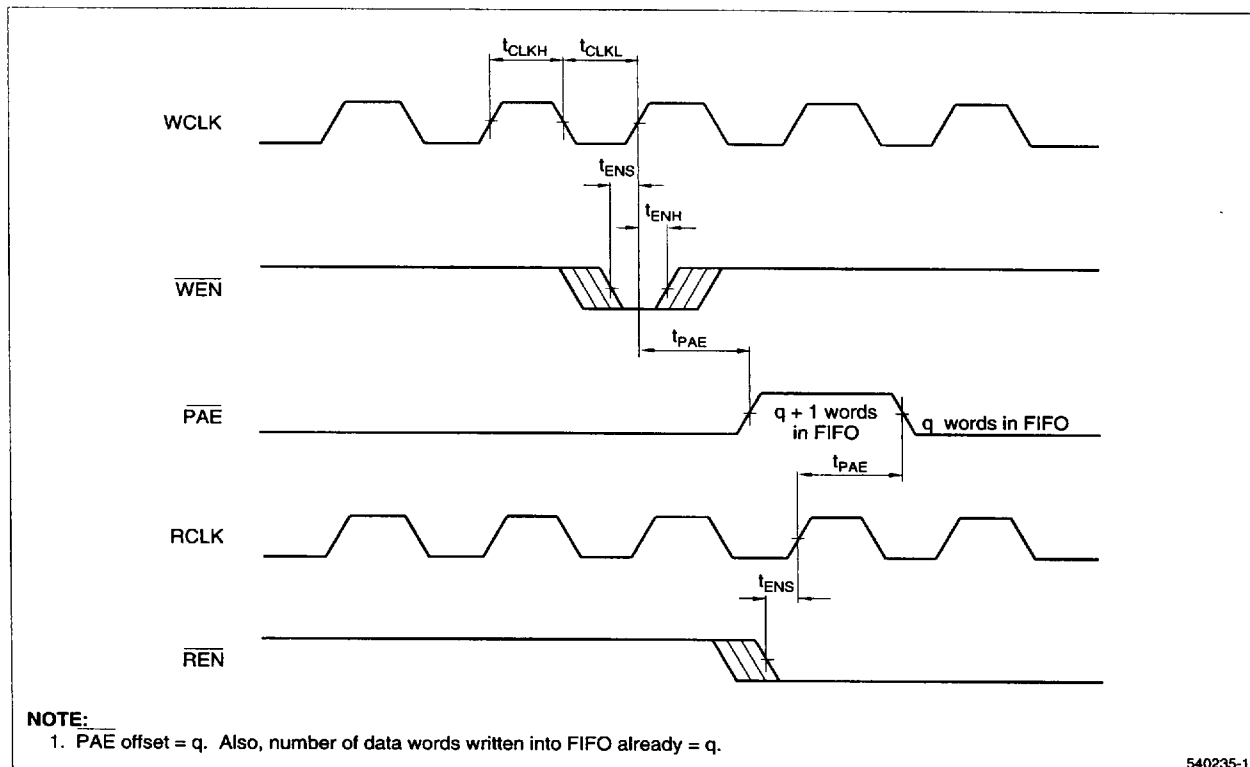
Figure 14. Programmable-Almost-Empty Flag Timing, IDT-Compatible Operating Mode
