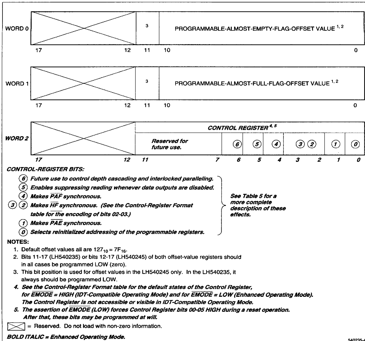
Figure 5. Programmable Registers
