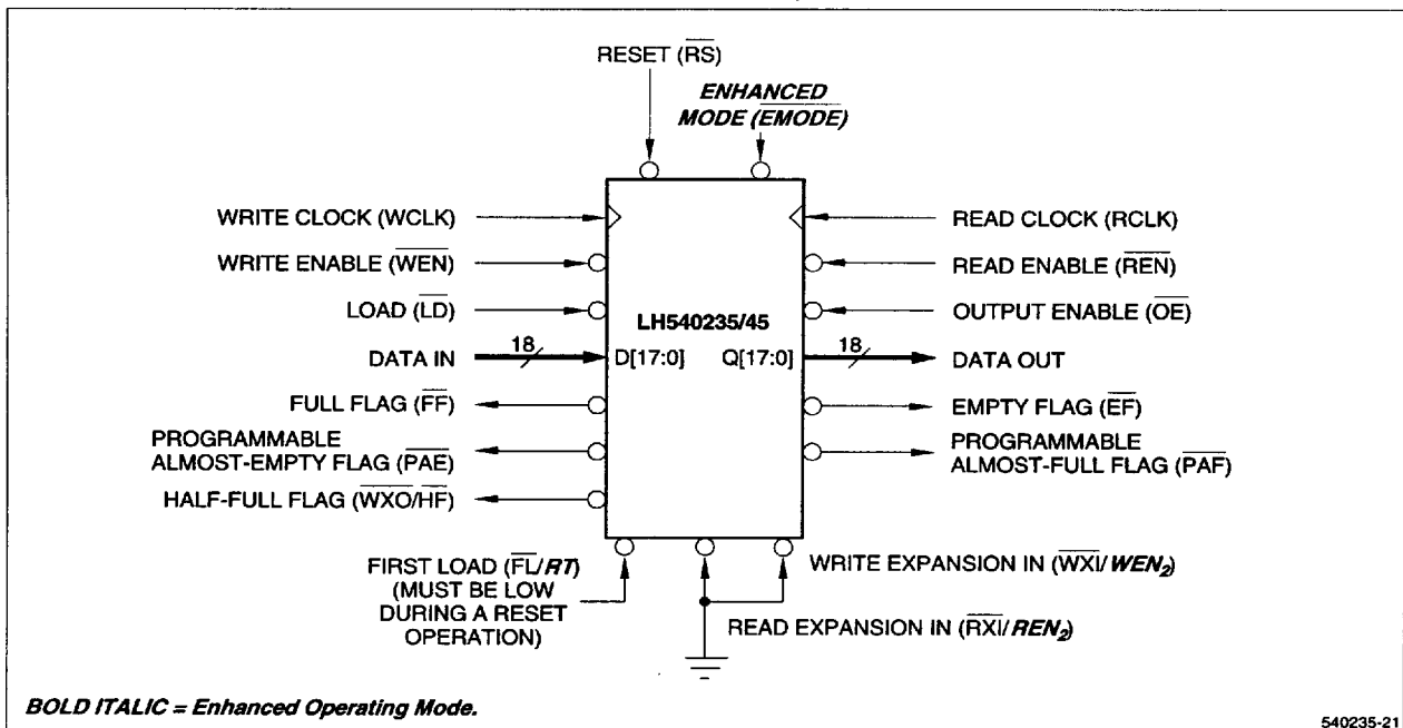
Figure 26. Standalone FIFO (2048 x 18 / 4096 x 18)
