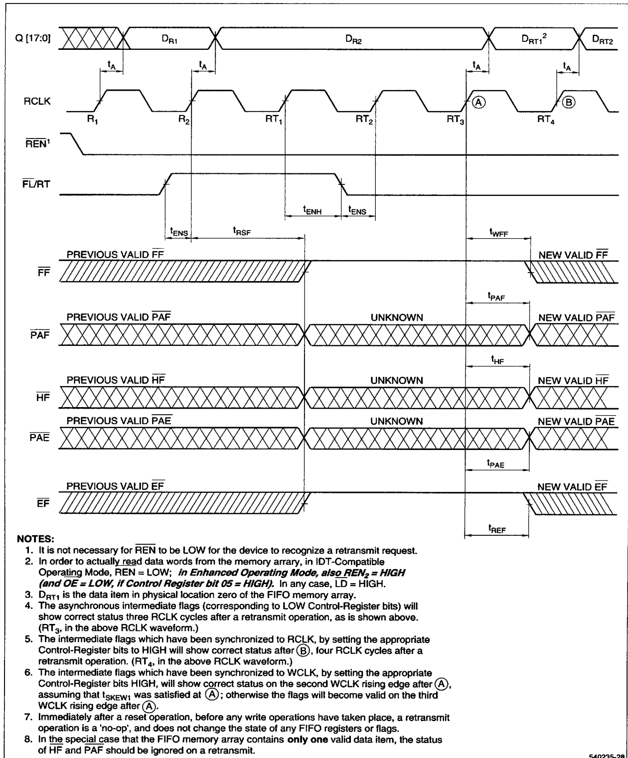
Figure 21. Retransmit Timing, IDT-Compatible Operating Mode
