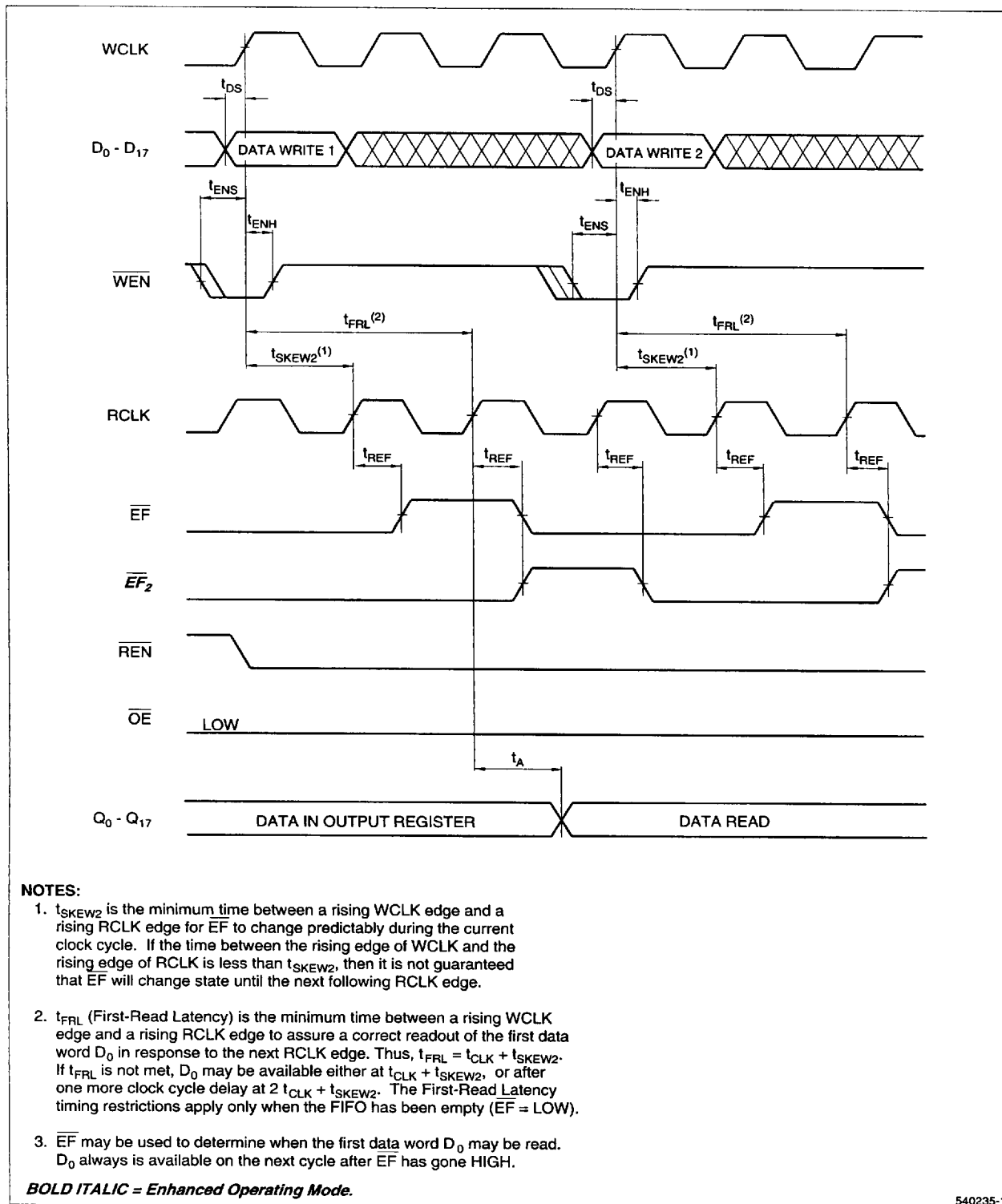
Figure 11. Empty-Flag Timing
