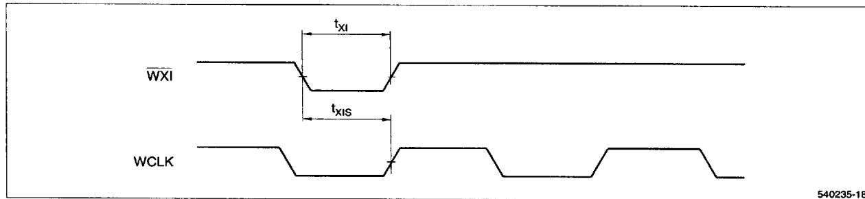
Figure 24. Write-Expansion-In Timing,
