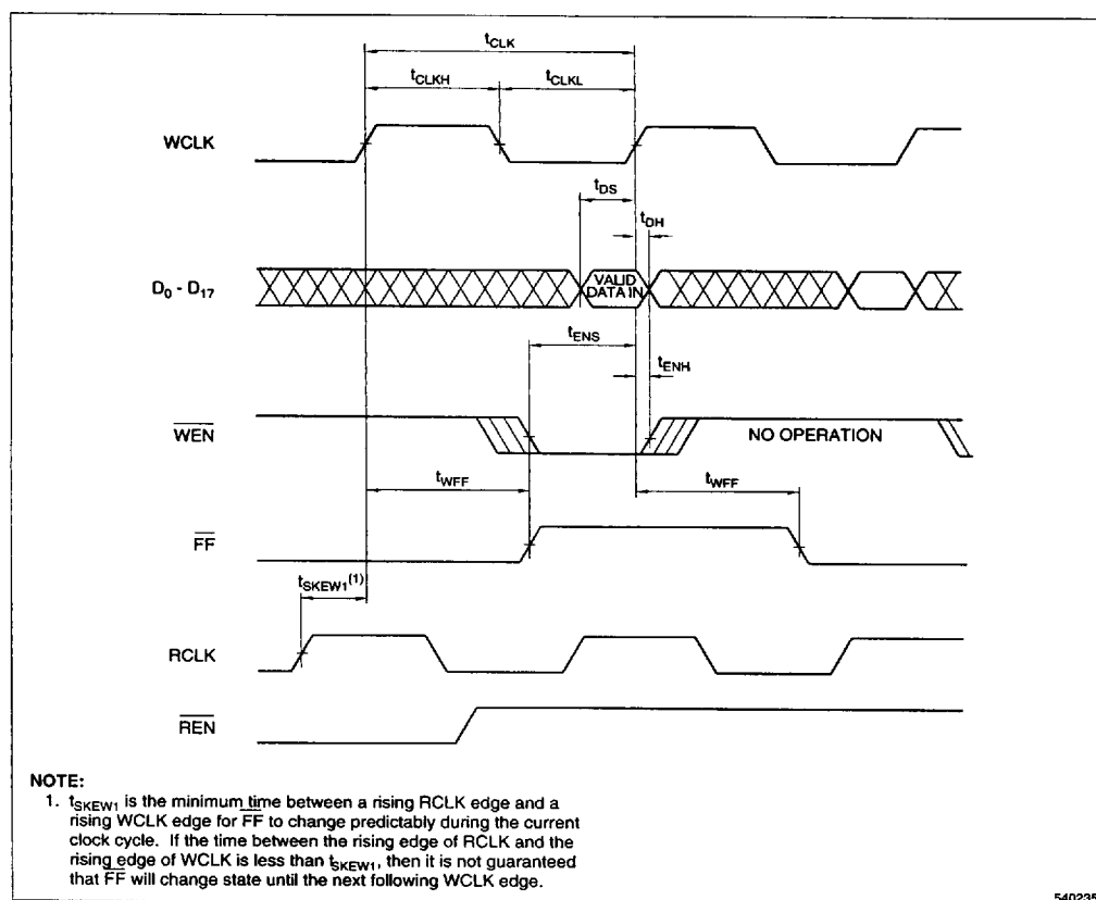
Figure 7. Synchronous Write Operation
