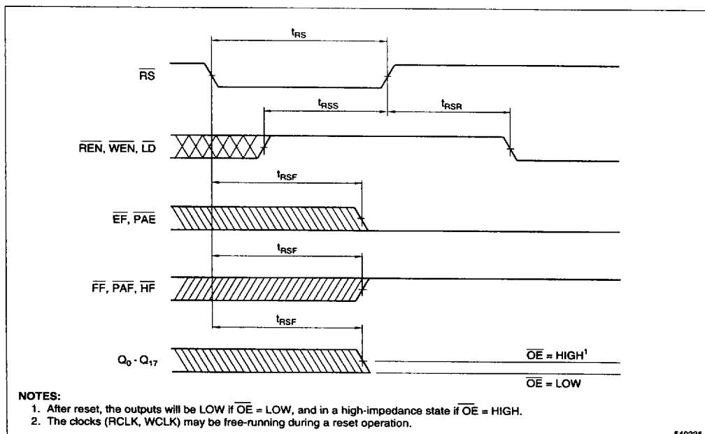
Figure 6. Reset Timing
