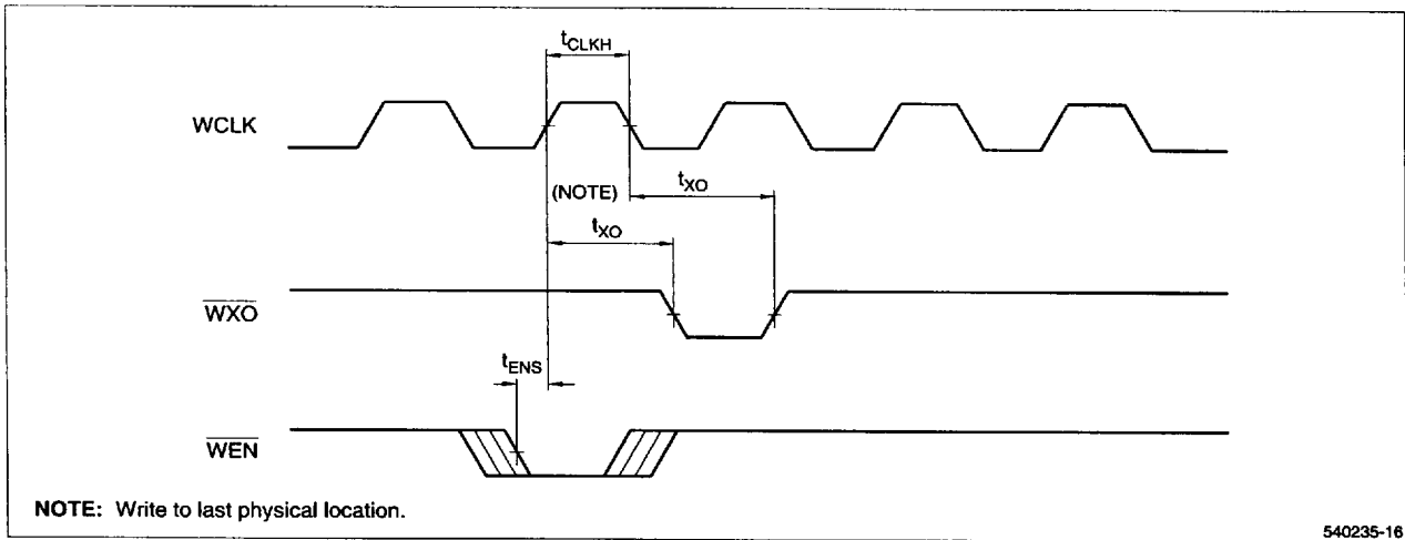
Figure 22. Write-Expansion-Out Timing, IDT-Compatible Operating Mode
