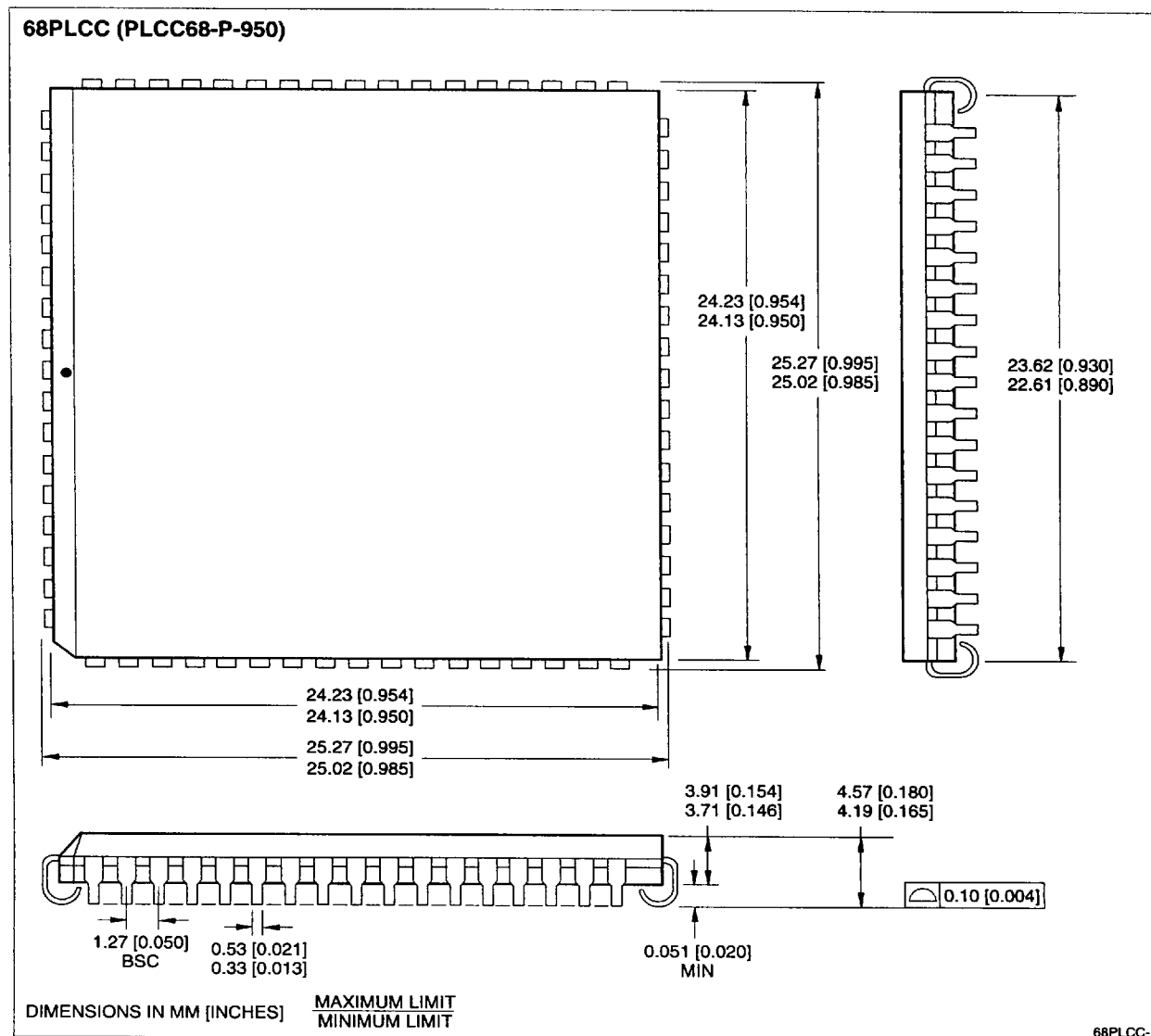
68-Pin PLCC
