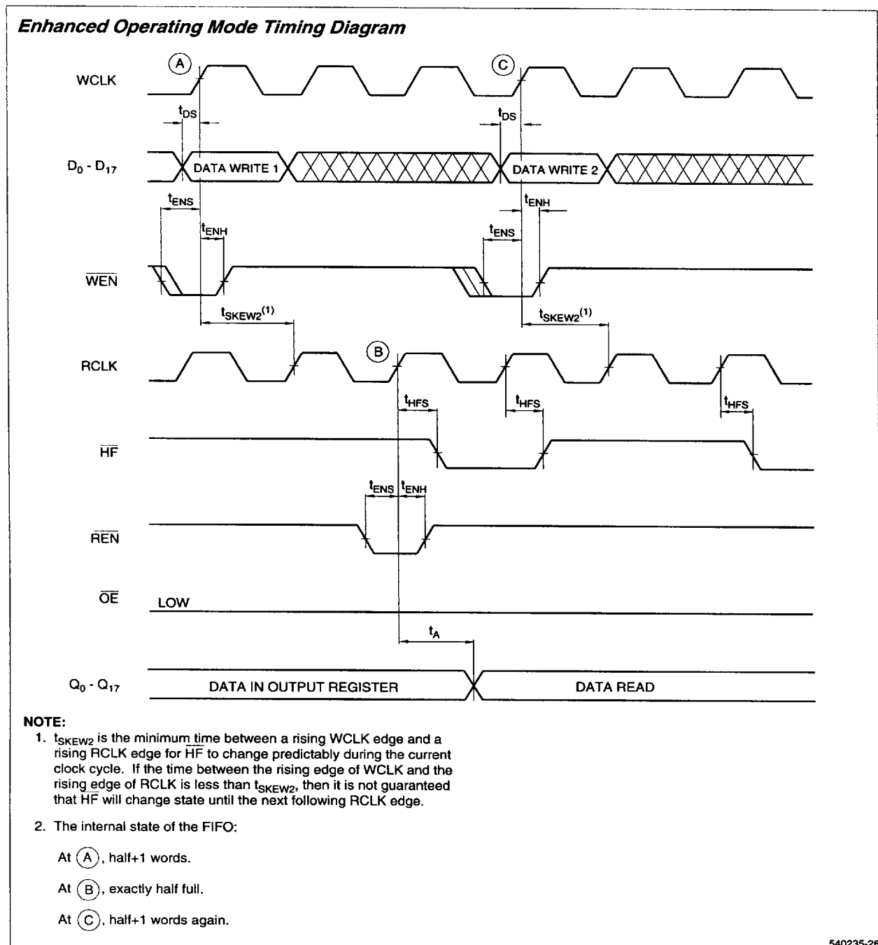
Figure 20. Half-Full-Flag Timing, When Synchronized to Output Port (Enhanced Operating Mode)
