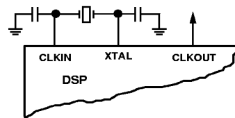
Figure 3. External Crystal Connections
