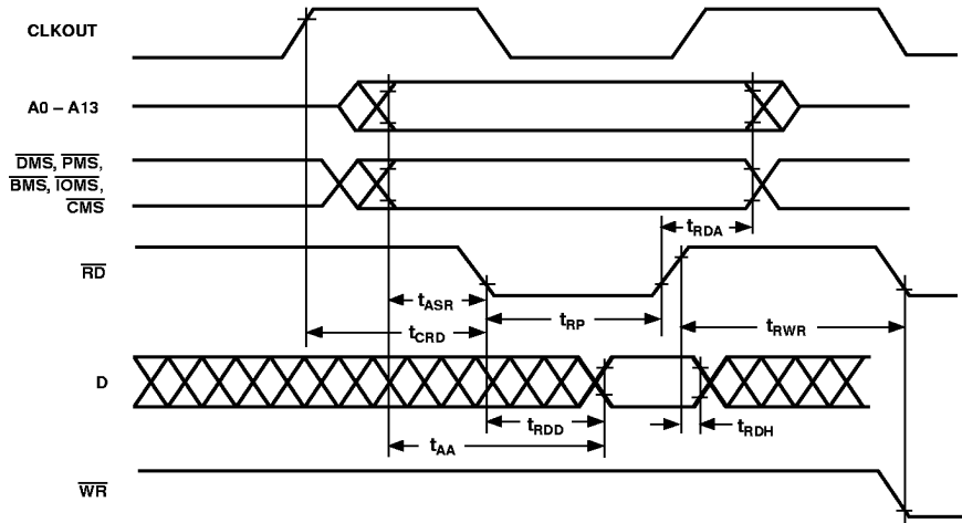
Figure 18. Memory Read
