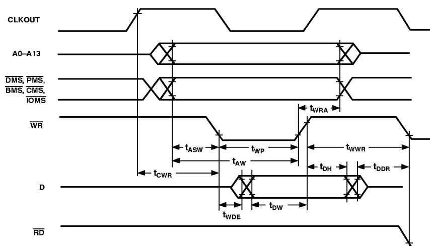
Figure 19. Memory Write
