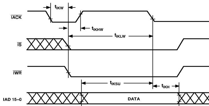
Figure 23. IDMA Write, Short Write Cycle
