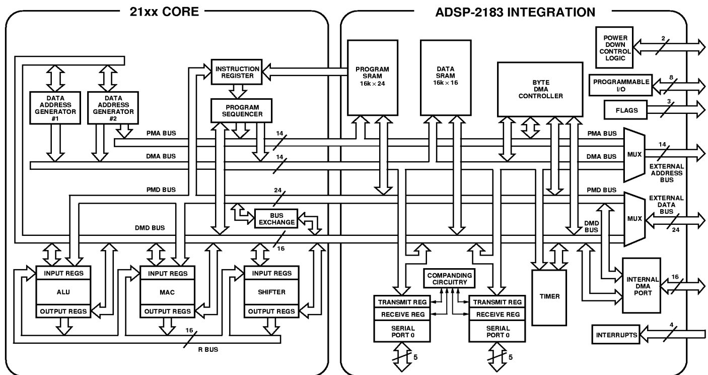
Figure 1. Block Diagram
