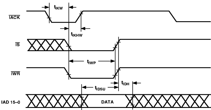
Figure 22. IDMA Write, Short Write Cycle
