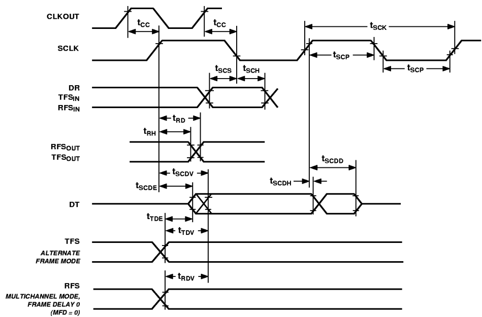
Figure 20. Serial Ports
