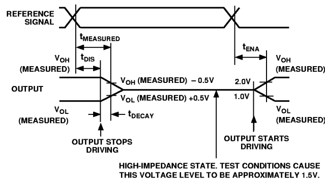
Figure 13. Output Enable/Disable
