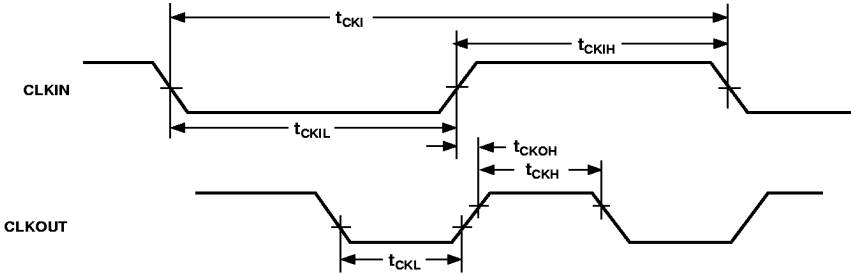
Figure 15. Clock Signals
