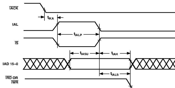
Figure 21. IDMA Address Latch
