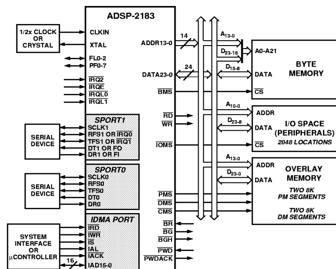
Figure 2. ADSP-2183 Basic System Configuration
