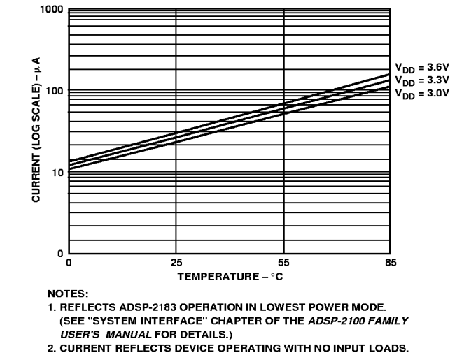
Figure 8. Power-Down Supply Current (Typical)
