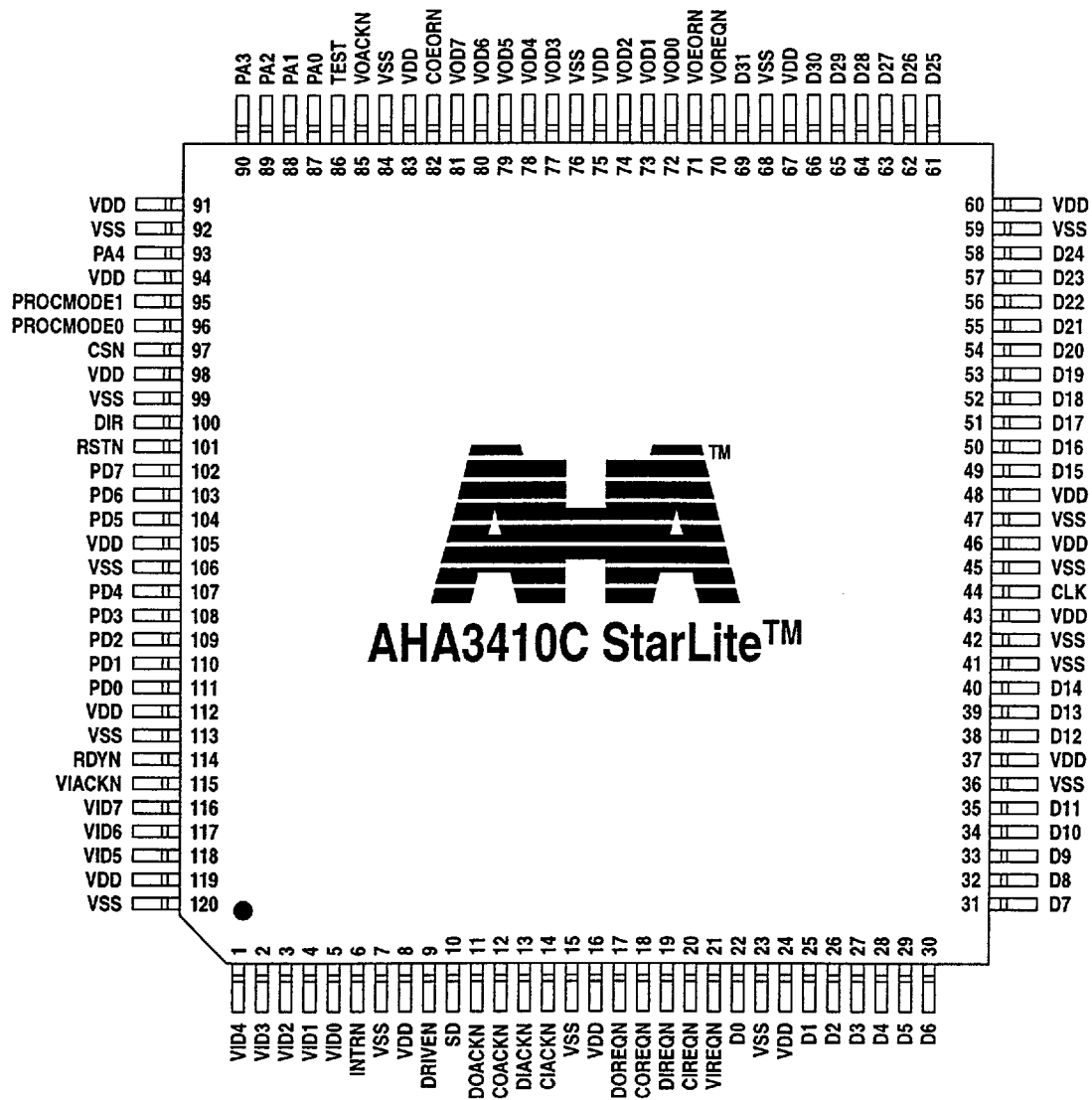
Figure 16: Pinout
