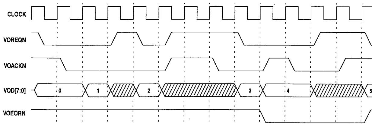
Figure 15: Timing Diagram, Video Output
