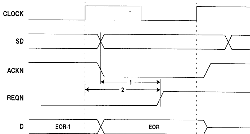
Figure 19: Request Deasserts at EOR, Strobe Condition of DSC=0-3, 6-15; ERC=0
