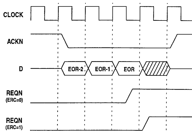
Figure 13: Request vs. End-of-Record, Strobe Condition of DSC=010
