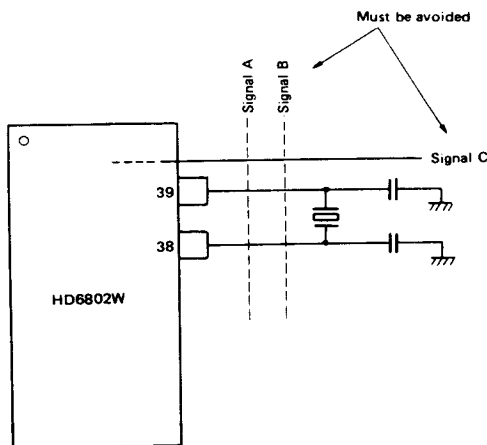
Figure 15 Note for Board Design of the Oscillation Circuit
