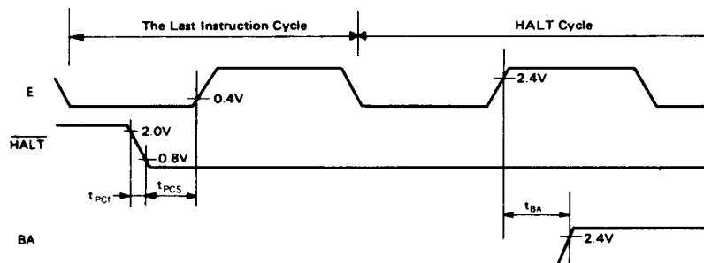
Figure 6 Timing of \overline{\text{HALT}} and BA
