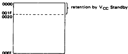
Figure 2 Address Map of HD6802W
