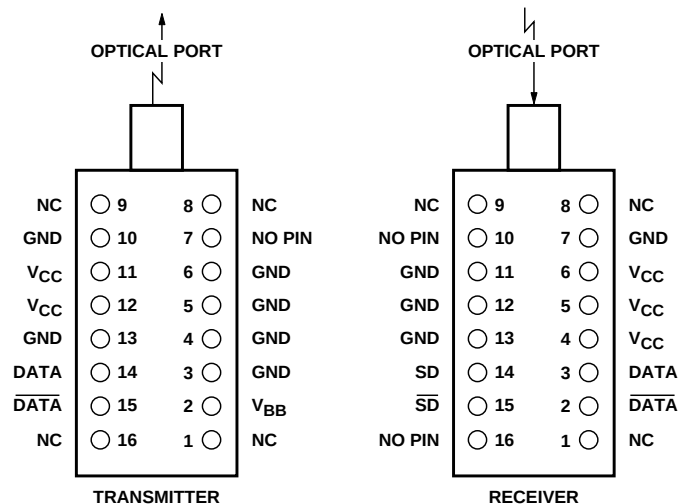
Figure 3. Pinout Drawing.
