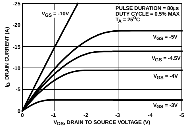
FIGURE 7. SATURATION CHARACTERISTICS
