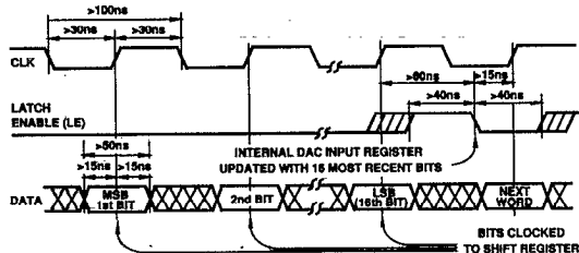
Figure 8. Timing Relationships of Input Signals
