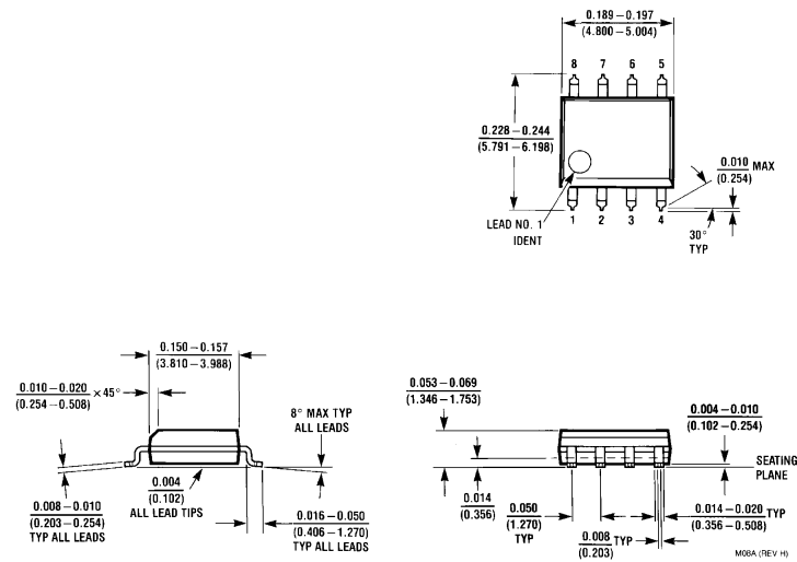
8-Pin Small Outline Package Order Number LMC7211AIM or LMC7211BIM NS Package Number M08A
