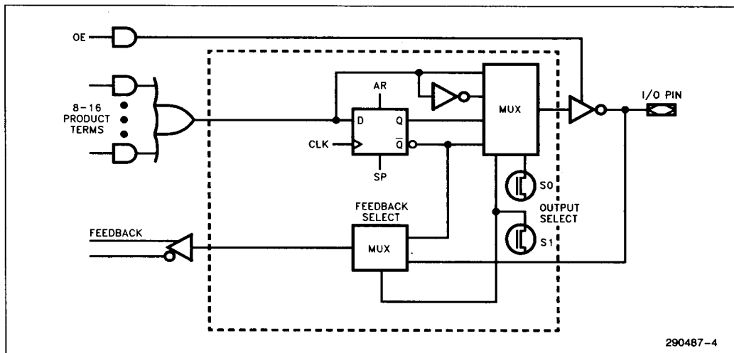
Figure 3. IPLDLV22V10 Macrocell Architecture
