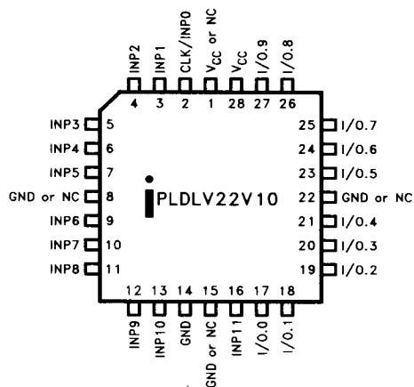
Figure 1. Pinout Diagrams
