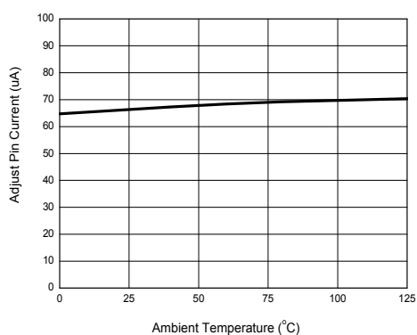
Figure 9. Adjust Pin Current vs. Temperature
