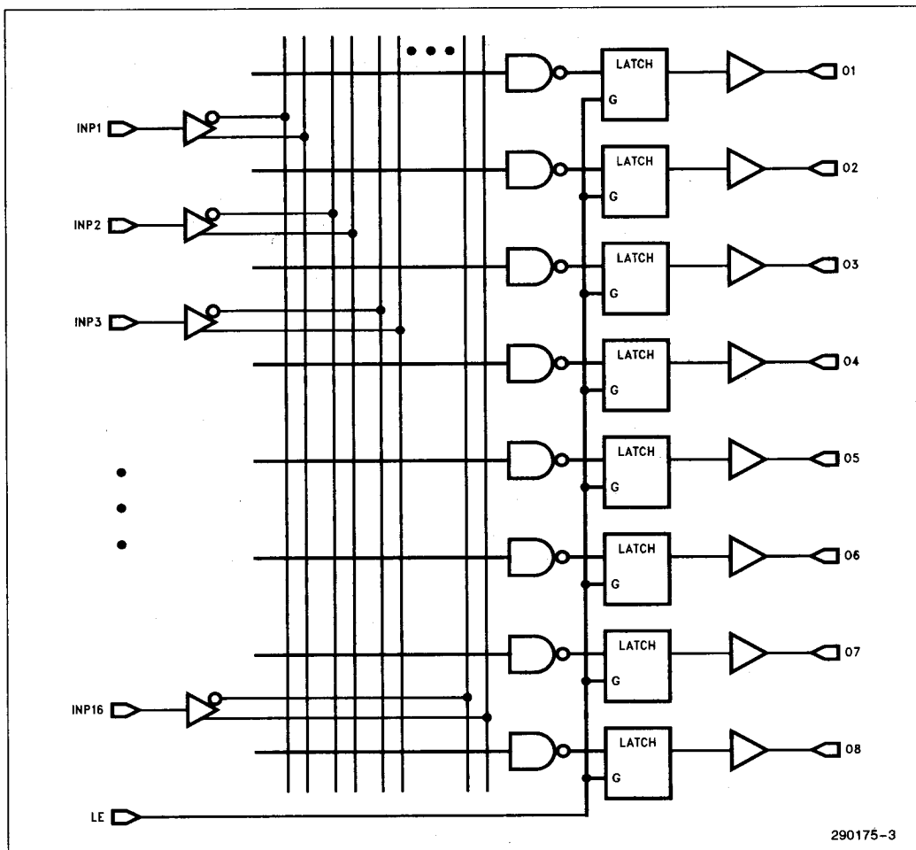
Figure 2. 85C508 Global Architecture
