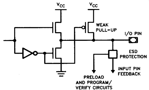
Input/Output Equivalent Schematics
