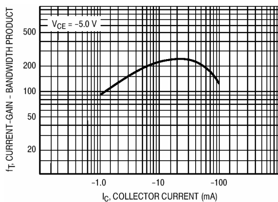
Fig 6. Bandwidth Product
