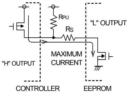
Fig.47 I/O Circuit
