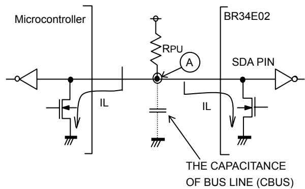
Fig.43 I/O Circuit
