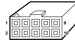
10 POSITION IDC CONNECTOR CENTER POLARIZED.
