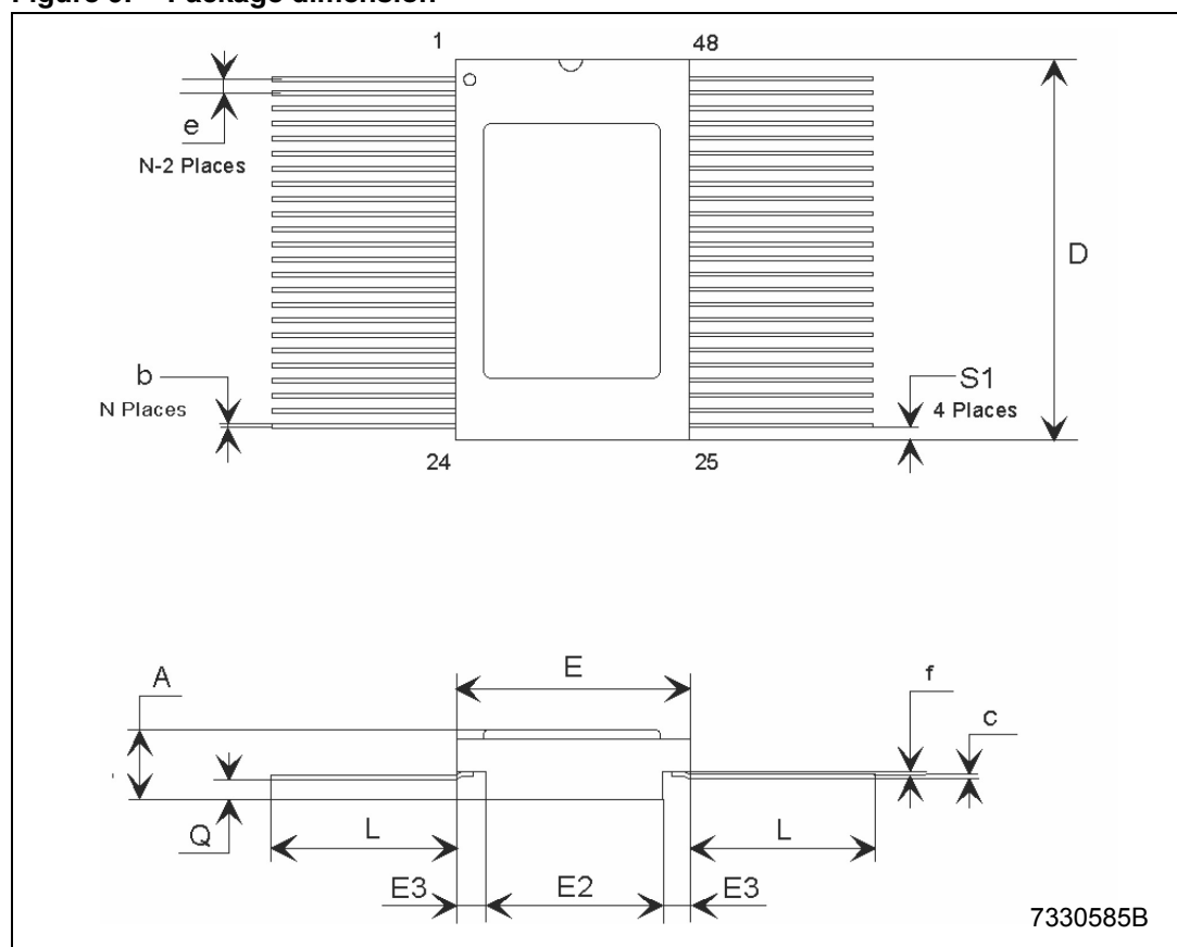
Figure 9. Package dimension
