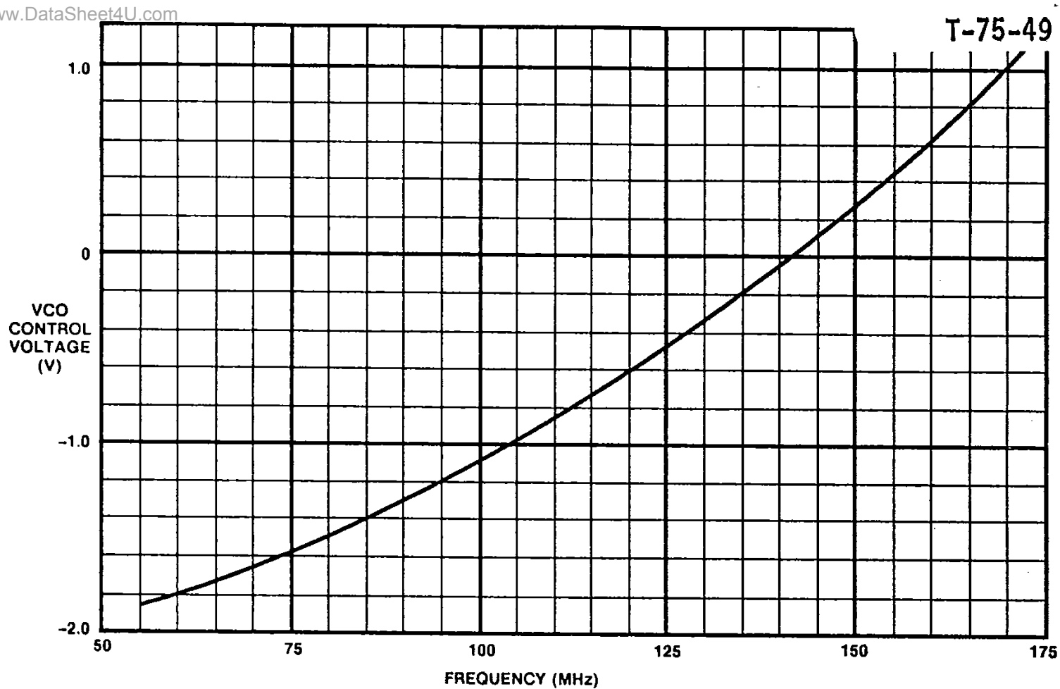
Fig.5 Receiver VCO characteristic (typical)
