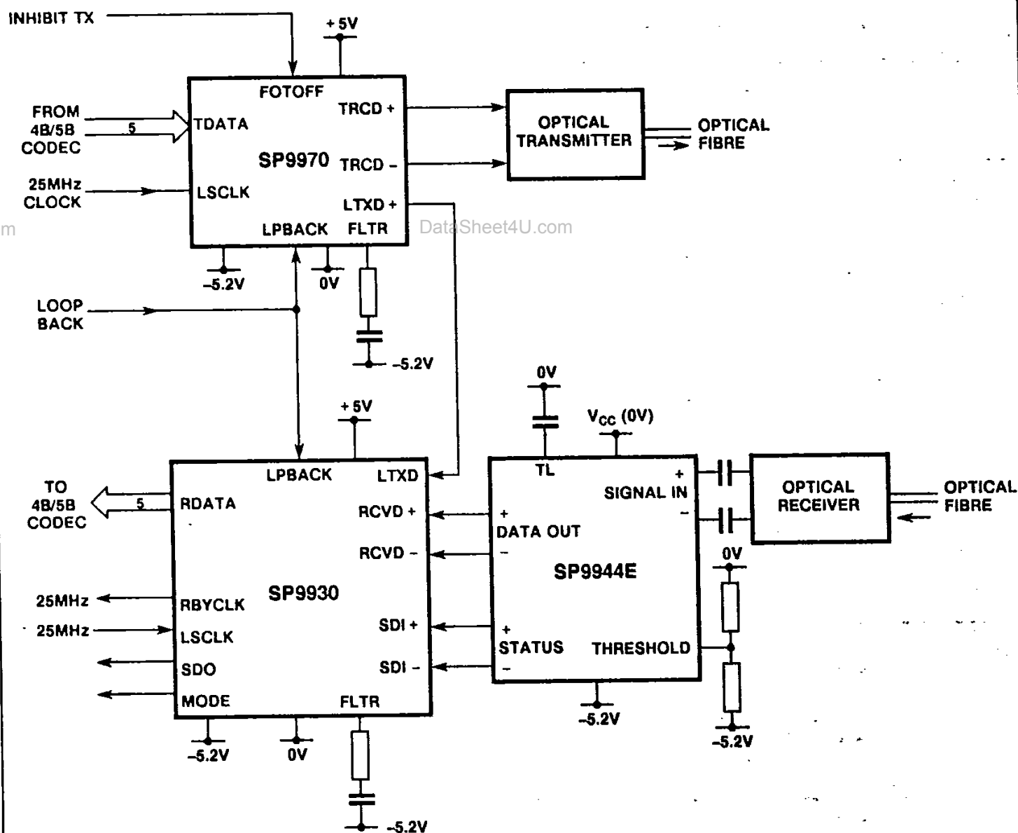
Fig.8 Typical FDDI application circuit
