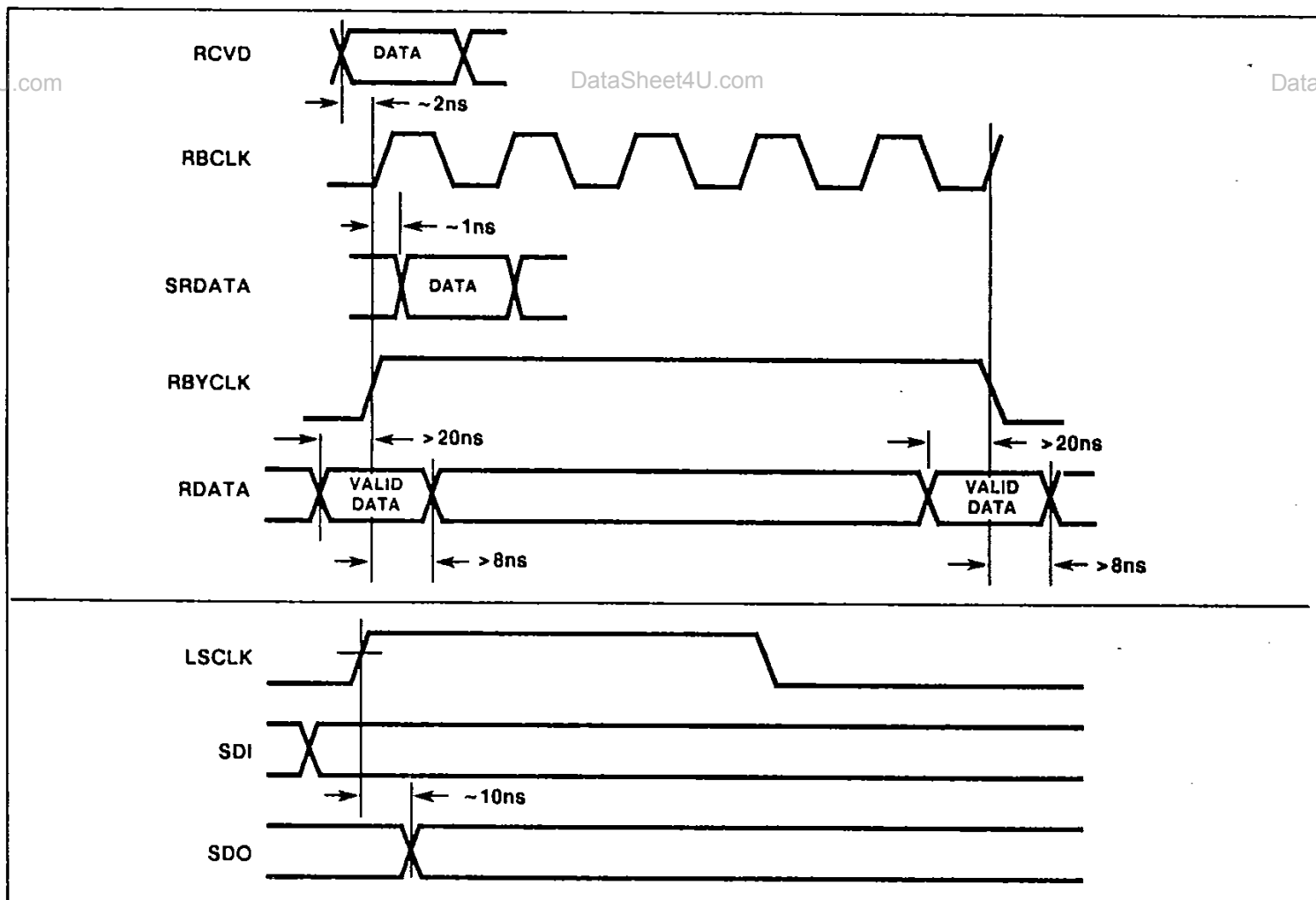
Fig.6 Receiver timing diagram
