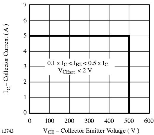
Figure 3. V_{\text{CEW}} - Diagram
