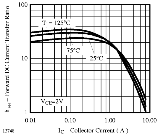
Figure 8. h_{\text{FE}} vs. I_{\text{C}}
