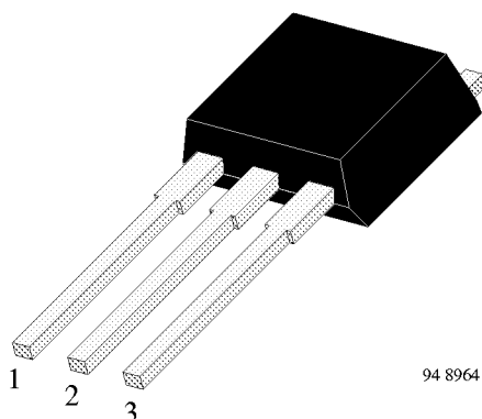
BUD725D 1 Base 2 Collector 3 Emitter
