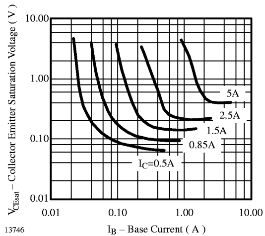
Figure 7. V_{\text{CEsat}} vs. I_{\text{B}}
