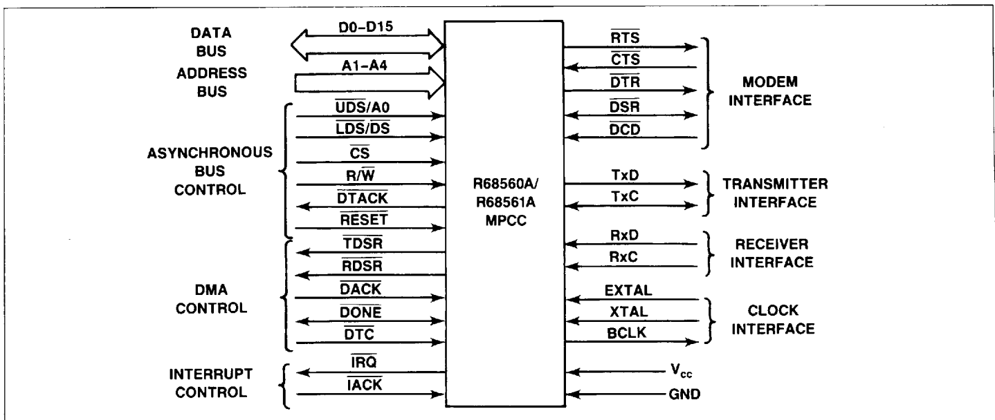
Figure 2. MPCC Input and Output Signals
