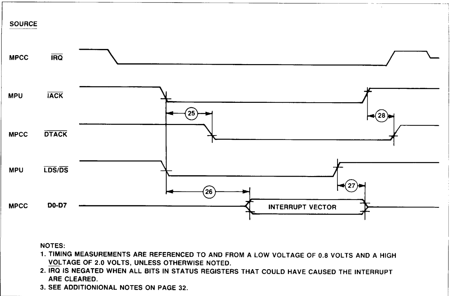
Figure 16. Interrupt Request Cycle Timing
