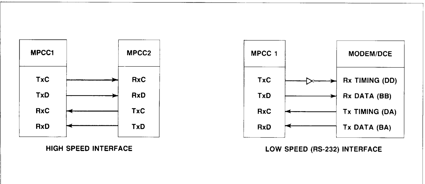
Figure 17. Serial Interface
