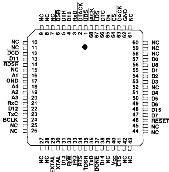
R68561AJ-68-Pin PLCE
