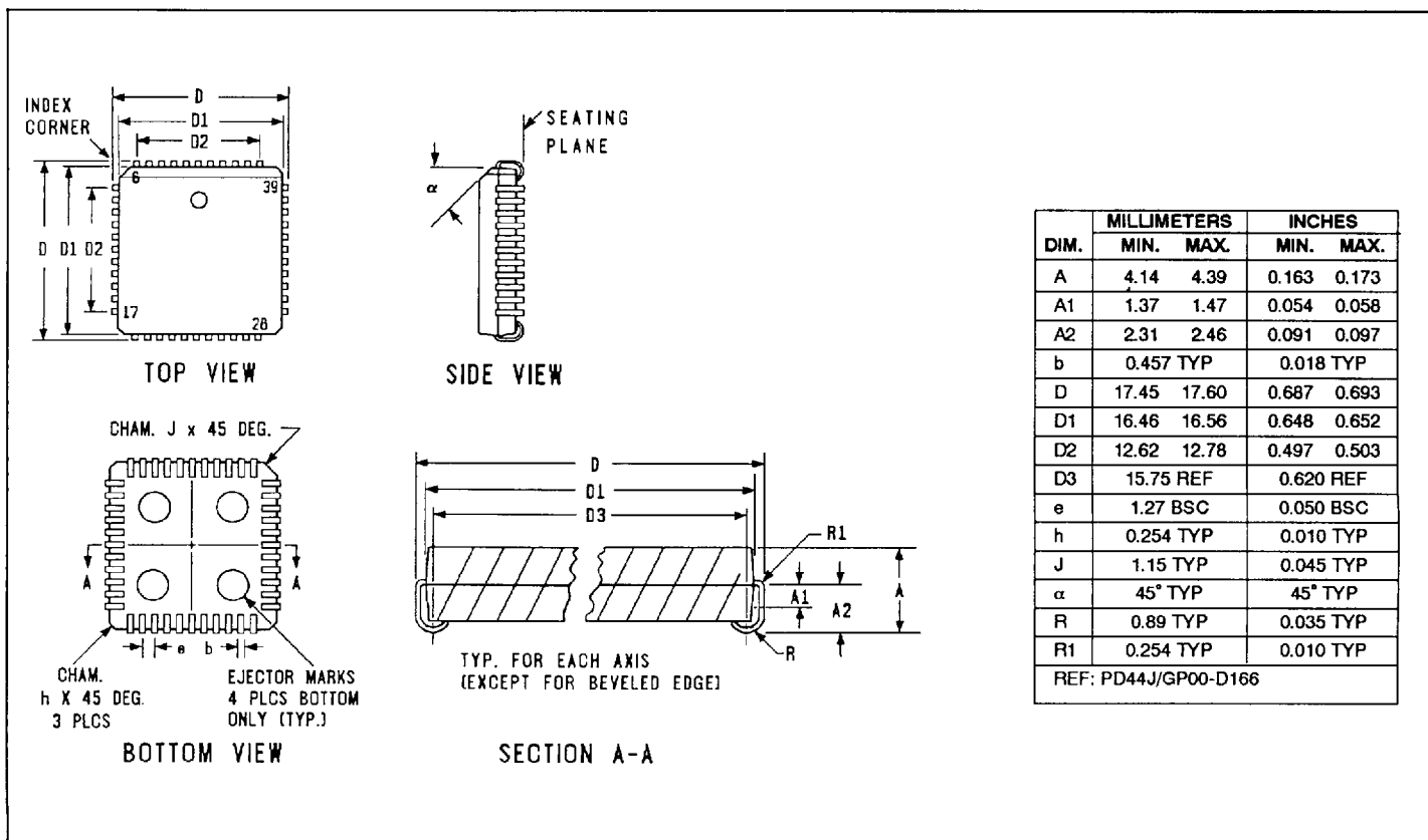
44-Pin PLCC
