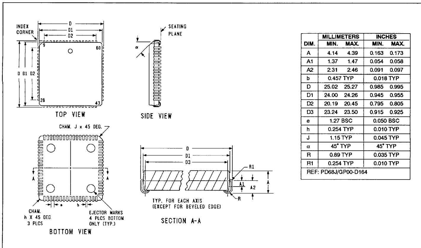
68-Pin PLCC
