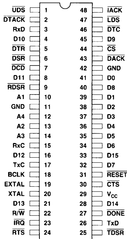
R68561AP, AC-48-Pin DIP
