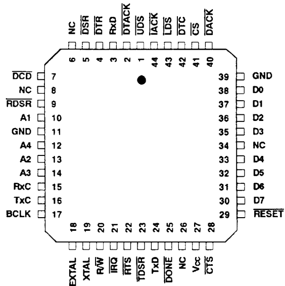
R68560AJ-44-Pin PLCE
