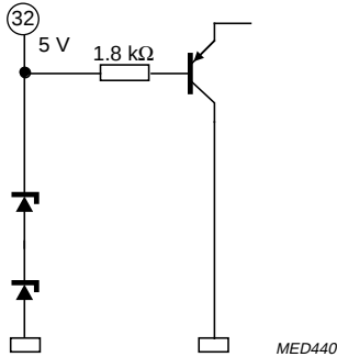
Fig.31 Pin 32: SCL (I 2 C-bus clock).
