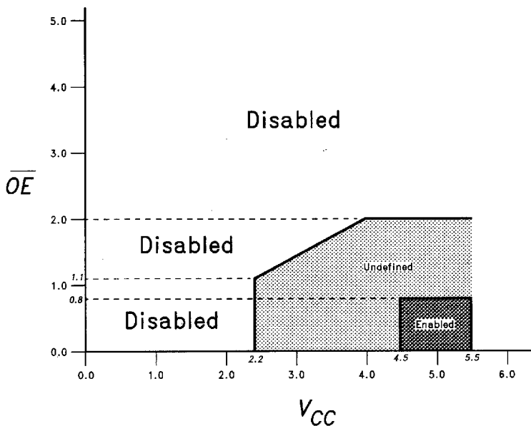
V_{CC} and \overline{OE} Power-up Relationship
