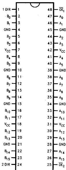
Pin Assignment for SSOP and Flatpak
