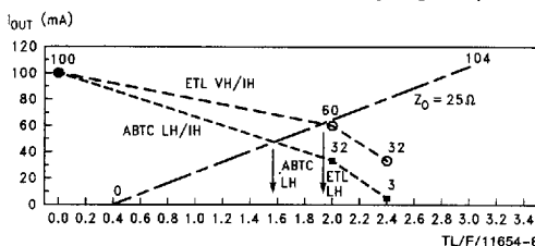
Estimated ETL/ABTC Initial Rising Edge Step
