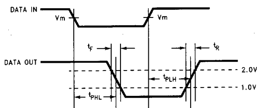
FIGURE 4. Rise, Fall Time and Propagation Delay Waveforms
