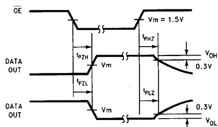
FIGURE 3. TRI-STATE Output HIGH and LOW Enable and Disable Times
