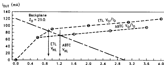
Estimated ETL/ABTC Initial Falling Edge Step
