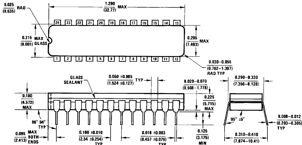
24 Lead Slim (0.300" Wide) Ceramic Dual-In-Line (SD) NS Package Number J24F
