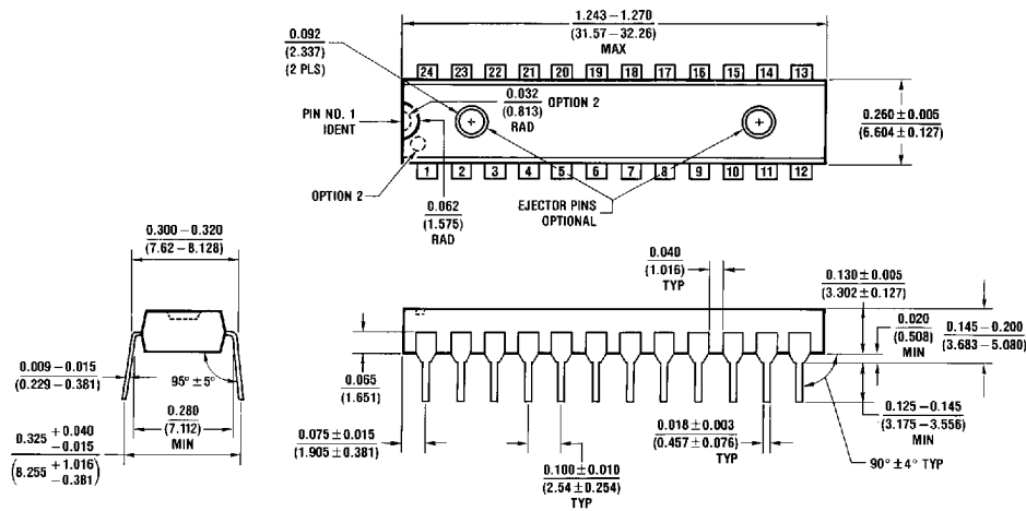
24 Lead Slim (0.300" Wide) Plastic Dual-In-Line (SP) NS Package Number N24C
