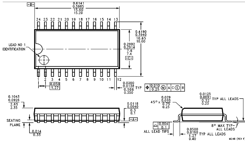
24 Lead Small Outline Integrated Circuit (S) NS Package Number M24B
