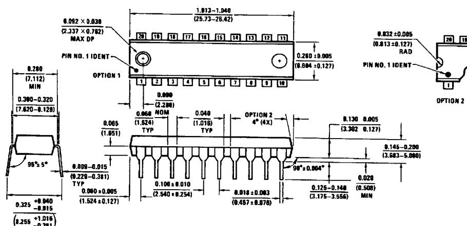
Molded Dual-In-Line Package (N) Order Number DM64ALS574AN or DM74ALS574AN NS Package Number N20A
