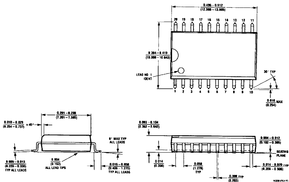
S.O. Package (M) Order Number DM64ALS574AWM or DM74ALS574AWM NS Package Number M20B
