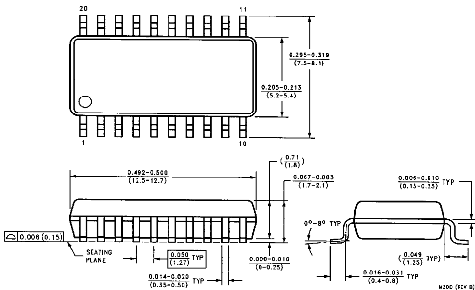
Small Outline Package (SJ) Order Number DM64ALS574ASJ or DM74ALS574ASJ NS Package Number M20D
