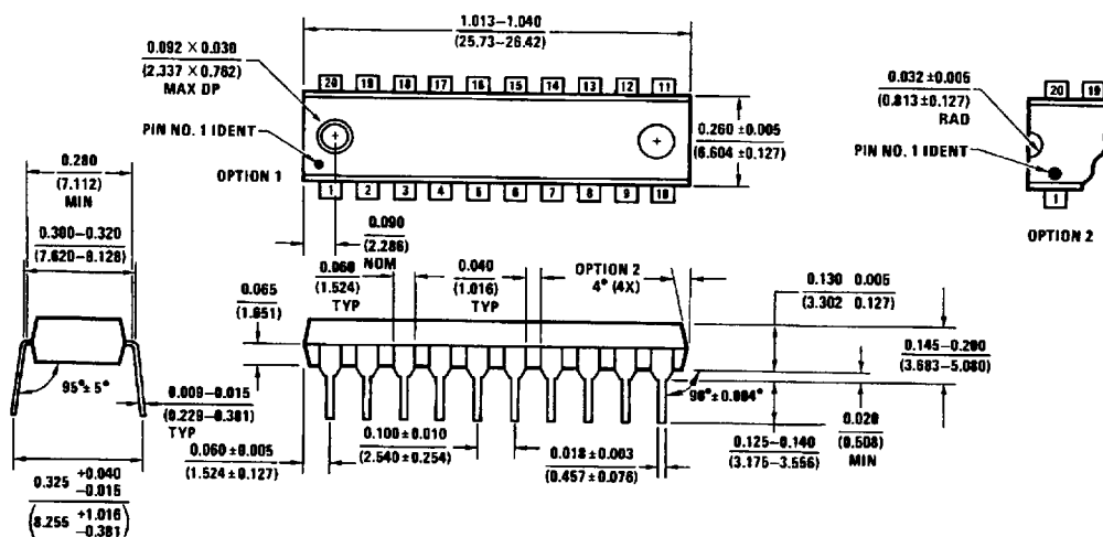
Molded Dual-In-Line Package (N) Order Number DM74ALS576AN NS Package Number N20A
