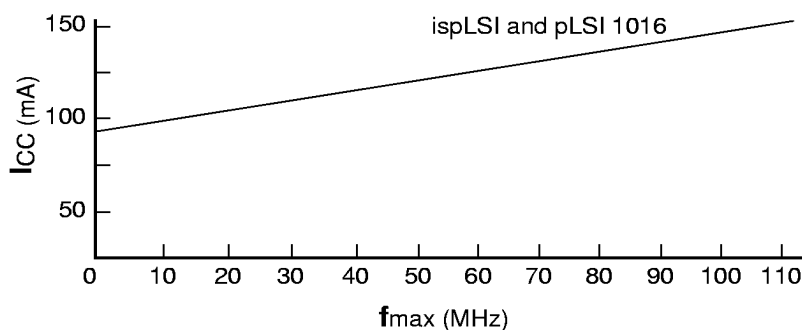
Figure 3. Typical Device Power Consumption vs fmax
