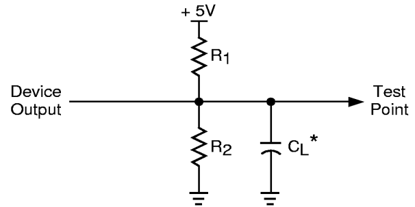
Figure 2. Test Load
