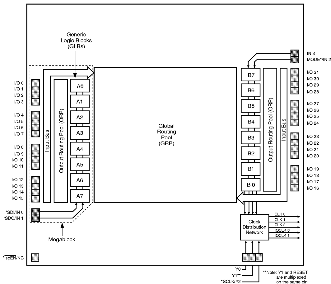
Figure 1. ispLSI and pLSI 1016 Functional Block Diagram
