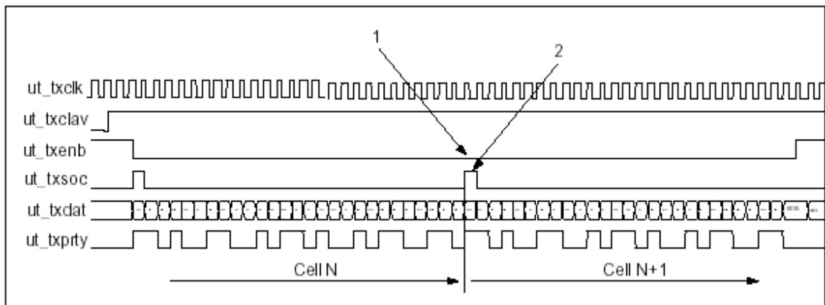
Figure 9: Back to Back Cells Transfer
