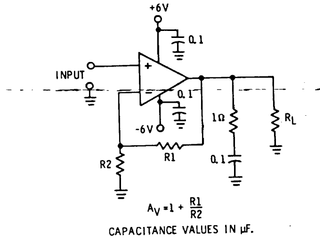
NON-INVERTING POWER AMPLIFIER
