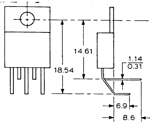
DESIGNATOR ZH PACKAGE Z (Except as Shown)
