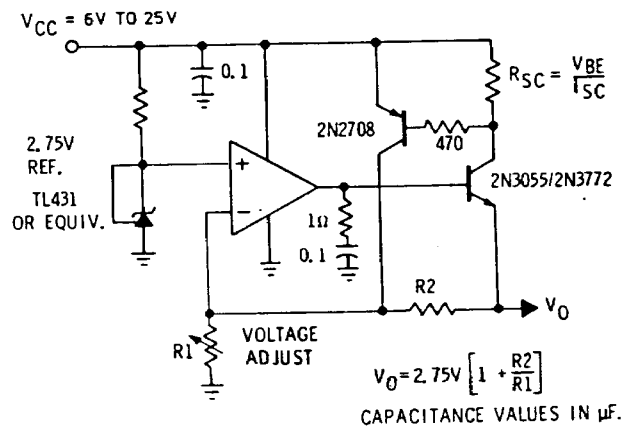
HIGH-POWER LINEAR REGULATOR (Short-Circuit Protected)
