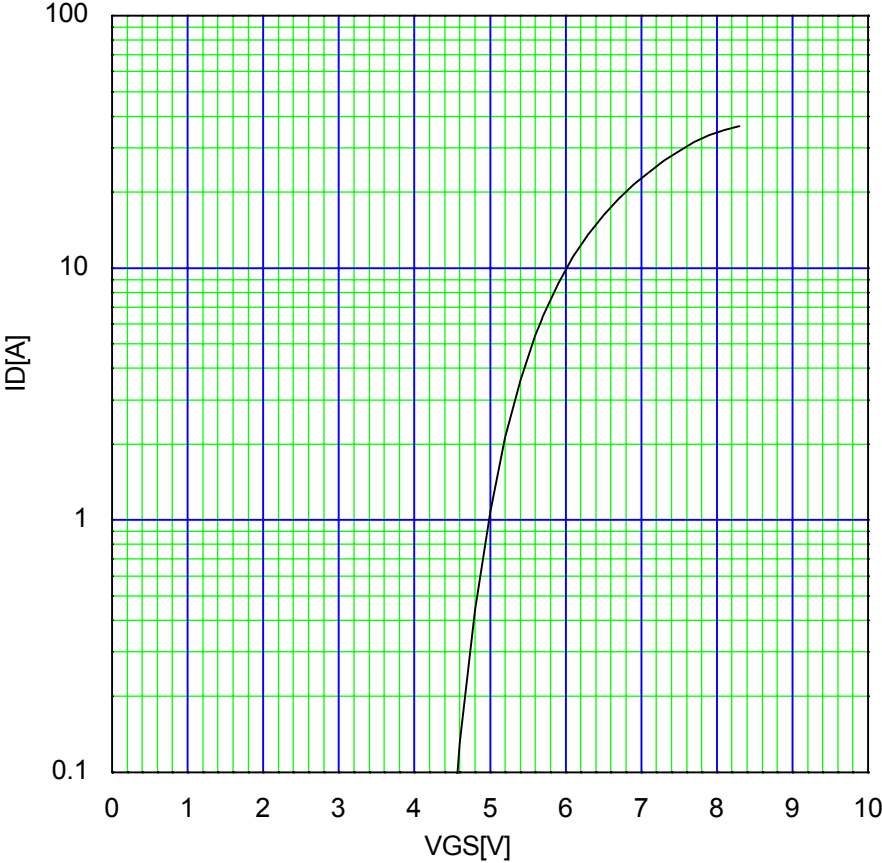
Typical Transfer Characteristic ID=f(VGS):80\text{ }\mu\text{s pulse test, }VDS=25\text{V, }Tch=25^{\circ}\text{C}
