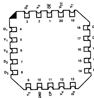
Leadless Chip Carrier L-20-1
