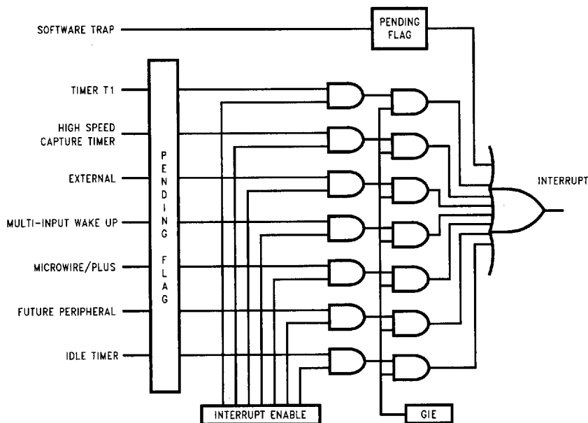
FIGURE 12. Interrupt Block Diagram
