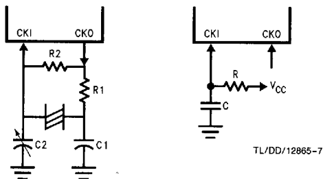
FIGURE 5. Crystal and R/C Oscillator Diagrams
