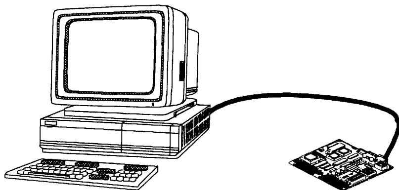
FIGURE 16. COP-DM Environment
