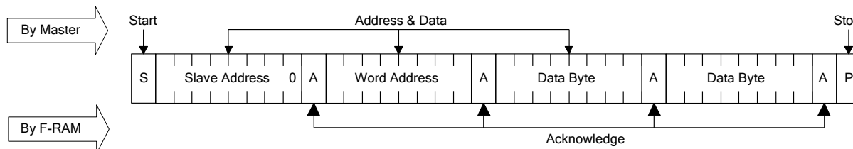
Figure 6. Multiple-Byte Write
