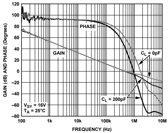
Figure 21. Open-Loop Gain and Phase Shift vs. Frequency
