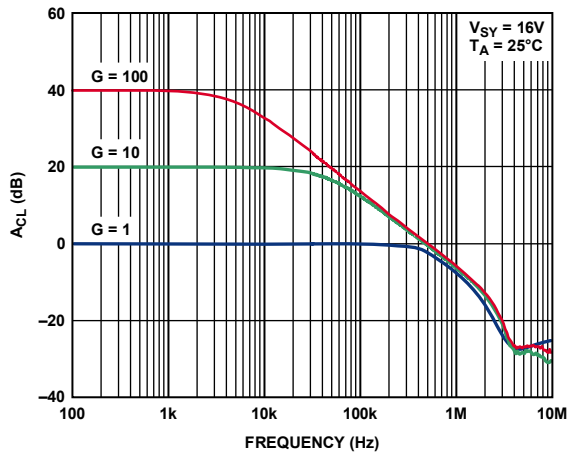
Figure 22. Closed-Loop Gain vs. Frequency, V_{SY} = 16V
