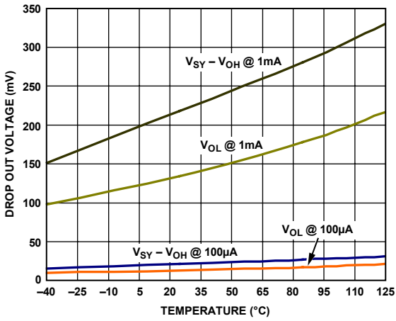
Figure 17. Output Voltage Saturation vs. Temperature
