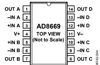
Figure 4. 14-Lead SOIC (R-14)
