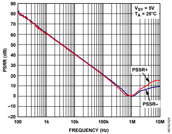
Figure 24. PSRR vs. Frequency, V_{SY} = 5\text{ V}
