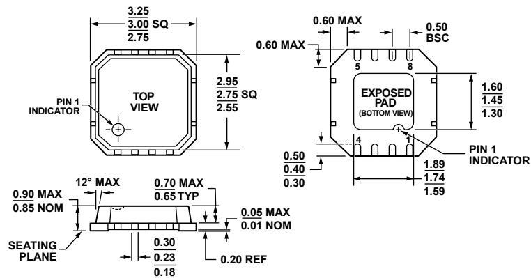
Figure 44. 8-Lead Lead Frame Chip Scale Package [LFCSF_VD] 3 mm x 3 mm Body, Very Thin, Dual Lead (CP-8-2)
