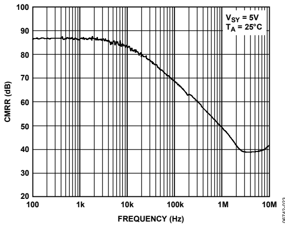
Figure 12. CMRR vs. Frequency, V_{SY} = 5V
