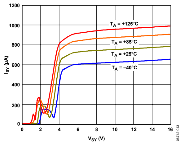
Figure 34. Supply Current vs. Supply Voltage AD8669
