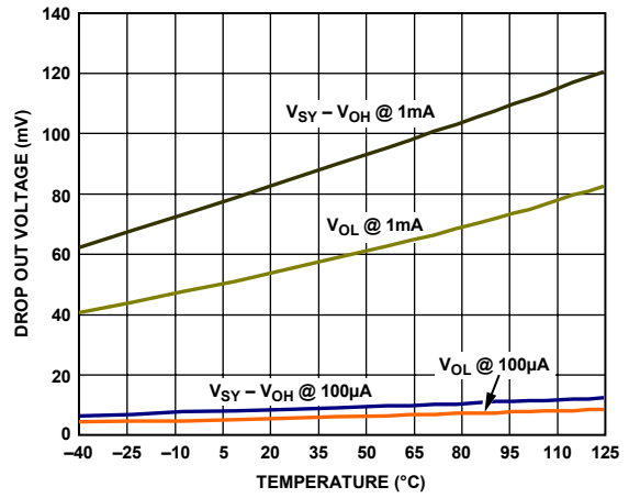
Figure 20. Output Voltage Saturation vs. Temperature
