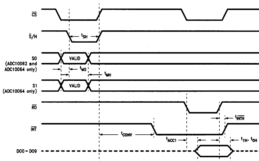
FIGURE 1. Mode 1 ( t_{RD} > t_1 ). The conversion time ( t_{CONV} ) is set by the internal timer.
