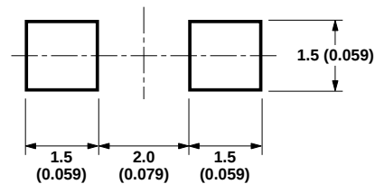
Figure 11. Recommended soldering pattern for HSMx-C152.
