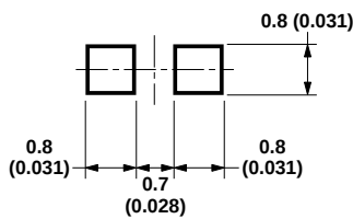
Figure 10. Recommended soldering pattern for HSMx-C192 and HSMx-C196.
