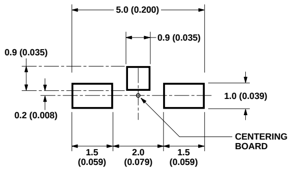
Figure 8. Recommended soldering pattern for HSMx-C112.
