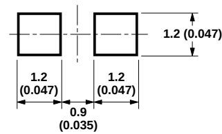
Figure 9. Recommended soldering pattern for HSMx-C172.
