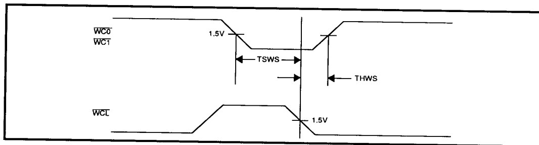
FIGURE 5: Control Timing
