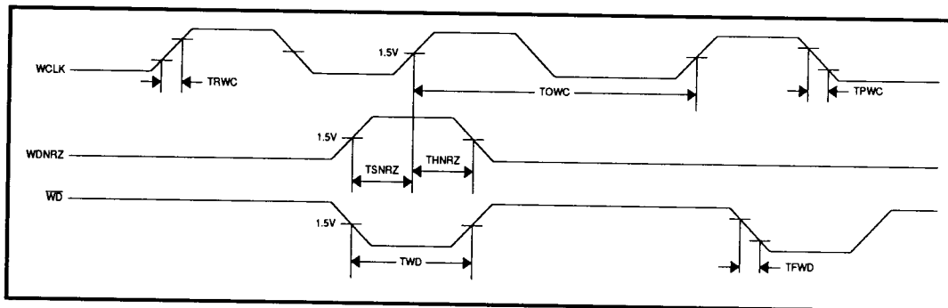
FIGURE 4: Write Timing
