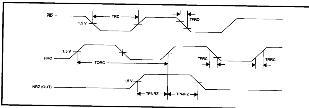
FIGURE 3: Read Timing
