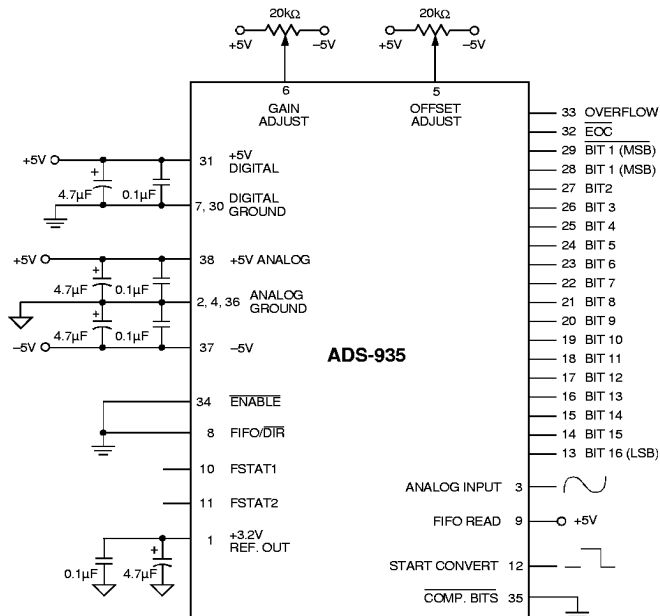
Figure 2. Connection Diagram
