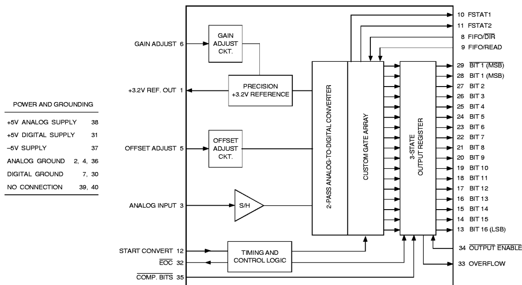
Figure 1. ADS-935 Functional Block Diagram
